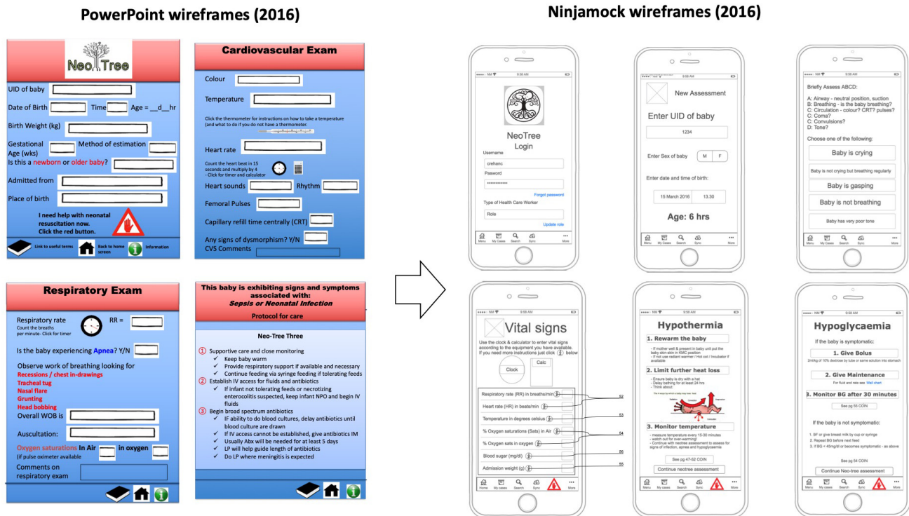
Figure 2. Prototype wireframes.
