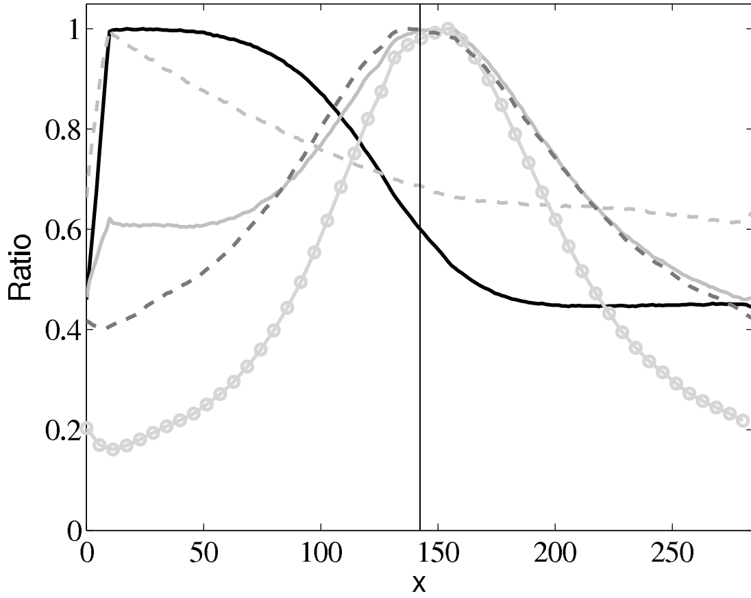
Figure 5.14: The change in x of various flux/stress quantities along the centre line in the converging-diverging channel. The configurational pressure \sigma_{CV}/\sigma_{0CV} (—), the left hand side of Eq. (5.34) normalised to one (—), broken down into kinetic pressure \kappa_{CV}/\kappa_{0CV} (---) and the convective term \rho \mathbf{u} \mathbf{u} / \rho_0 \mathbf{u}_0 \mathbf{u}_0 (-o-). The mass flux ratio (---) obtained from flow of molecules (Eq. (4.60) Advection) is also plotted which, on average, matches \rho u / \rho_0 u_0 in figure D.8. Subscript 0 denotes channel maximum, \sigma_{0CV} = 4.6 , \kappa_{0CV} = 1.3 and \rho_0 \mathbf{u}_0 \mathbf{u}_0 = 1.8 .
