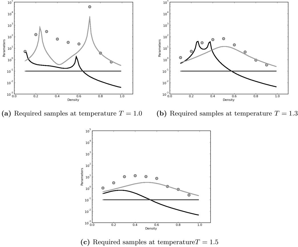
Figure E.1: Estimate of the required samples for a 5% error from Eq. 2.86 shown by M_\rho (—), M_u (—) and M_P (—) with MD estimates for M_P (•) calculated from equation E.1
