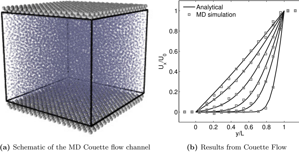
Figure 3.14: The y -dependence of the streaming velocity profile at times t = 2^n for n = 0, 2, 3, 4, 5, 6 from right to left. The squares are the NEMD CV data values and the analytical solution Eq. (3.10) are the black lines.
