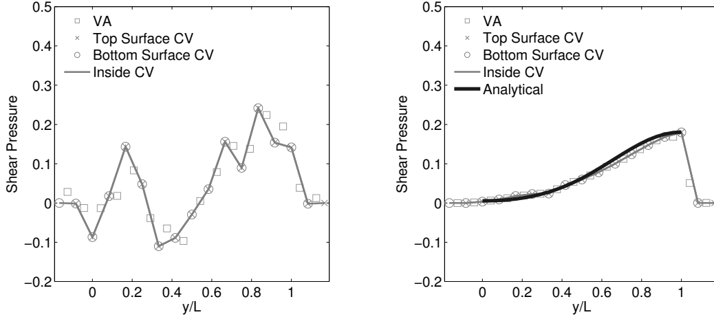
(a) The y -dependence of the shear pressure at t = 10 , averaged over 100 timesteps and for a single simulation trajectory. The VA value from Eq. (4.32) are the squares. The CV surface traction from Eq. (4.34) is indicated by \times and \circ for the top and bottom surfaces, respectively. The solid gray line displays the resulting pressure field using Eq. (4.39) with linear shape functions.
