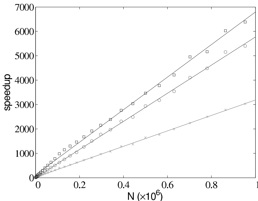
Figure 3.2: Relative speedup compared to an all pairs calculation ( t_{case}/t_{ap} ) – using the cell list (x), neighbour list (o) and neighbour list with half interaction (□) optimisations.
