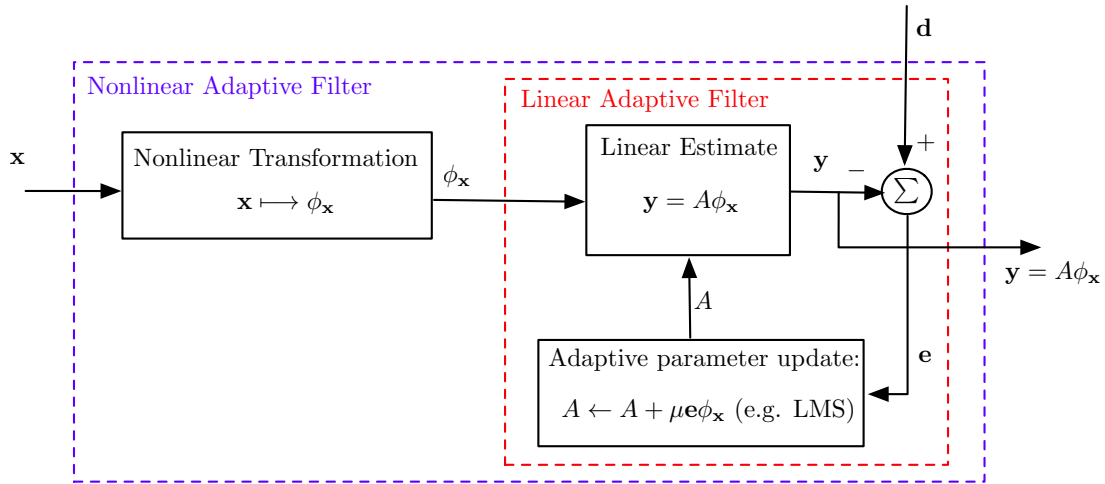
Figure 3.3: Diagram of an adaptive filter that is nonlinear in the input ( x ) and linear in the parameters ( A ). This filter is constructed by applying a nonlinear transformation on the input and then performing adaptive filtering using the transformed sample.
