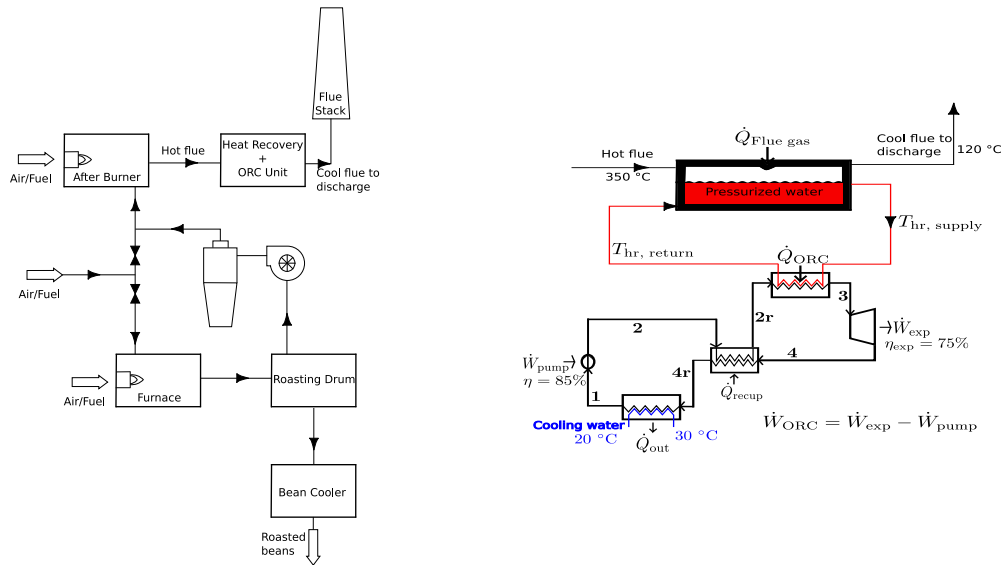
Fig. 3. Case Study 2: Waste heat recovery from flue gas via the organic Rankine cycle (ORC) system: LEFT – Schematic of coffee torrefaction process showing heat recovery and ORC power generating unit; RIGHT – Schematic of pressurized-water heat recovery unit and recuperative ORC engine.
