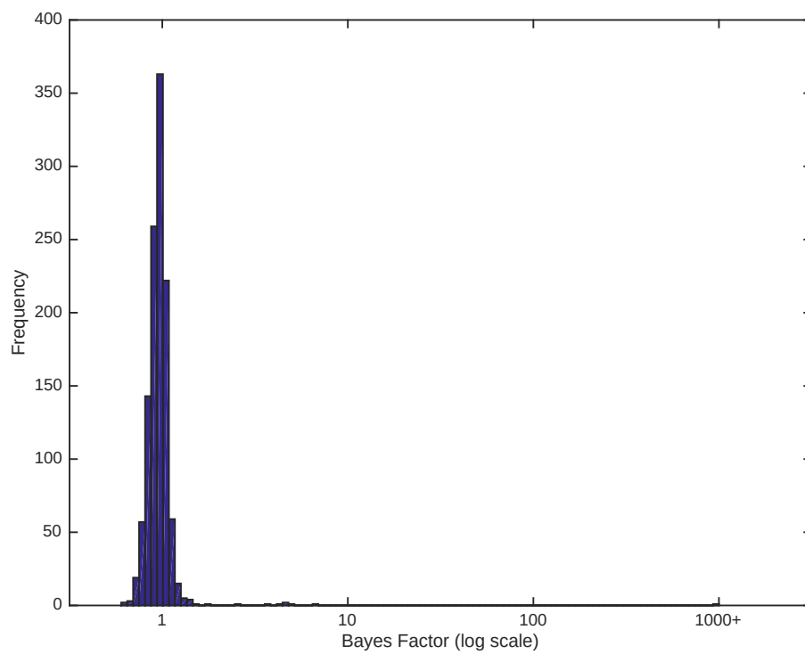
Figure S3: Bayes factor calculation for the HIV study.
