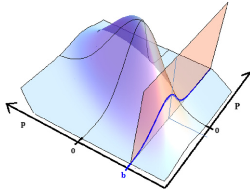
Figure 2. Joint probability distribution of the momenta of the particle and measurement device after weak measurement. The position p of the particles are weakly measured with devices sampled from a momentum distribution with mean zero and \Delta_P \neq 0 . Each particle's momentum is shifted by an amount proportional to the momentum of the device P , following (34). If one now postselects measurement devices based on the particle having momentum p = b , then the distribution of these devices is shown on the plane intersecting the plot. The mean of this postselected distribution is no longer zero.
