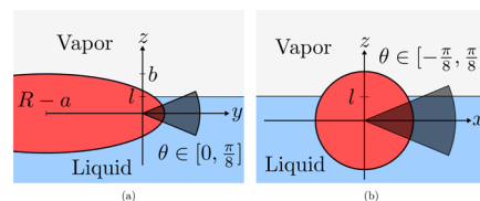
Figure 4. Systems used in the calculation of the radial distribution of the (a) tip and (b) side of the prolate ellipsoidal particle. R = b^2/a is the radius of curvature at the tip of the nanoparticle, \theta is the polar angle in the spherical coordinate system, \phi is the azimuthal angle of the cylindrical coordinate system, l is the distance from the nanoparticle center-of-mass to the GDS of the liquid–vapor interface, and a and b are the long and short radii of the nanoparticle, respectively.
