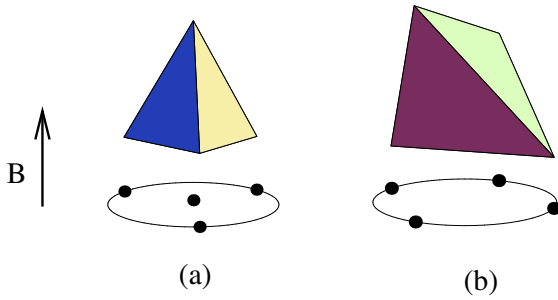
FIG. 1: Orientations of the cyclic state in an external magnetic field which breaks the spin rotational symmetry. The spin-two spinors are represented by four spin-half vectors on the unit sphere [9]. Upon increasing the magnetic field, the spinor will undergo a transition from state (a) to state (b). As indicated by the tetrahedra, orientation (a) and (b) will have rotational symmetries given by the angles 2\pi n/3 and 2\pi n/2 respectively ( n is an integer) when rotated about the vector defined by the magnetic field. These symmetries determine what types of vortices can occur for such spin configurations.
