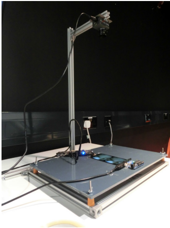
Fig. 3. Image of the apparatus showing the low speed camera, Arduino and DK2 screen
