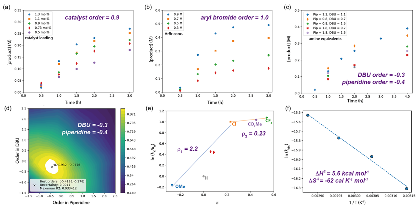
Figure 4. Kinetic profiles for photoaminocarbonylation catalysis with variation of (a) [\text{Co}_2(\text{CO})_8] , (b) p -bromoanisole, (c) piperidine, and DBU. (d) Auto-VTNA analysis. (e) Hammett plot for electronically modified aryl bromide substrates at 3 bar CO pressure ( R = \text{OMe}, \text{H}, \text{F}, \text{Cl}, \text{CO}_2\text{Me}, \text{CF}_3 ). (f) Eyring analysis plot of p -bromoanisole substrate. Reactions were tested between 318 and 348 K in increments of 10 K for analysis.
