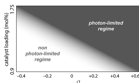
Figure 6. Simplified graphic representation of the transition between photon-limited and non-photon-limited catalysis with changes in catalyst loading and substrate electronics.
