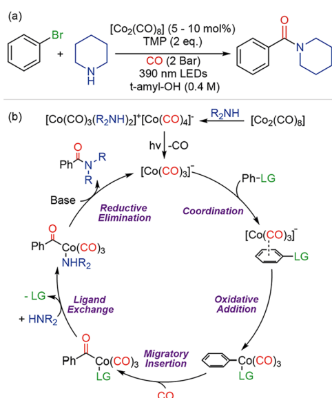
Figure 1. (a) [\text{Co}_2(\text{CO})_8] -catalyzed aminocarbonylation conditions presented by the Alexanian group. 20 (b) A recent proposed catalyst scheme is shown. 25 Cation species [\text{Co}(\text{CO})_3(\text{R}_2\text{NH})_2]^+ is omitted in catalyst cycle for clarity.
