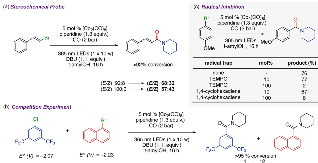
Figure 5. Mechanistic probe experiments for photocatalytic aminocarbonylation. (a) Stereochemical probe E/Z \beta -bromostyrene. (b) Competition experiment for the SET process. (c) Radical inhibition experiments using TEMPO = (2,2,6,6-tetramethylpiperidin-1-yl)oxyl and 1,4-cyclohexadiene.
