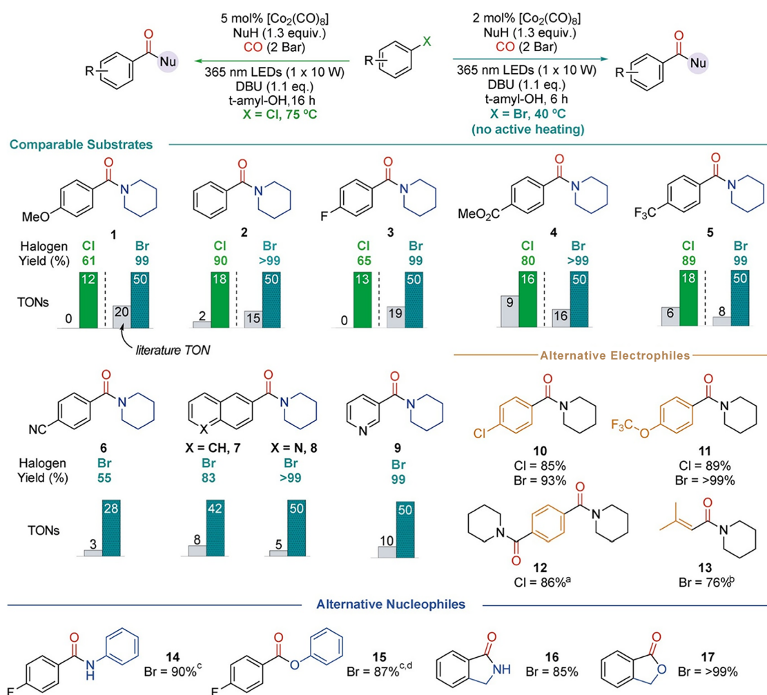
Figure 9. Reaction scope for photocatalyzed aminocarbonylation reaction, yields are isolated unless otherwise stated. TON and TOF comparison for p -bromoanisole and piperidine reagents. a 0.5 equiv of electrophile used. b Yield determined by quantitative 1 H NMR spectroscopy versus 1,3,5-trimethoxybenzene internal standard. c Yield determined by quantitative 19 F NMR spectroscopy relative to \alpha,\alpha,\alpha -trifluorotoluene internal standard. d 2 equiv of DBU used.
