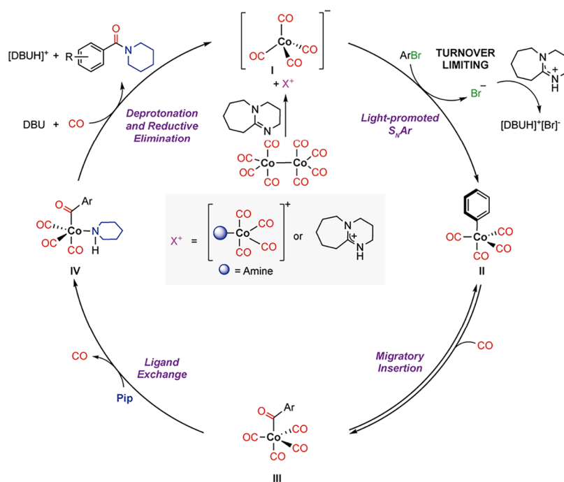
Figure 8. Updated catalytic cycle for the [Co_2(CO)_8] -catalyzed aminocarbonylation of aryl bromides.
