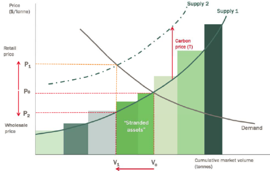
Figure 3: Simple supply-demand diagram for a fossil fuel sector (e.g., crude oil) taken from Simm et al. (2016). The x -axis reports assets with different volumes and marginal costs of production: to fix ideas, Middle Eastern oil is likely to be to the left of the curve, while Arctic deep sea reserves will likely be to the right. Drawing a demand curve gives the volume consumed by the industry, V_0 , and the market price P_0 which is both paid by consumers and received by suppliers. Considering now one type of carbon pricing, a tax T imposed by the government on the industry, raises the supply curve, which now intersects with the demand curve at a new point. The volume consumed drops to V_1 , while consumers pay P_1 but suppliers receive only P_2 . Assets represented by bars between V_0 and V_1 become stranded. See Simm et al. (2016) for further details.
