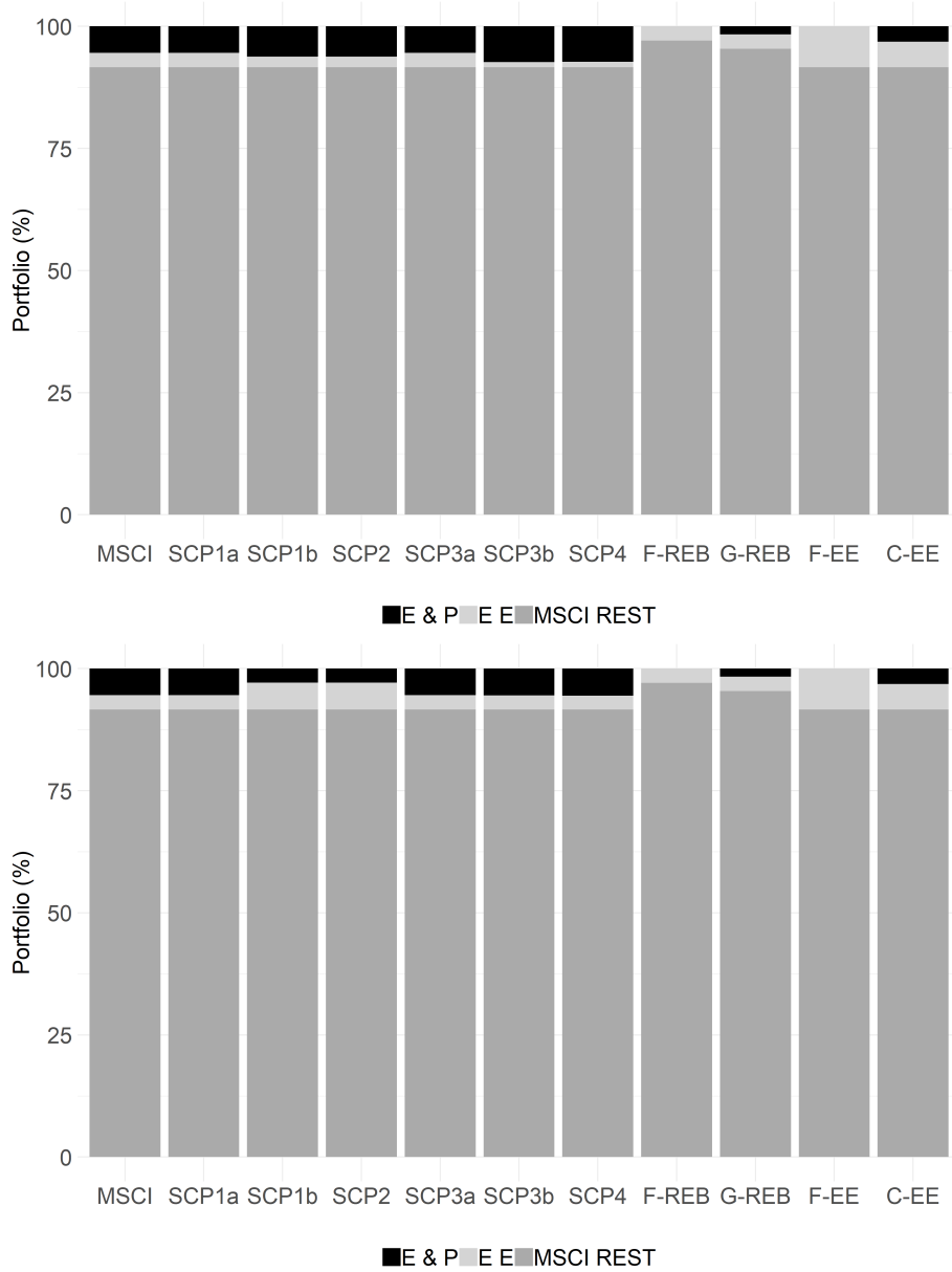
Figure 8: Portfolio weights supporting SCP1-4, as well as portfolios F-REB, G-REB, F-EE, and C-EE, for a target expected return coinciding with the one delivered by the MSCI World Index (last three year sampling period). Allocations are clustered into E&P stocks, the EE sector, and the rest of the MSCI World portfolio. The top panel reports the case with an undervaluation view on the EE sector of 4% p.a., whereas the bottom panel reports results for the same case but with the allocation to group D of E&P stocks (31 firms in total) capped at the current MSCI World allocation level. Views on E&P stocks are as per figure 4. The top panel consider the case of \tau = 0.99 , the bottom panel the case of \tau = 0.25 .
