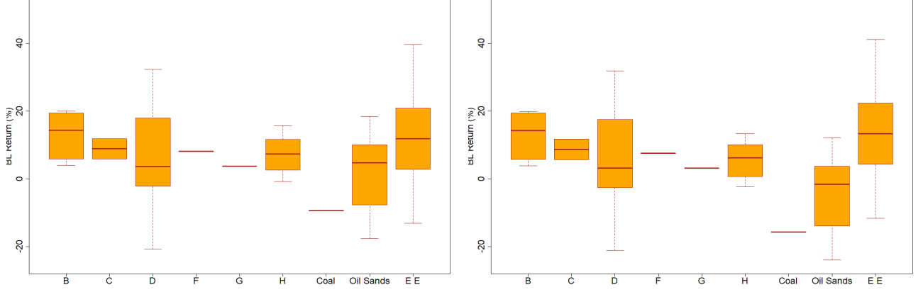
Figure 5: Black-Litterman (BL) expected return vector \mu_{BL} for confidence levels \tau = 0.25 and \tau = 0.99 , with components clustered into the main E&P classes, the EE sector and the rest of the MSCI World index. By expression (3.8), the case of \tau approaching one can be understood as yielding the Bayesian prior \mu_0 . As confidence in the views increases, the BL adjustment becomes more material for classes Coal and Oil Sands in particular.
