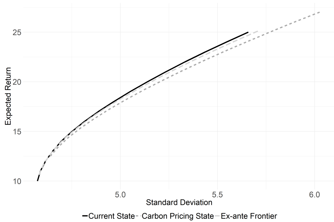
Figure 1: Efficient frontiers in the current (business as usual) state and in the carbon pricing state. In addition to the state-dependent frontiers, we plot the ex-ante frontier obtained by applying the methodology of section 3.
