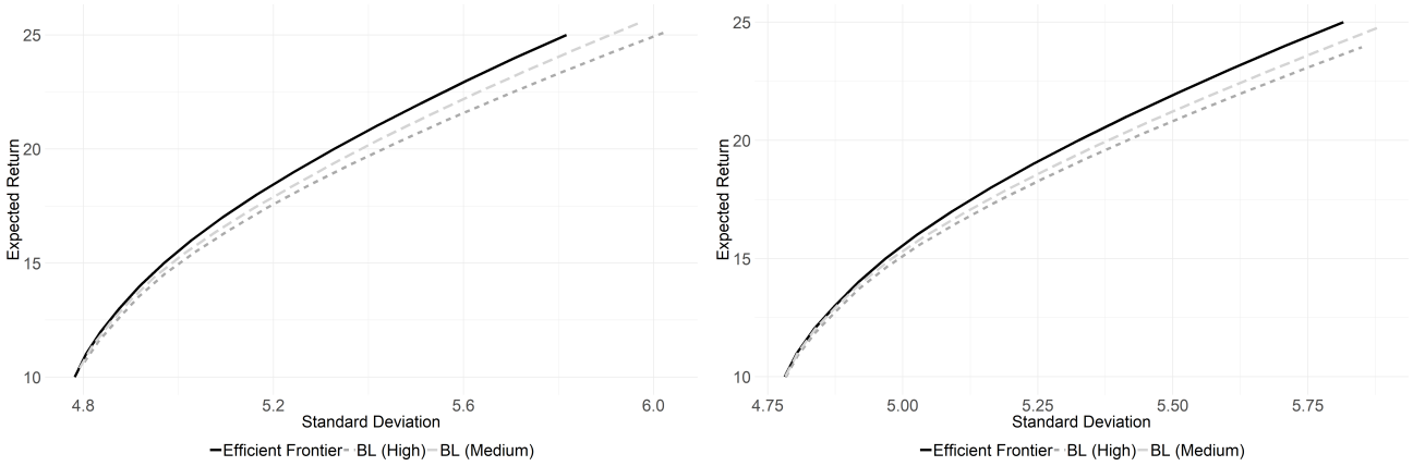
Figure 6: Baseline efficient frontier (plug-in estimators) and BL frontiers for portfolios SCP1(b) (left panel) and SCP2 (right panel) in the cases of medium ( \tau = 0.5 ) and high ( \tau = 0.99 ) confidence. The case of \tau = 0.25 gives a frontier very close to the baseline.
