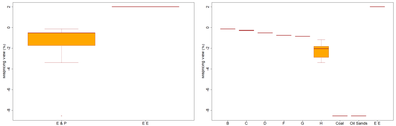
Figure 4: Mispricing of EE and E&P stocks (left panel), and cross-sectional disaggregation of views within the E&P sector (right panel). E&P stocks are clustered into eight groups, depending on the severity of their exposure to carbon pricing. Groups are labeled from A to I. Group A is not reported as the impact of carbon pricing is found to be negligible. Group E corresponds to coal stocks, group I to Oil Sands. Mispricing is expressed in terms of average stock depreciation (% p.a.) across carbon pricing scenarios.
