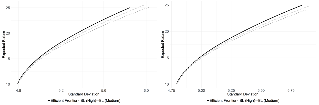
Figure 7: Baseline efficient frontier (plug-in estimators) and BL frontiers for portfolios SCP3(b) (left panel) and SCP4 (right panel) in the cases of medium ( \tau = 0.5 ) and high ( \tau = 0.99 ) confidence. The case of \tau = 0.25 gives a frontier very close to the baseline.
