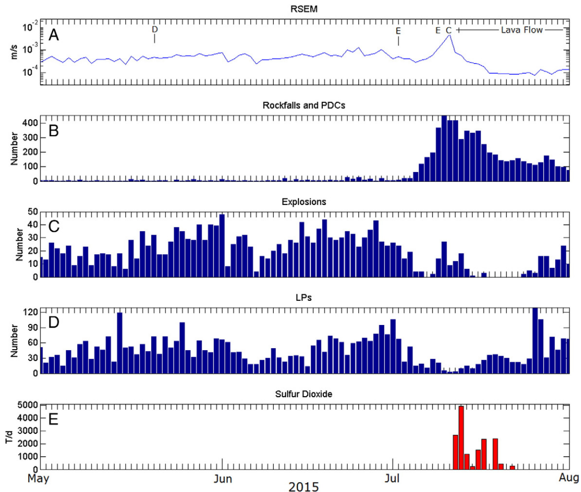
Fig. 1. A) RSEM. Daily number of events detected by automatic recognition based on Hidden Markov Models (HMMs, Benítez et al., 2009), B) rockfalls and PDCs, C) explosions, D) LPs, E) Sulfur dioxide measured with COSPEC starting on July 12th. 'D' = Dome extrusion, 'E' = moderate explosion, 'C' = Lava dome collapse.
