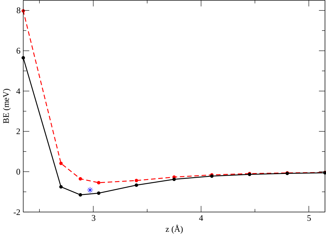
FIG. 1: The binding energy curve for the \text{He}_2 dimer computed using HF+MP2, red dotted line, and HF+MP2(B3LYP), black solid lines. The experimental value is shown by the blue star [18].
