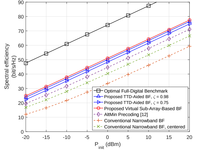
Fig. 13. Average spectral efficiency versus initial transmit power in dBm.
