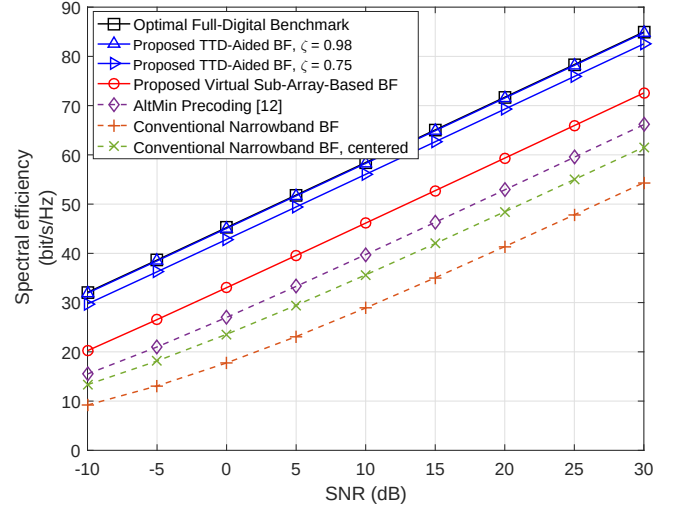
Fig. 9. Average spectral efficiency versus SNR.
