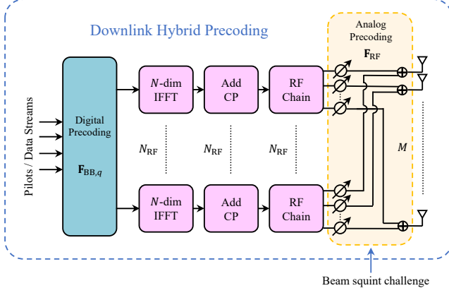
Fig. 2. The downlink hybrid precoding diagram based on phased array.
