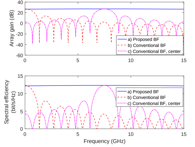
Fig. 7. Array gain across the whole frequency band of the proposed analog beamforming design based on TTD lines.
