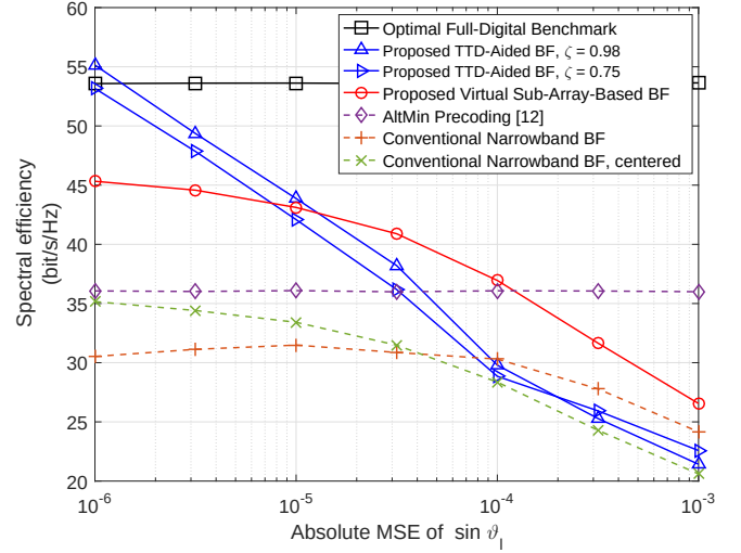
Fig. 14. Average spectral efficiency versus estimation error of path angles.
