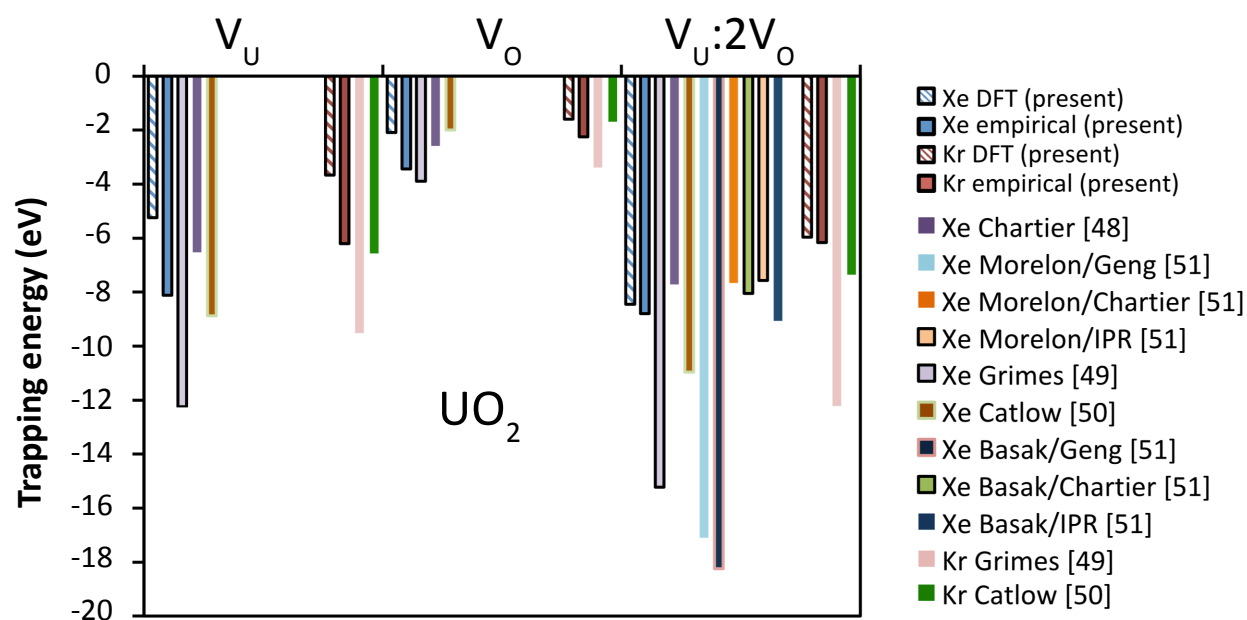
Figure 5: The trapping energy for the incorporation of a Xe or Kr atom starting at the interstitial site into an oxygen vacancy (reaction 10), uranium vacancy (reaction 11) or Schottky defect (reaction 12). DFT results (partially filled columns) are reported from the present study (using Table 2) for comparison with the new empirical potential and a range of alternative empirical potentials (solid columns).
