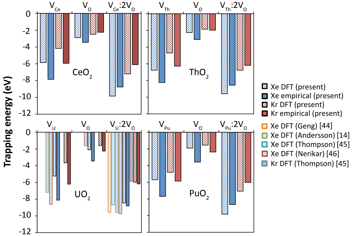
Figure 4: The trapping energy for the incorporation of a Xe (blue) or Kr (red) atom starting at the interstitial site into an oxygen vacancy (reaction 10), cation vacancy (reaction 11) or Schottky defect (reaction 12). DFT results (partially filled columns) are reported from the literature [14, 44, 45, 46] and the present study (using Table 2) for comparison with the new empirical potential potential (solid columns).
