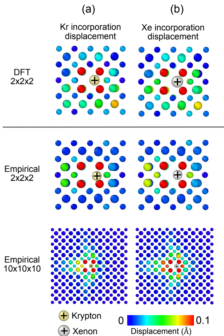
Figure 3: The displacement of U and O atoms due the incorporation of a) Kr and b) Xe into a pre-existing Schottky defect. The color of the U and O atoms corresponds to the magnitude of the displacement. Xe and Kr atoms are shown by grey and beige spheres respectively and are marked with a black cross.
