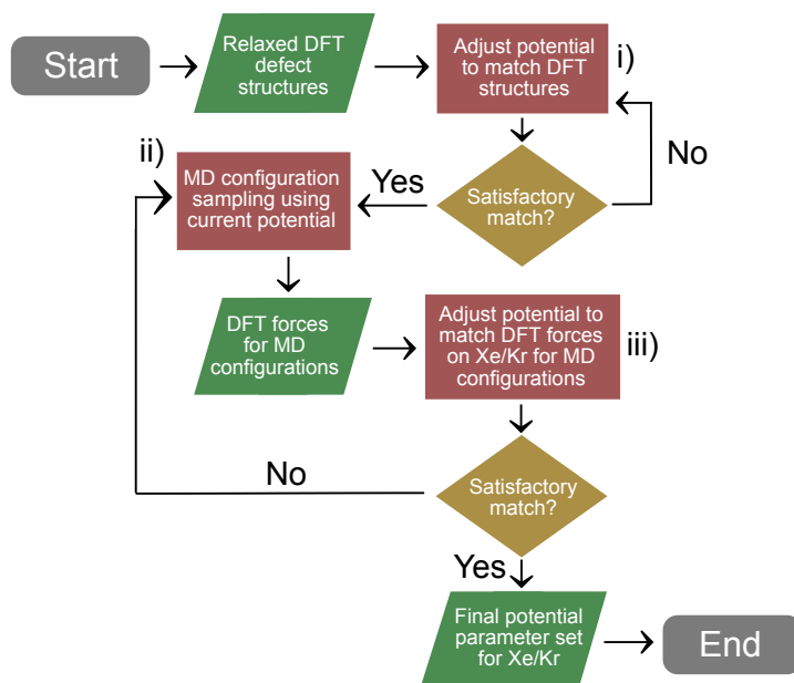
Figure 1: A schematic illustration of the fitting procedure conducted for the development of the potential parameters for Xe and Kr in \text{CeO}_2 , \text{ThO}_2 , \text{UO}_2 and \text{PuO}_2 . The final parameter set is reported in Table 4.
