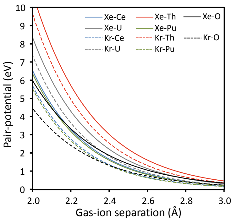
Figure 2: The pair-potential interactions for plotted as a function of gas-ion separation for Xe-O, Xe-Ce, Xe-Th, Xe-U, Xe-Pu, Kr-O, Kr-Ce, Kr-Th, Kr-U and Kr-Pu. Expanded views of the potential are shown near the oxygen-gas separation, the cation-gas separation and the potential minima.
