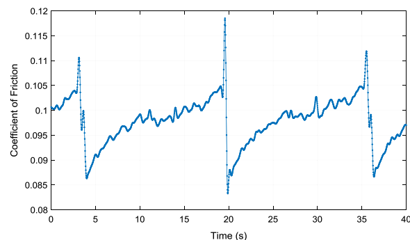
Fig. 15. – Averaged experimental coefficient of friction, showing 3 pocket entrainments. The experiment was conducted under a (tangential) sliding speed of 0.0035 m/s wherein the contact is predominantly in the mixed lubrication regime.
