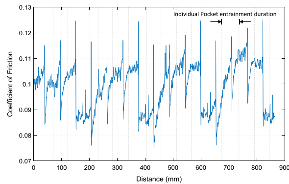
Fig. 14. – Raw experimental coefficient of friction data, obtained using the pin-on-disc setup from a test in which 15 pocket entrainments were observed. The experiment was conducted under a (tangential) sliding speed of 0.0035 m/s wherein the contact is predominantly in the mixed lubrication regime.
