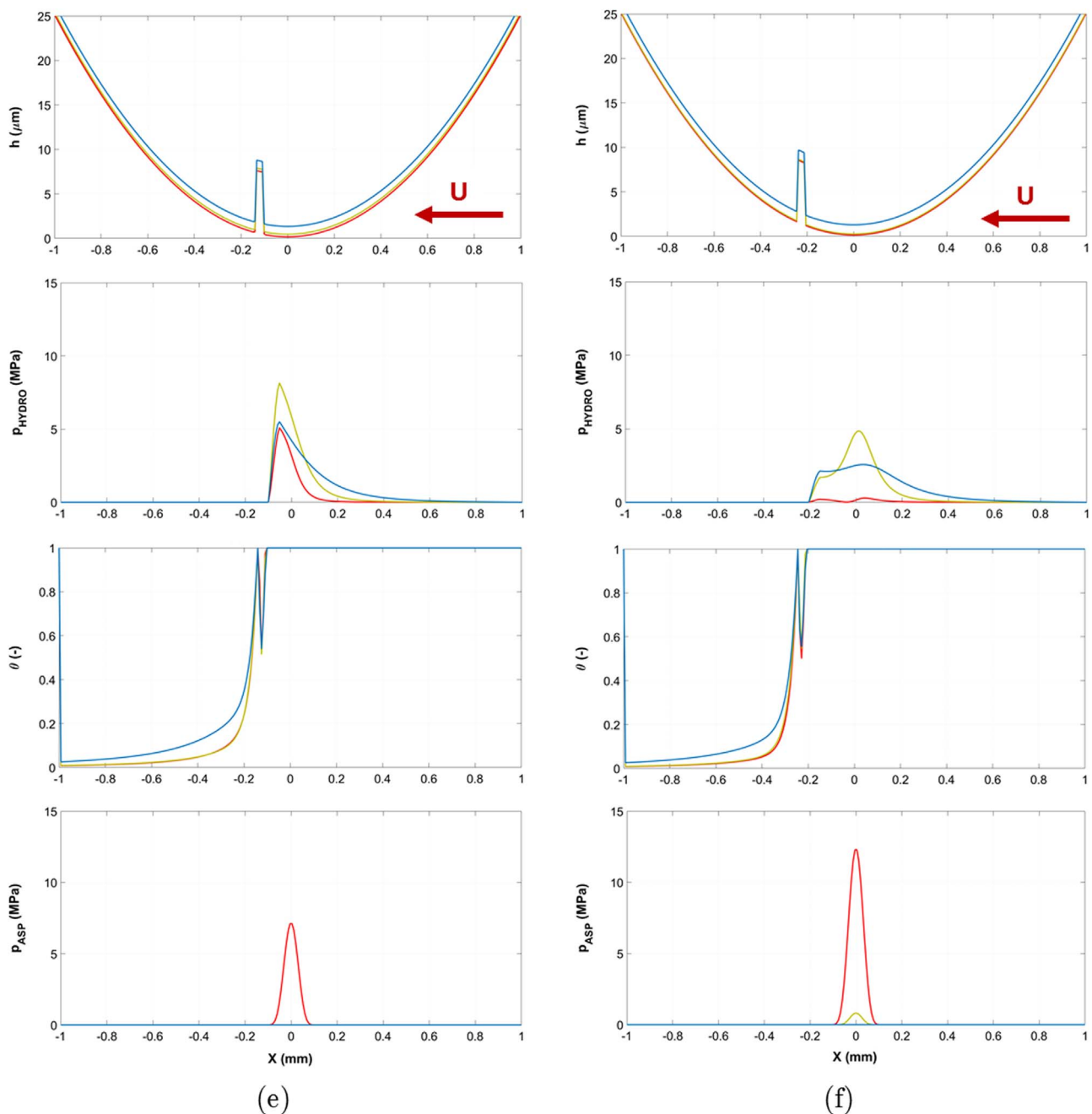
Fig. 12. Variation of the film thickness, fluid pressure, film fraction (cavitation) and asperity contact pressure along the pad center ( z = 0 ) over the sliding distance as the pocket leaves the contact. (e) and (f) are the sliding positions compatible with those illustrated in Fig. 7. V = 0.0035 m/s (red, boundary regime), V = 0.035 m/s (yellow, mixed regime) and V = 0.35 m/s (blue, full-film regime). (For interpretation of the references to color in this figure legend, the reader is referred to the web version of this article.)
