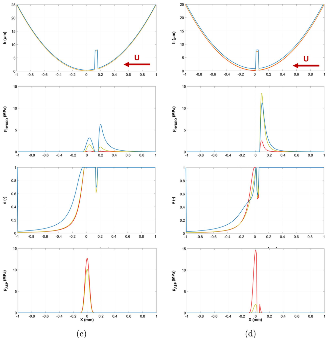
Fig. 11. Variation of the film thickness, fluid pressure, film fraction (cavitation) and asperity contact pressure along the pad center ( z = 0 ) over the sliding distance during the pocket entrainment. (c) and (d) are the sliding positions compatible with those illustrated in Fig. 7. V = 0.0035 m/s (red, boundary regime), V = 0.035 m/s (yellow, mixed regime) and V = 0.35 m/s (blue, full-film regime). (For interpretation of the references to color in this figure legend, the reader is referred to the web version of this article.)
