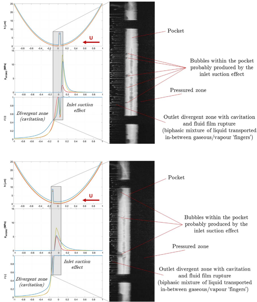
Fig. 8. Predicted hydrodynamic pressure and film fraction (left) and fluorescence images (right) of the moving pocket at the inlet (top) and just after the inlet (bottom) zones measured in the friction tests reported in [3]. Both cavitation at the outlet divergent region with fluid film rupture, along with tiny bubbles within the pocket probably associated with the inlet suction effect are shown in the images and correlated with simulated results.
