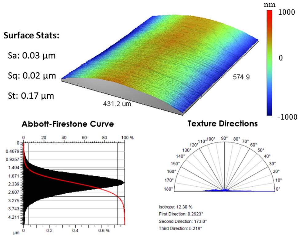
Fig. 5. Three-dimensional surface topography of the barrel-shaped steel specimen as obtained by the Veeco Wyko optical profiler. A surface roughness analysis showed that the roughness heights follow an anisotropic Gaussian distribution.
