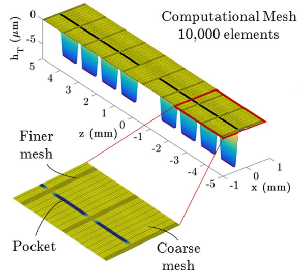
Fig. 6. Film thickness geometry projected on the pad mesh for a given instant as the pocket moves through the pad.
