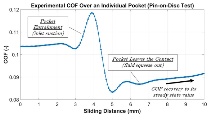
Fig. 9. Average experimental coefficient of friction over an individual pocket measured from the pin-on-disc test described in this work. The experiment was conducted under a (tangential) sliding speed of 0.0035 m/s wherein the contact is predominantly in the mixed lubrication regime.
