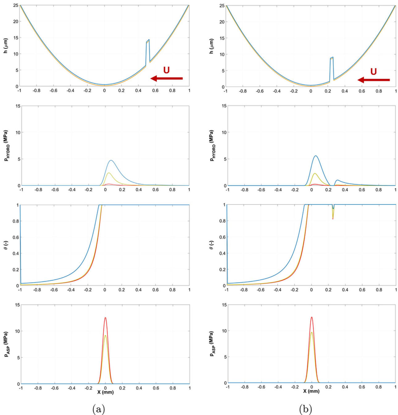
Fig. 10. Variation of the film thickness, fluid pressure, film fraction (cavitation) and asperity contact pressure along the pad center ( z = 0 ) over the sliding distance before the pocket entrainment. (a) and (b) are the sliding positions compatible with those illustrated in Fig. 7. V=0.0035 m/s (red, boundary regime), V=0.035 m/s (yellow, mixed regime) and V=0.35 m/s (blue, full-film regime). (For interpretation of the references to color in this figure legend, the reader is referred to the web version of this article.)
