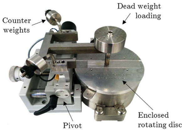
Fig. 2. Experimental setup on Anton Paar high temperature tribometer (THT).
