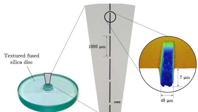
Fig. 4. Two-dimensional surface plot of a section of the laser surface-textured fused silica disc and a 3D surface profile of one pocket.
