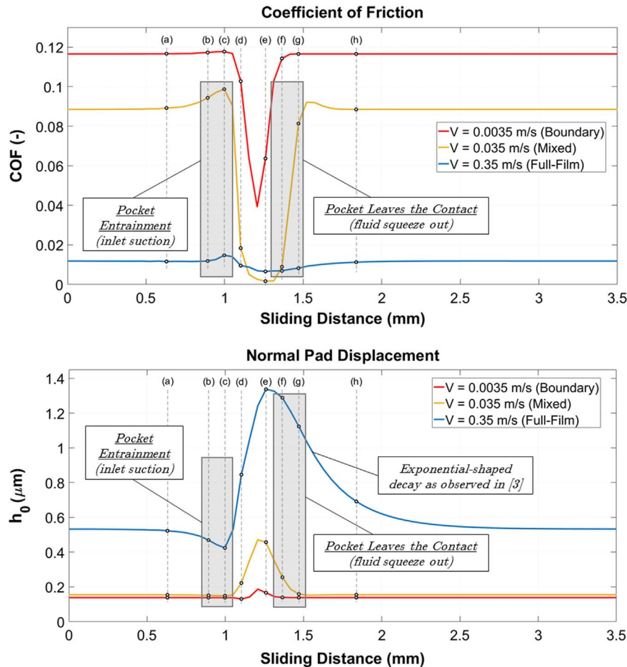
Fig. 7. Variation of the coefficient of friction (top) and normal pad displacement (bottom) over the sliding distance as the moving pocket passes through the fixed pad. Results for three sliding velocities are considered to illustrate the transient effects under different lubrication regimes.
