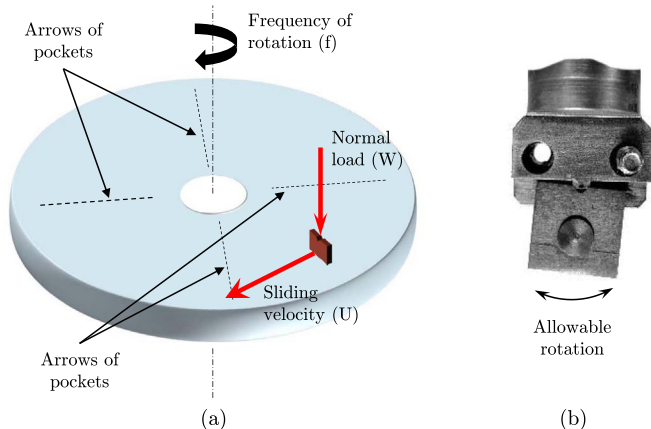
Fig. 3. a) Schematic representation of the simulated piston ring/cylinder liner contact for testing at constant sliding speed; b) Front view of the piston ring specimen holder with half of the clamp removed.
