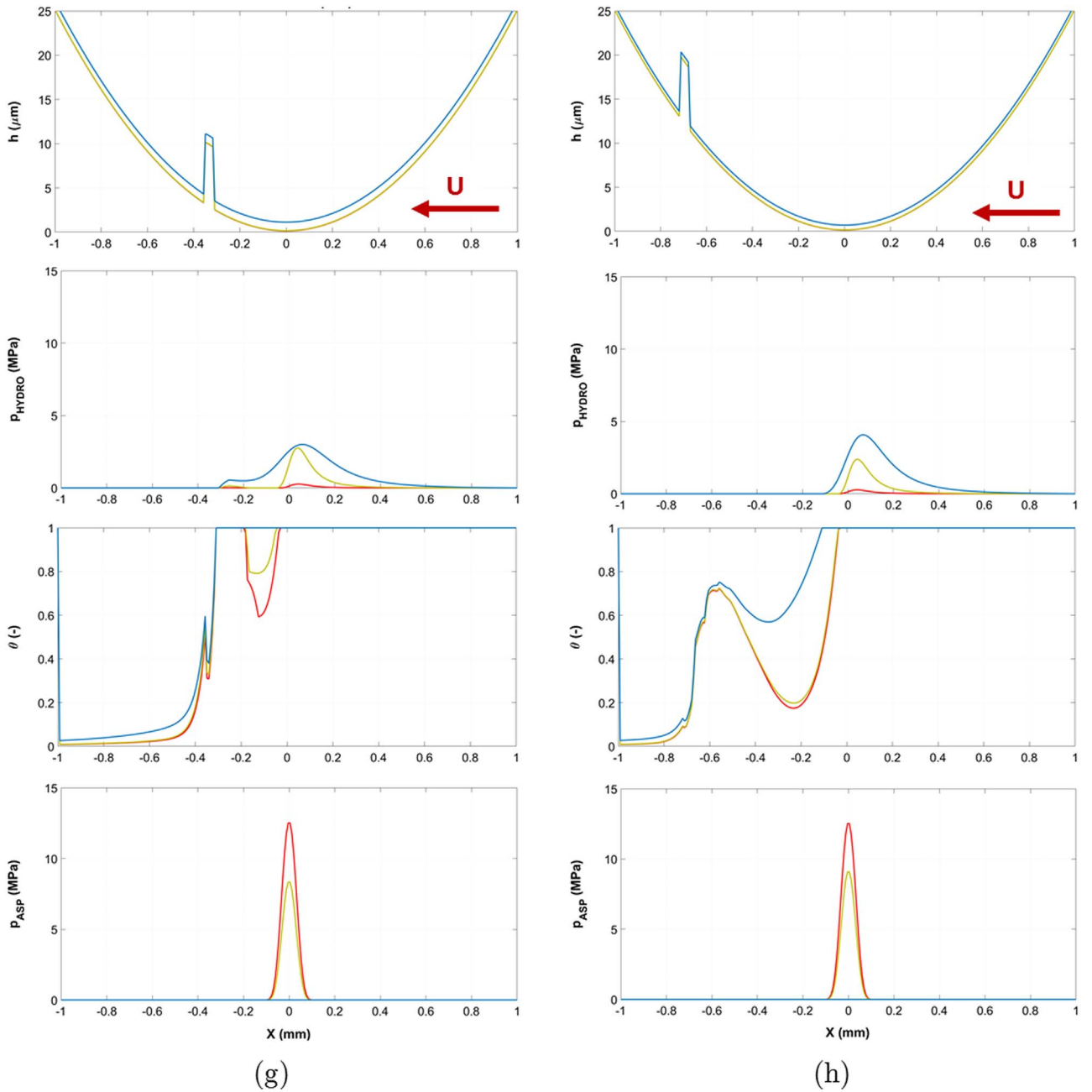
Fig. 13. Variation of the film thickness, fluid pressure, film fraction (cavitation) and asperity contact pressure along the pad center ( z = 0 ) over the sliding distance after the pocket leaves the contact. (g) and (h) are the sliding positions compatible with those illustrated in Fig. 7. V=0.0035 m/s (red, boundary regime), V=0.035 m/s (yellow, mixed regime) and V=0.35 m/s (blue, full-film regime). (For interpretation of the references to color in this figure legend, the reader is referred to the web version of this article.)
