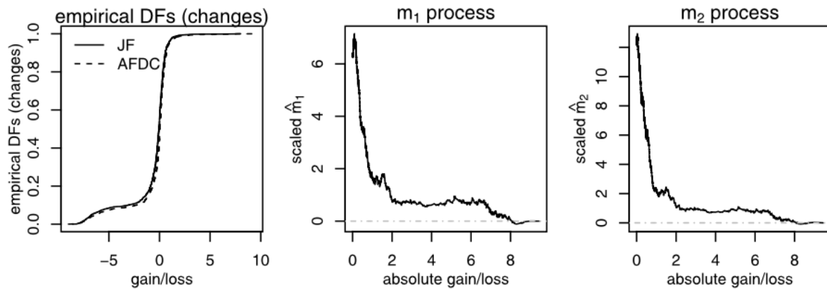
Fig. 1. Empirical distribution functions of changes in income near the JF time limit and the T_2(F) coordinate processes that are used to test loss aversion-sensitive dominance. The second and third panels show the two coordinate functions in T_2(F_n) defined in Eq. (12). The large positive values in the second panel drive the rejection of the hypothesis F_{JF} \geq F_{AFDC} seen in Table 1.
