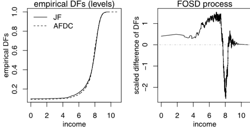
Fig. 2. Empirical distribution functions of (levels of) post-TL income and the resulting process that is used to test first-order stochastic dominance. Although there are positive values in the second panel, they are not large enough to drive a rejection of the hypothesis G_{JF} \succeq_{FOSD} G_{AFDC} , as seen in Table 1.
