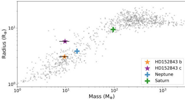
Figure 11. The plot show mass versus radius of HD152843 b and c compared with the sample of known planets with masses and radii known to better than 50 percent precision, sourced from the TEPICAT data base. For reference, Neptune and Saturn are shown as blue and green pluses, respectively.
