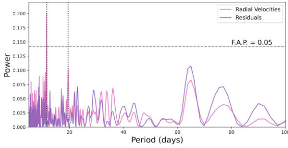
Figure 5. Lomb–Scargle periodograms of the raw RVs (pink) and the residuals of the two-planet fit (purple). The 5 per cent FAP level for each periodogram is indicated by the horizontal dashed line of the same colour. The two vertical lines are the estimated periods of planet b (left) and planet c (right).
