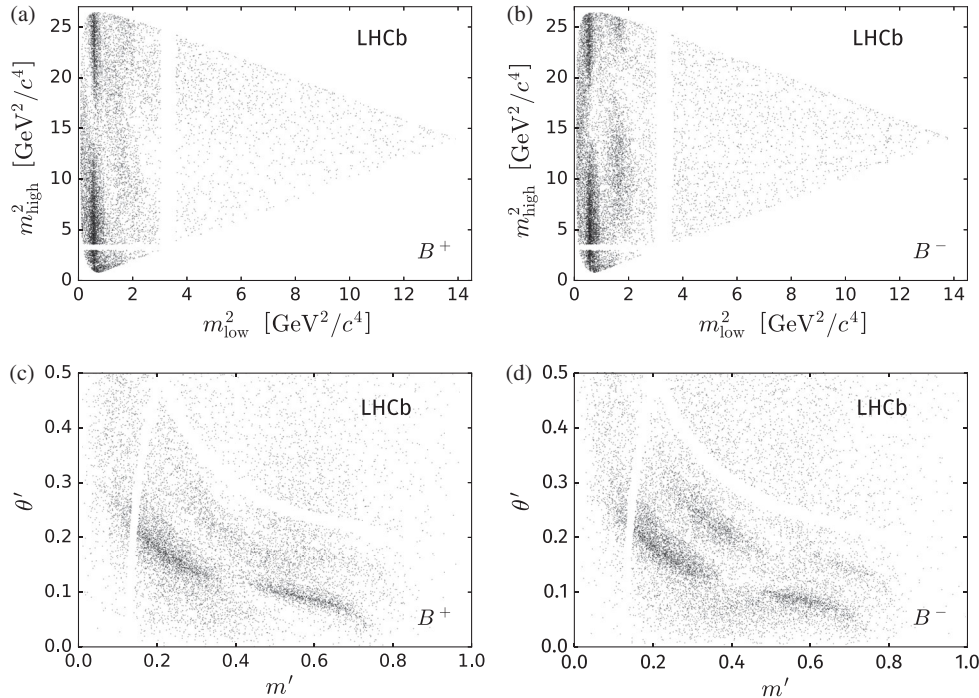
FIG. 2. Conventional Dalitz-plot distributions for (a) B^+ and (b) B^- , and square Dalitz-plot (defined in Sec. V A 1) distributions for (c) B^+ and (d) B^- candidate decays to \pi^\pm\pi^+\pi^- . Depleted regions are due to the \bar{D}^0 veto.
