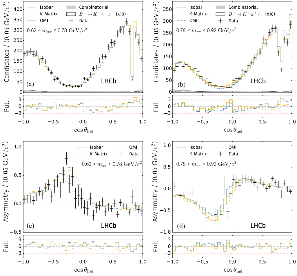
FIG. 10. Fit projections of each model on \cos \theta_{\text{hel}} in the regions (a) below and (b) above the \rho(770)^0 resonance pole, with the corresponding asymmetries shown beneath in panels (c) and (d). The pull distribution is shown below each fit projection.
