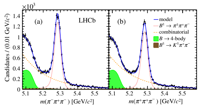
FIG. 1. Invariant-mass fit model for (a) B^- and (b) B^+ candidates reconstructed in the \pi^\mp \pi^+ \pi^- final state for the combined 2011 and 2012 data taking samples. Points with error bars represent the data while the components comprising the model are listed in the plot legend.
