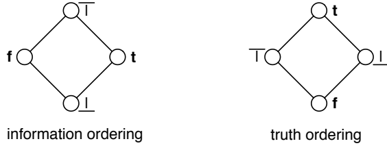
Figure 1. The information and truth orderings on elements of the Belnap space.
