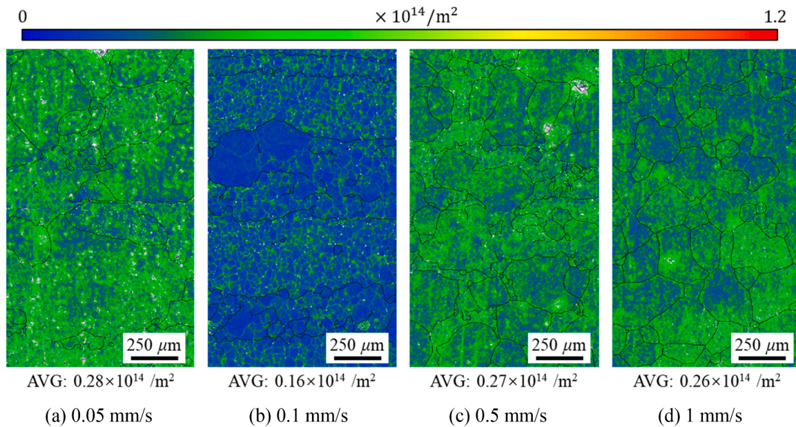
Fig. 21. Geometrically necessary dislocation (GND) density maps at selected zones from profile extruded at different speeds.
