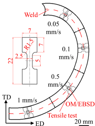
Fig. 5. Tensile specimen and sampling locations for post-extrusion examination.
