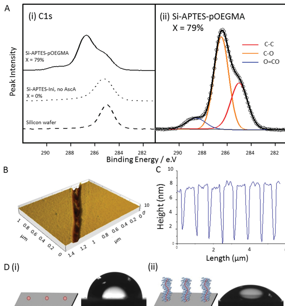
Figure 1. Demonstration and characterization of surface-initiated polymer brush growth from functionalized 2D silicon surfaces. A) XPS analysis of pOEGMA grafting from a silicon wafer functionalized with APTES-Ini with controls (dashed bottom trace), silicon functionalized with APTES-Ini that underwent polymerization with no reducing agent, ascorbic acid (AScA, dotted middle trace), and pOEGMA grafting from a silicon wafer (top trace, left). Conversion by ^1\text{H-NMR} (X) is included above each trace. Si-APTES-pOEGMA sample with the C1s peaks fitted (right). B) AFM scratch test and C) representative profile of pOEGMA grafted from silicon wafers. D) Water contact angle measurement of a silicon wafer functionalized with (i) APTES-Ini and (ii) following grafting of pOEGMA.
