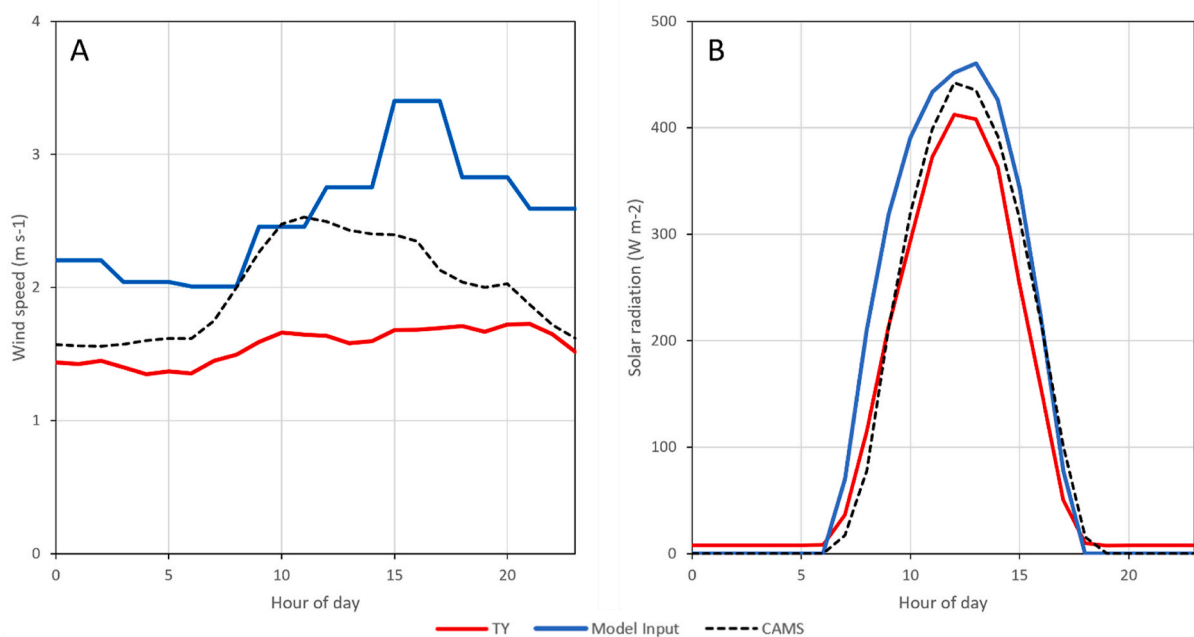
Fig. 6. Mean diurnal variation of (a) wind speed, and (b) solar radiation.
