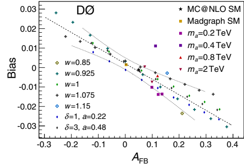
FIG. 7 (color online). The bias as a function of the input A_{\text{FB}} . Axigluon scenarios are indicated in the legend by the mass of the axigluon, m_a . The toy models are labeled by parameters w , a , and \delta of Eq. (8). Unless stated otherwise w = 1 , a = 0 , and \delta = 1 . For each set of a , \delta , and w , the value of \mu is varied to produce different input asymmetries. The dashed line indicates the calibration applied to the inclusive measurement and the dotted lines indicate the assigned calibration uncertainties. The point significantly outside of the dotted lines corresponds to an axigluon mass of 0.4 TeV and is discussed in the text.
