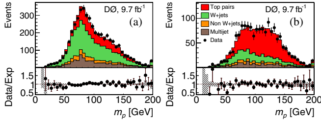
FIG. 1 (color online). The reconstructed m_p for l + 3 jet events with (a) one and (b) two or more b tags. Sample composition determination is discussed in Sec. VI. The ratio between the data counts and the model expectation is shown in the lower panel, with the hashed area representing the systematic uncertainties.
