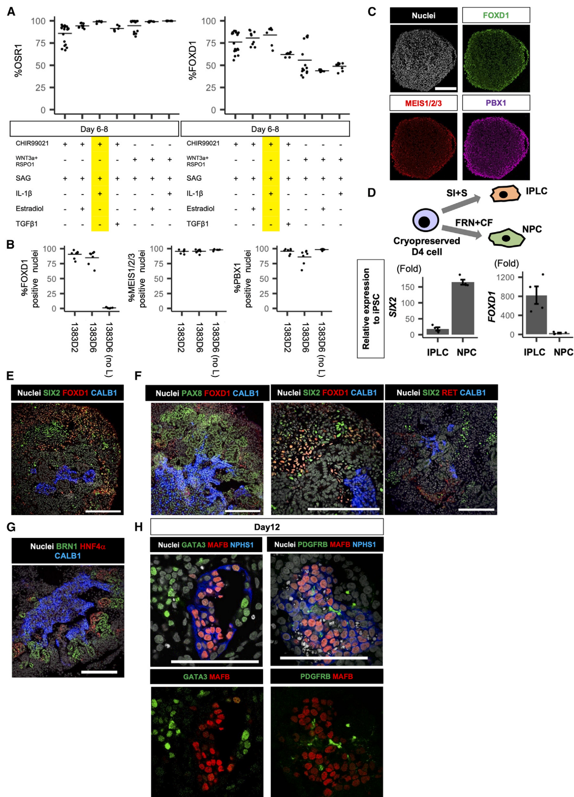
Figure 3. Efficient induction of IPLCs from hiPSCs
