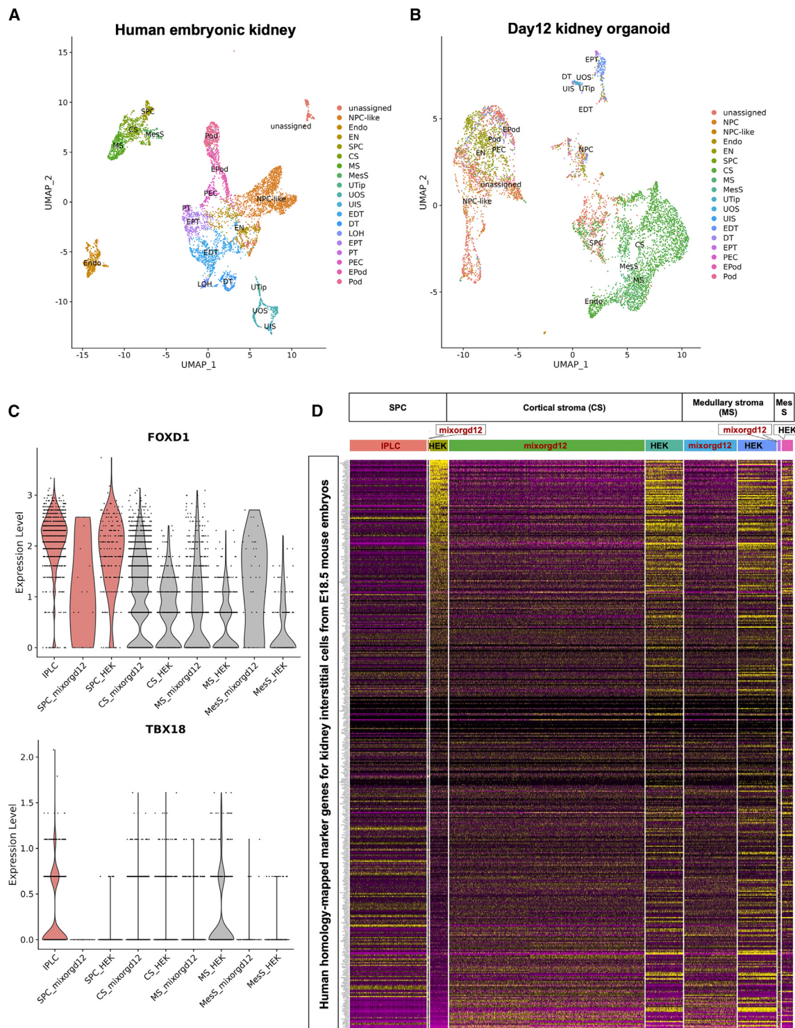
Figure 4. scRNA-seq analysis of day-12 kidney organoids generated from hiPSC-derived IPLCs, NPCs, and NDCs
