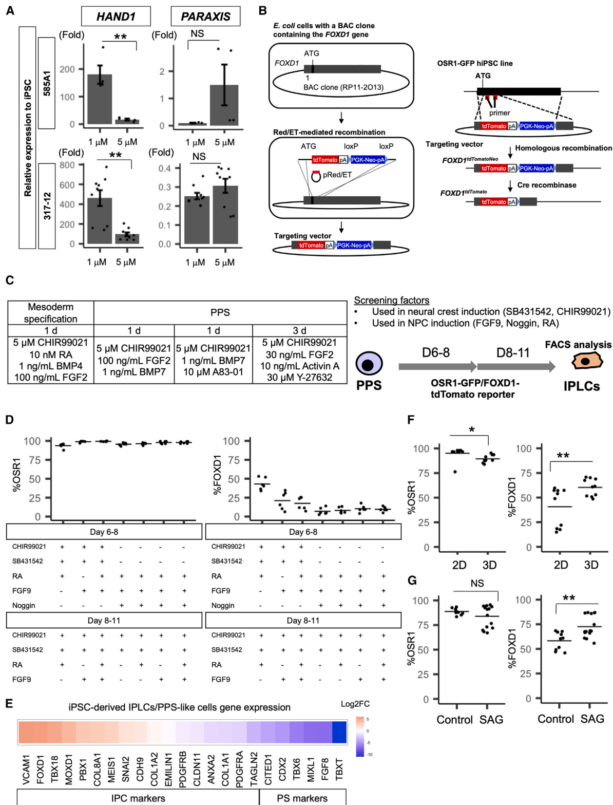
Figure 1. Induction of renal IPLCs from hiPSCs
