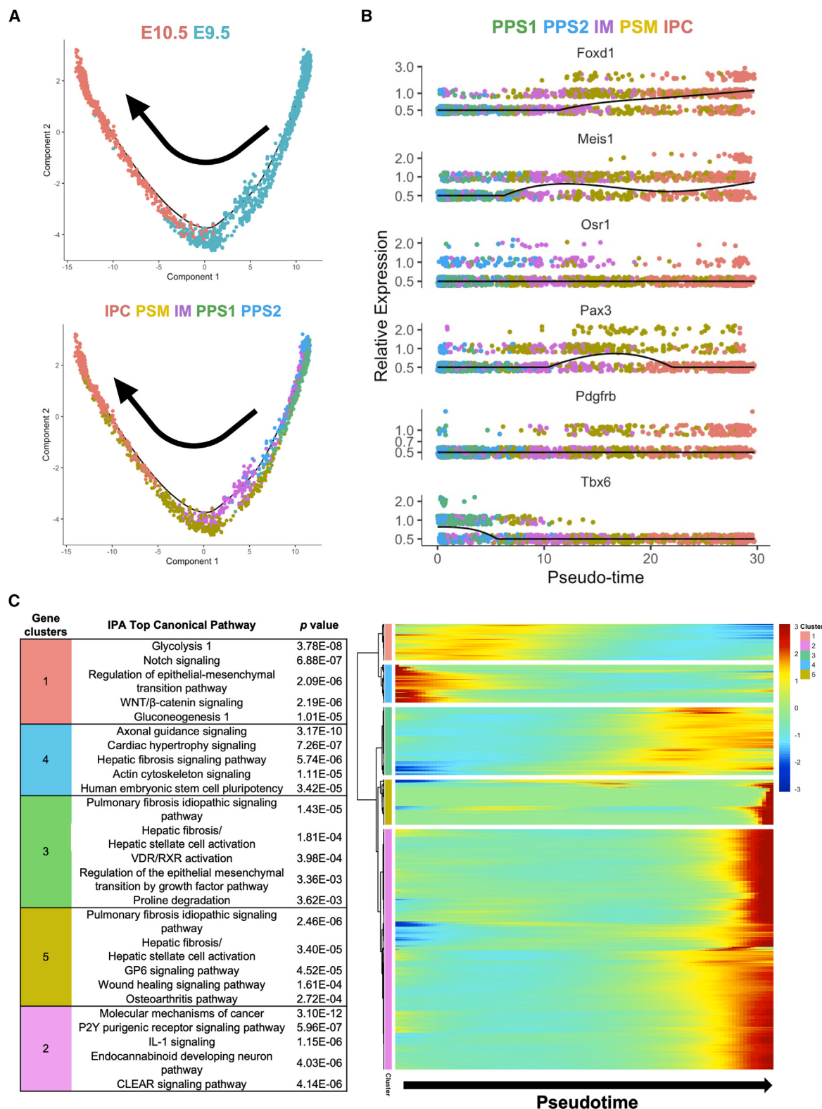
Figure 2. Molecular events during transition from PPS to metanephric IPCs
