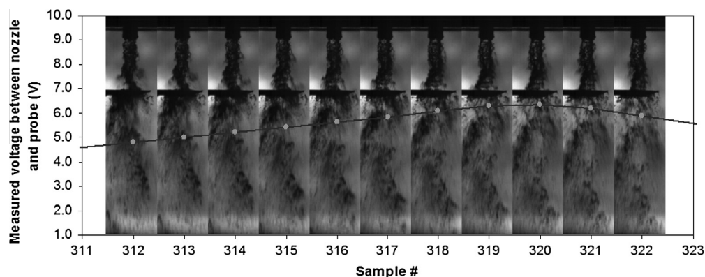
Fig. 9. Sequence of temporally resolved shadowgraphic images ( We = 526 and MR = 171 ) with the simultaneously measured voltage between the nozzle and the probe (black horizontal line on images) superimposed. The higher voltages indicate lower electrical connectivity.
