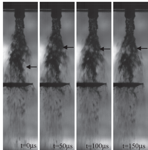
Fig. 7. Time resolved imaging reveals the location of liquid jet breaking point, which could be missed by single frame shadowgraphy. The horizontal dark line in the middle of the images is the electrical connectivity probe. The black arrows indicate the location of the liquid jet breakup on each image. (The example shown is for Re = 5442 , We = 526 and MR = 171 ).
