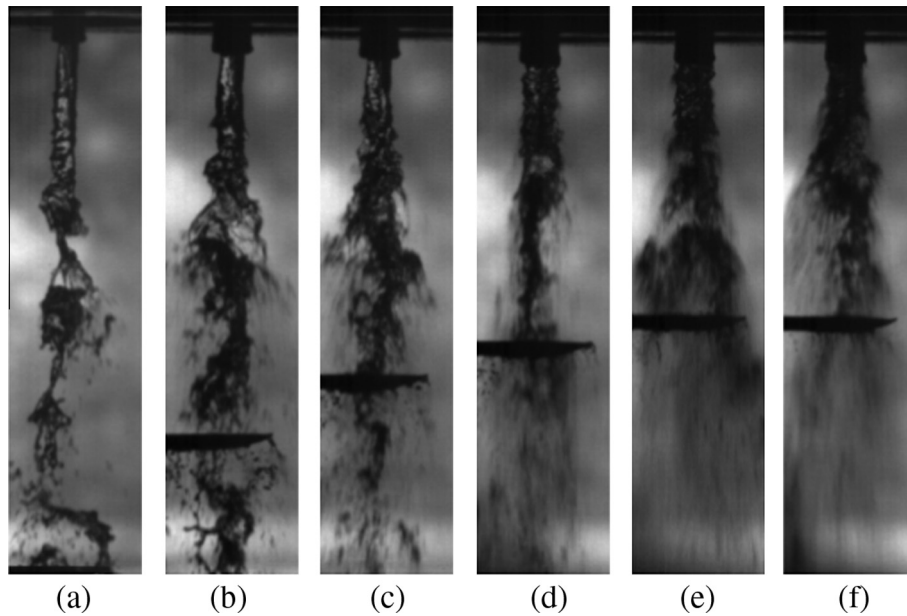
Fig. 5. Examples of the shadowgraphic jet morphology for all the considered flow conditions. (a) MR = 27 , (b) MR = 61 , (c) MR = 109 , (d) MR = 171 , (e) MR = 246 and (f) MR = 335 . The horizontal dark line is the electrical connectivity probe.
