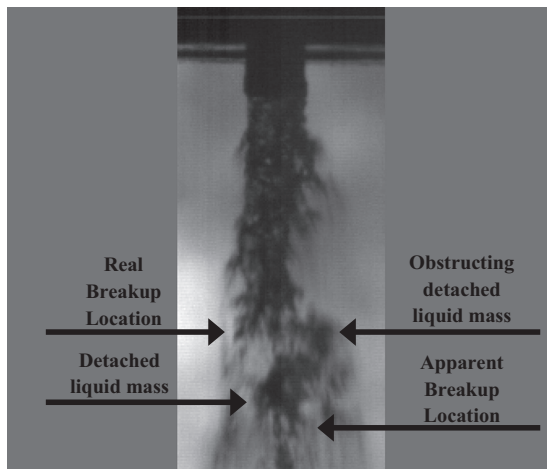
Fig. 6. Demonstration of ambiguity of shadowgraphic measurements of breakup length. If the liquid jet is imaged from the left side and recorded at the right side, the detached liquid mass will obstruct the observation of the breakup point and the breakup length will appear about 50% longer than the real value.
