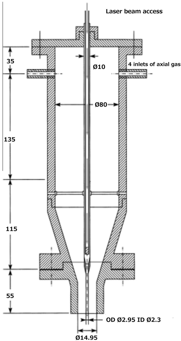
Fig. 4. Geometry of coaxial air-blast atomiser.
