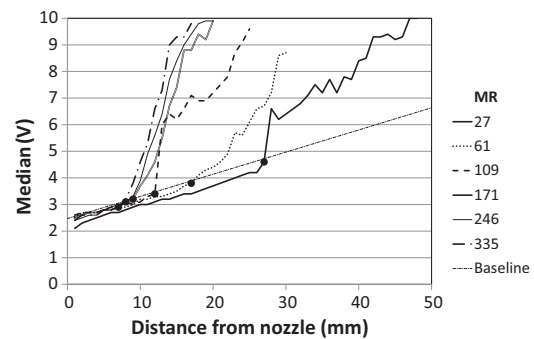
Fig. 15. Evaluation of the liquid jet breakup length based on the median value of the measured potential. The added 'dot' on each line indicates the considered location of the break-up length of the liquid jet for that operating condition.
