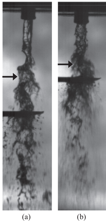
Fig. 8. Instantaneous images of the needle probe in contact with the main liquid jet core through minor physical connectivity. (a) We = 185 and (b) We = 762 . The black arrow shows the location of the breakup, which occurs upstream of the location of the needle probe. The respective measured voltages of 4.1 and 3.9 V indicate the presence of remaining electrical connectivity.
