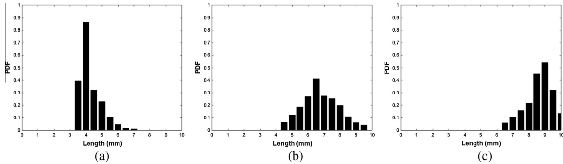
Fig. 10. Example of the evolution of the Probability Density Function of the electrical connectivity signal for the flow condition of We = 526 and MR = 171 when the voltage is measured at (a) 11 mm, (b) 14 mm and (c) 16 mm downstream of the nozzle exit.
