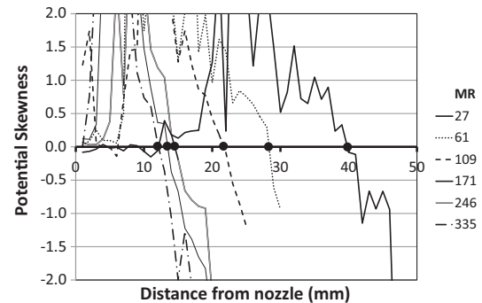
Fig. 13. Skewness of the Probability Density Function of the measured potential plotted as a function of the distance of the probe from the nozzle exit for different flow conditions indicated by the MR value. The added 'dot' on each line indicates the considered location of the break-up length of the liquid jet for that operating condition.
