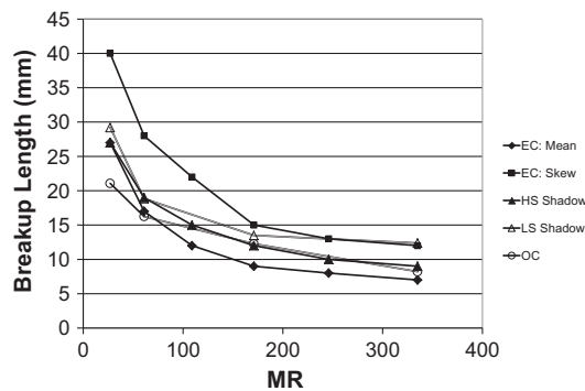
Fig. 17. Comparison of the breakup length measurements obtained by the three experimental techniques. Each technique is indicated as EC Mean: Electrical Connectivity using the mean criterion (◆), EC Skew: Electrical Connectivity using the Skewness Criterion (■), HS Shadow: High Speed Shadowgraphy (▲), LS Shadow: Low Speed Shadowgraphy (△) and OC: Optical Connectivity (○).
