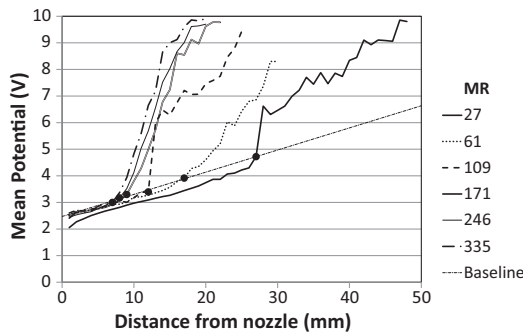
Fig. 11. Average values of the measured potential against the distance of the probe from the nozzle exit. The added 'dot' on each line indicates the considered location of the break-up length of the liquid jet for that operating condition.
