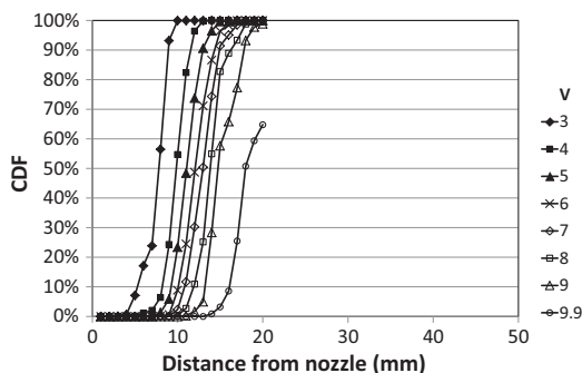
Fig. 14. Cumulative Distribution Function (CDF) of the time the measured potential is below a threshold value.
