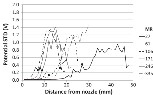
Fig. 12. Standard deviation of the fluctuations of the measured potential plotted as a function of the distance of the probe from the nozzle exit. The added 'dot' on each line indicates the considered location of the break-up length of the liquid jet for that operating condition.
