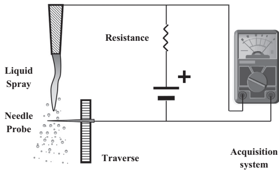
Fig. 2. Principle of the electrical connectivity technique.
