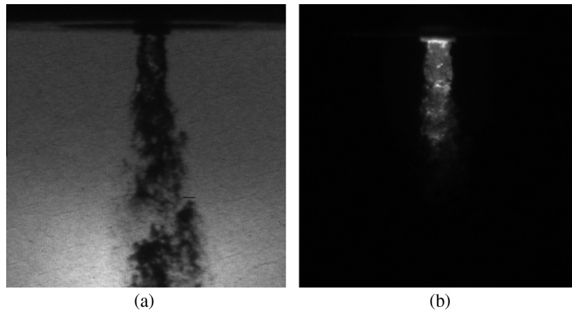
Fig. 16. Example of liquid jet visualisation with (a) shadowgraphy and (b) optical connectivity for operating condition We = 526 and MR = 171 . The optical connectivity technique is less influenced by the products of atomisation around the continuous jet, making the determination of the breakup length easier.
