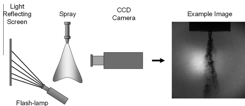
Fig. 1. Principle of photographic spray imaging using shadowgraphy.
