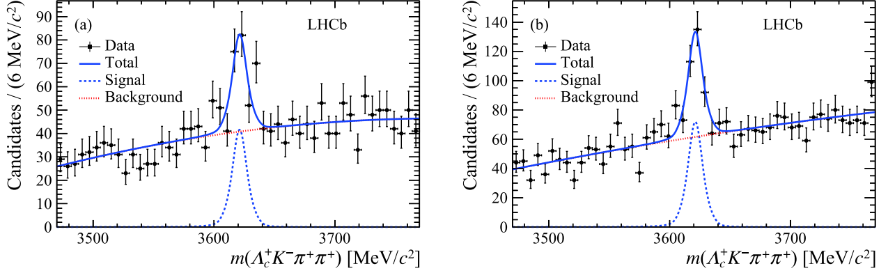
Fig. 1. (color online) Invariant-mass distributions of \Xi_{cc}^{++} candidates (a) triggered by TOS and (b) triggered by exTIS, with fit results shown.
