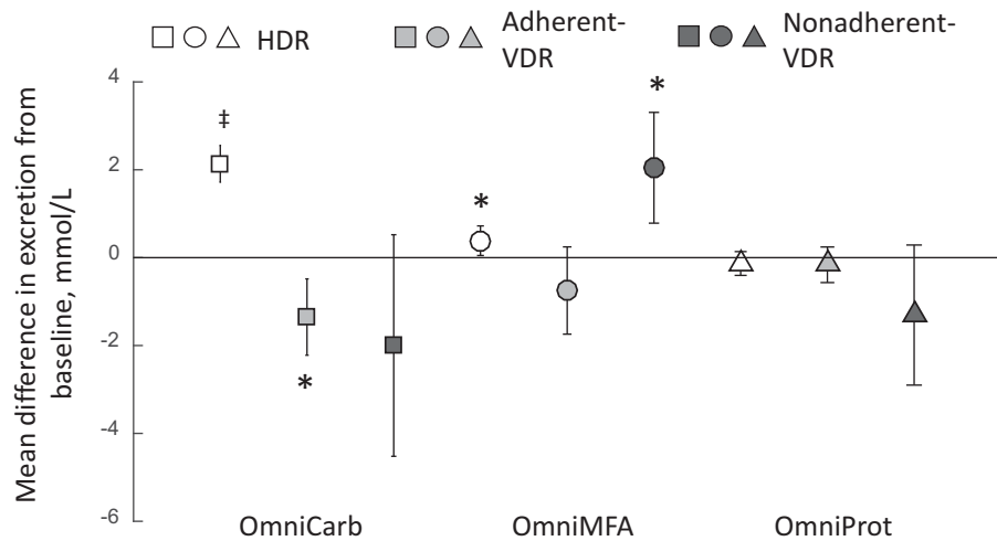
FIGURE 1 The observed mean differences in excretion for hippurate between HDR and adherent- and nonadherent-VDR groups when OmniHeart diets and their corresponding baseline spectra were compared. Open square, OmniCarb-HDR ( n = 137 ); light-grey closed square, adherent-OmniCarb-VDR ( n = 6 ); dark-grey closed square, nonadherent-OmniCarb-VDR ( n = 15 ); open circle, OmniMFA-HDR ( n = 127 ); light-grey closed circle, adherent-OmniMFA-VDR ( n = 10 ); dark-grey closed circle, nonadherent-OmniMFA-VDR ( n = 21 ); open triangle, OmniProt-HDR ( n = 113 ); light-grey closed triangle, adherent-OmniProt-VDR ( n = 10 ); dark-grey closed triangle, nonadherent-OmniProt-VDR ( n = 35 ). Error bars indicate 95% CIs. Significant t test comparison between baseline and post OmniHeart diets: * P < 0.05 ; ‡ P < 10^{-10} . HDR, homogeneous dietary response; OmniCarb, OmniHeart carbohydrate-rich diet; OmniHeart, Optimal Macronutrient Intake Trial for Heart Health; OmniMFA, OmniHeart monounsaturated fat-rich diet; OmniProt, OmniHeart protein-rich diet; VDR, variable dietary response.
