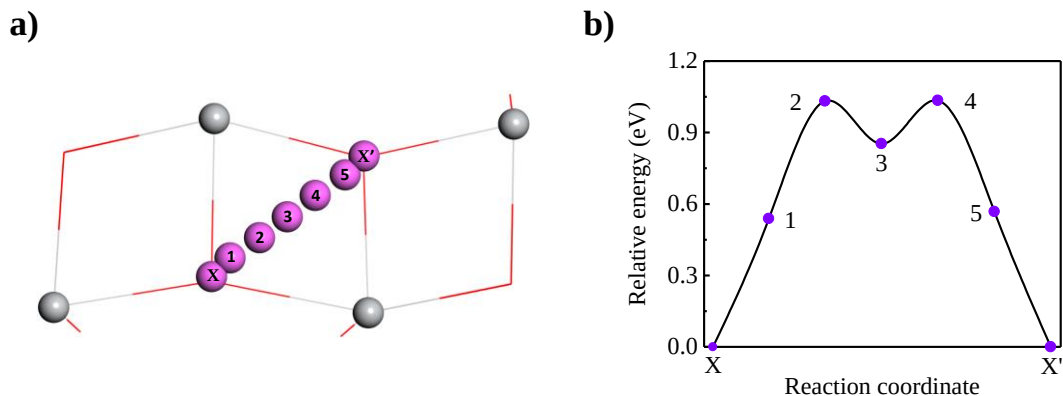
Fig. 6. a) Aluminum positions at the CI-NEB images for the GGA calculation in anatase \text{TiO}_2 . b) Energy profile for aluminum diffusion between adjacent octahedral in anatase \text{TiO}_2 , Interstitial sites (X and X') are equivalent. Silver and purple ball represent Ti and Al atoms, respectively.
