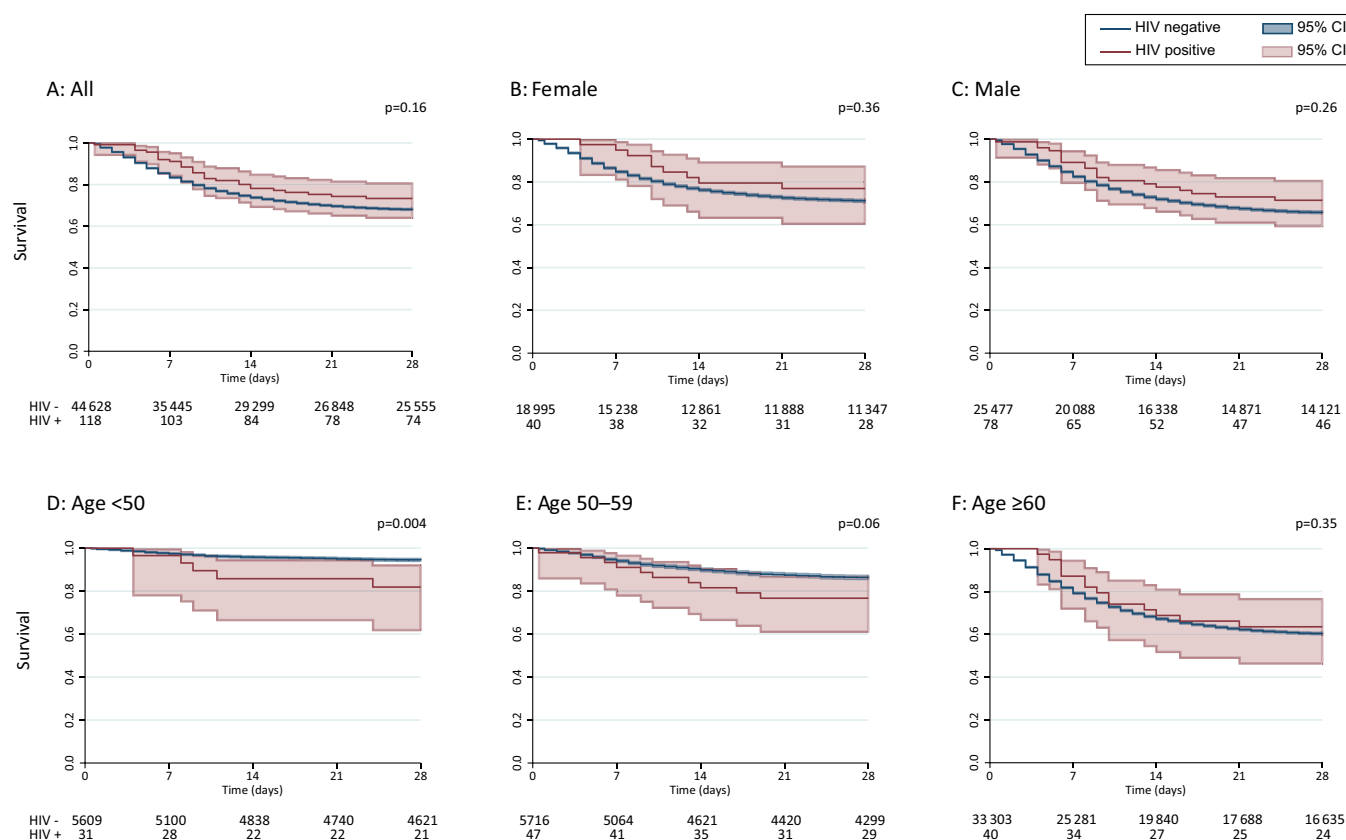
Figure 3. Kaplan-Meier survival plots stratified by HIV status. (A) All, (B) female, (C) male, (D) <50 years, (E) 50–59 years, (F) ≥60 years. P values are log-rank tests. Abbreviation: HIV, human immunodeficiency virus.
