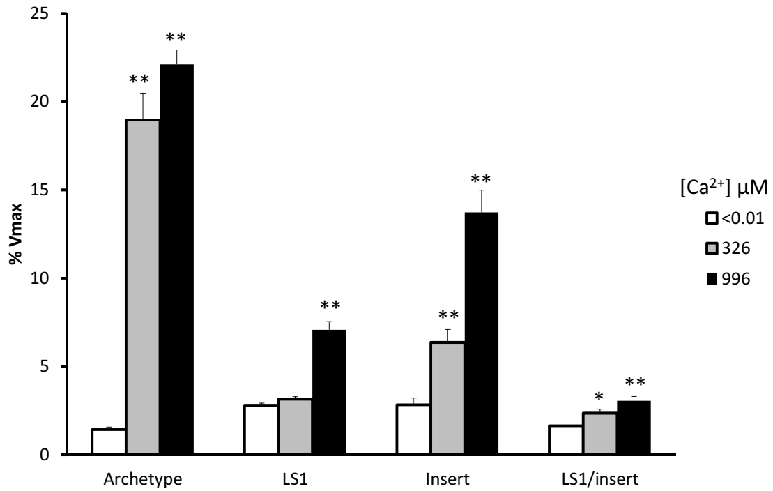
Figure 3 Effects of Ca 2+ on the activity of human OGDH E1 splice variants.
