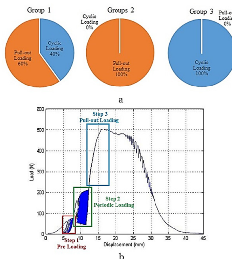
Figure 4. (a) loading step that samples reached the failure in Groups 1, 2 and 3; (b) Three loading steps load-displacement result of the fifth sample in Group 2.
