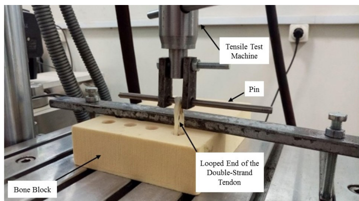
Figure 3. Testing a typical sample using BASHTI technique. It was assumed that when the tendon displacement became more than 10 mm, the failure mode occurs on the fixation site.
