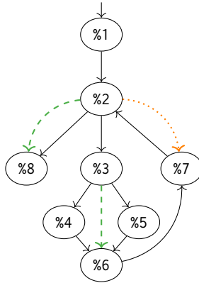
(d) The same CFG with explicit edges for merge (→) and continue (→) targets
