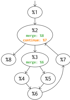
(c) Its CFG, with loop/selection headers annotated with merge/continue targets
