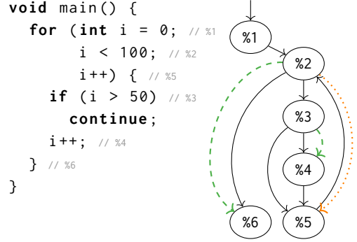
Fig. 4. A loop with an early continue
