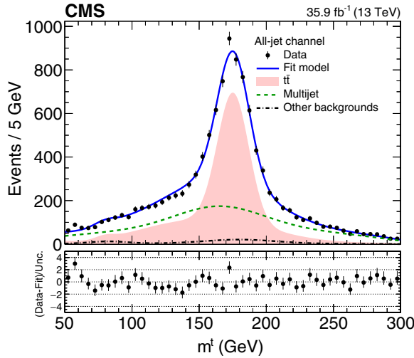
FIG. 1. Result of the fit of m_{\text{SD}} of the t jet candidate, m' , in the signal region \text{SR}_A to data in the all-jet events. The shaded area shows the t\bar{t} contribution, the dashed line shows the multijet background, and the dot-dashed line shows the other subdominant backgrounds. The solid line is the fit to the combined signal + background model, and the data points are represented by the filled circles. The lower panel shows the difference between the data and the fit model, divided by the uncertainty in the fit.
