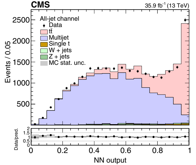
FIG. 2. Comparison between data and prediction in the signal region \text{SR}_B (same as the \text{SR} , but without an NN requirement) of the NN output distribution for the all-jet channel. The contributions from t\bar{t} and multijet production are normalized according to the fitted values of their respective yields and shown as stacked histograms. The data points are represented by filled circles, while the shaded band represents the statistical uncertainty in simulation. The lower panel shows the data divided by the sum of the predictions.
