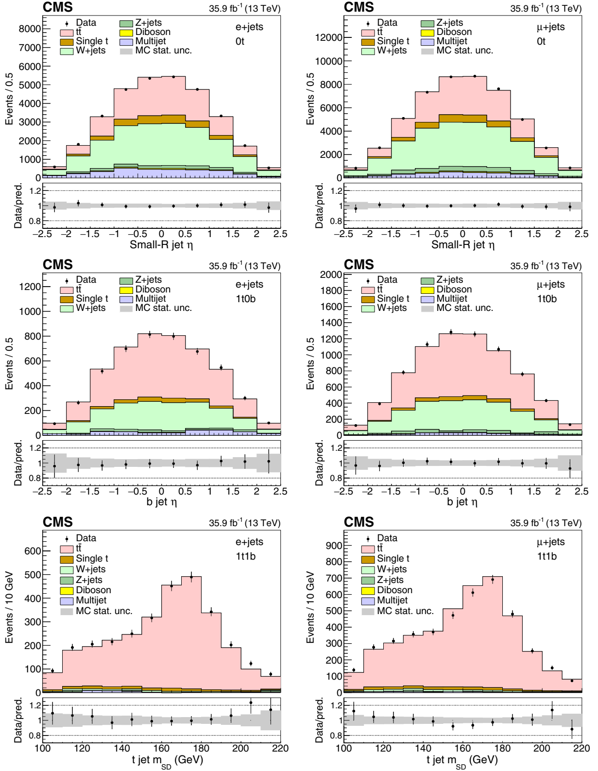
FIG. 6. Posterior kinematic distributions in the maximum-likelihood fit. Different event categories and variables are fitted: \eta distribution for small-R jets in Ot events (upper row), \eta distribution of the b jet candidate in 1t0b events (middle row), and m_{SD} of the t jet candidate in 1t1b events (lower row), in the e + \text{jets} (left column) and \mu + \text{jets} (right column) channels. The data points are indicated by filled circles, while the signal and background predictions are shown as stacked histograms. The lower panels show data divided by the sum of the predictions and their systematic uncertainties as obtained from the fit (shaded band).
