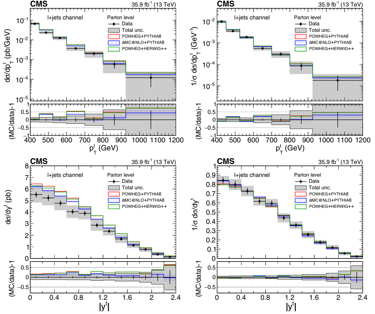
FIG. 20. Differential cross section measurements at the parton level, as a function of the parton-level top quark p_T (upper row) and |y| (lower row) for the \ell + \text{jets} channel. Both absolute (left column) and normalized (right column) cross sections are shown. The lower panel shows the ratio (\text{MC}/\text{data}) - 1 . The vertical bars on the data and in the ratio represent the statistical uncertainty in data, while the shaded band shows the total statistical and systematic uncertainty added in quadrature. The hatched bands show the statistical uncertainty of the MC samples.
