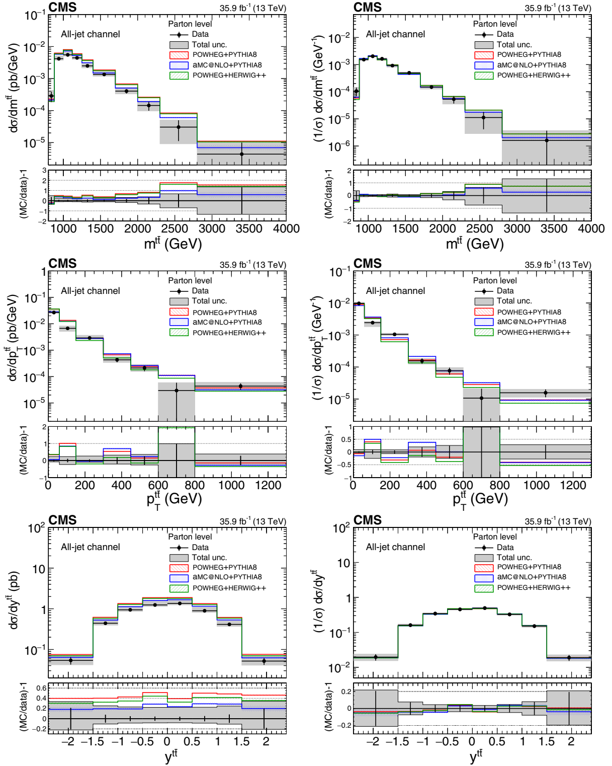
FIG. 16. Differential cross section unfolded to the parton level, absolute (left) and normalized (right), as a function of m^{t\bar{t}} (upper row), p_T^{t\bar{t}} (middle row), and y^{t\bar{t}} (lower row) in the all-jet channel. The lower panel shows the ratio (MC/data) - 1 . The vertical bars on the data and in the ratio represent the statistical uncertainty in data, while the shaded band shows the total statistical and systematic uncertainty added in quadrature. The hatched bands show the statistical uncertainty of the MC samples.
