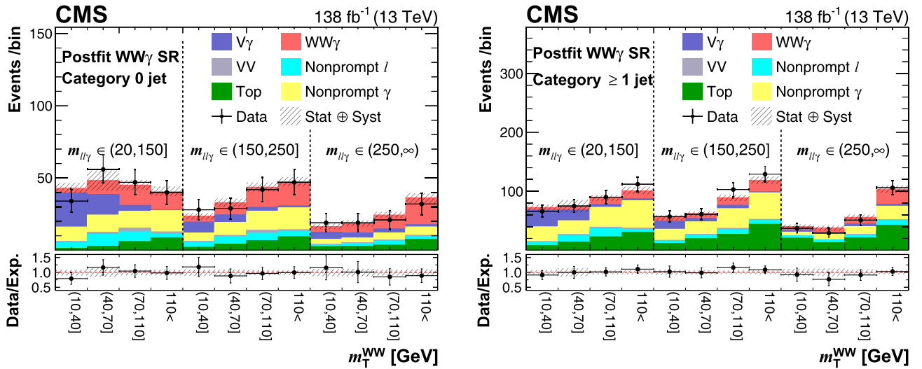
FIG. 3. The unrolled two-dimensional m_T^{\text{WW}} - m_{\ell\ell\gamma} distributions in category 0 jet (left) and \geq 1 jet (right) after the fit to data. The data are compared with the sum of the signal and expected background. The black points with error bars represent the data and their statistical uncertainties, whereas the hatched bands represent the total uncertainties in the predictions.
