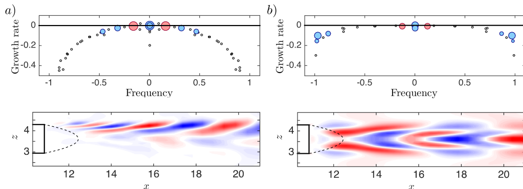
FIGURE 10. DMD results for (a) the unforced flow and (b) the flow with feedback control. The top figure shows the frequencies and growth rates of the DMD modes scaled by their optimum amplitudes; the bottom figure is a top-view of the spatial structure of the most dynamically represented modes (red markers on the frequency vs. growth rate figure) at (a) St = 0.16 for unforced flow and (b) St = 0.13 for the flow with feedback control.
