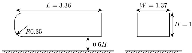
FIGURE 1. Schematic of square-back Ahmed body: (a) side view ; (b) rear view.
