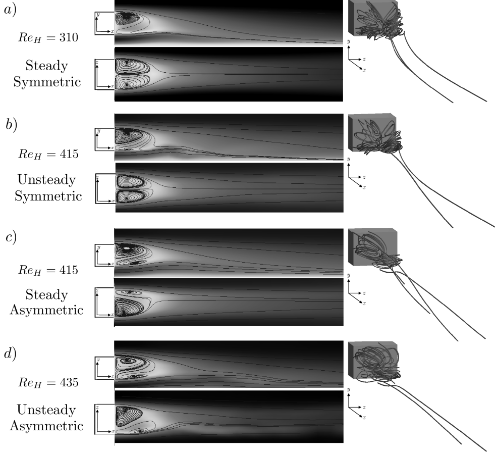
FIGURE 3. Visualisations of Ahmed Body flow at Reynolds numbers (a) Re_H = 310 , (b) and (c) Re_H = 415 , (d) Re_H = 435 . For each Re_H the top and bottom left pictures show side view and top view respectively of a 2D slice with streamlines projected onto it; the right picture shows 3D streamlines in the wake.
