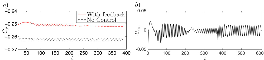
FIGURE 8. a) Comparison of converged base pressure coefficient, C_p , with (red) and without (black) feedback control. b) Corresponding actuation signal, U_{jet}
