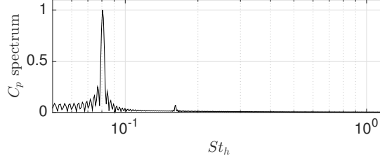
FIGURE 6. Amplitude of base pressure force spectrum for the Ahmed body flow at Re_H = 435 .
