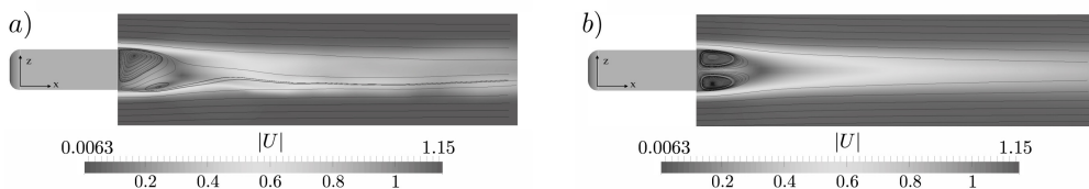
FIGURE 9. 2D slice of a) unforced and b) controlled instantaneous flow fields coloured by magnitude of the velocity with streamlines projected onto the 'top-view' slices.
