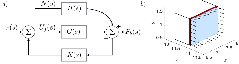
FIGURE 5. a) Dynamically linear model for feedback control: s denotes Laplace transform variable. b) Schematic of the control arrangement: sensor (light blue) measures the base pressure force and actuation (red) acts via synthetic jets angled at 10^\circ outwards from the downstream direction.
