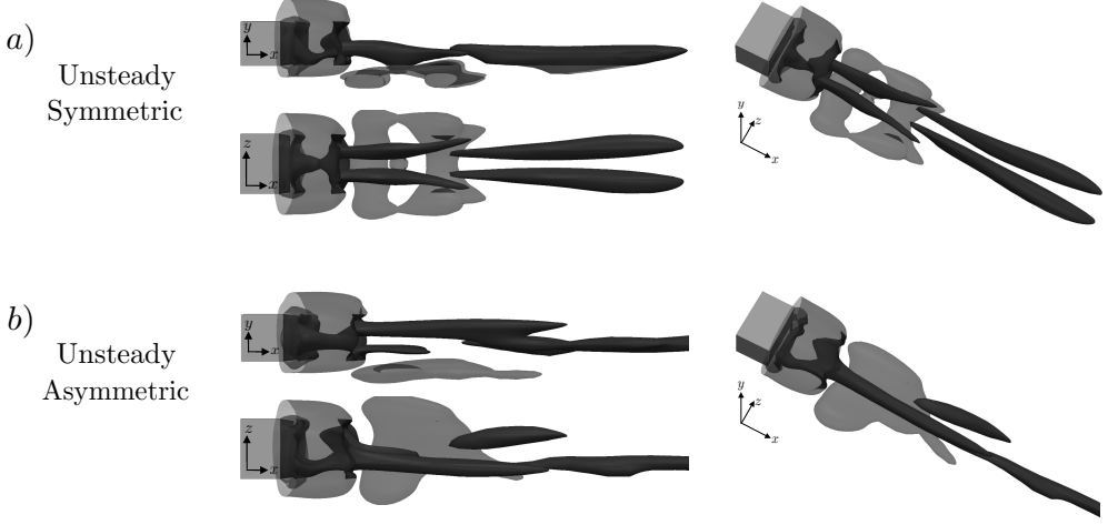
FIGURE 4. Q-criterion iso-contour of Ahmed Body flow at Reynolds number Re_H = 435 when the wake is (a) unsteady symmetric, (b) unsteady asymmetric. For each regime, the top and bottom left pictures show side view and top view respectively; the right picture shows the diagonal view from the top. The same Q-criterion iso-contour is plotted with opaque and transparent parts to reveal the internal structure of the vortex ring in the wake.
