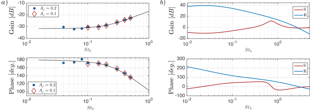
FIGURE 7. Frequency response gain and phase for (left) system identification data from open-loop simulations at A_j = 0.1 and A_j = 0.2 and (right) for the controller K(s) and sensitivity function S(s)
