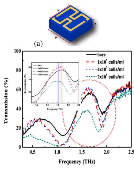
Fig. 5: (a) Unit cell of an EIT-like THz metamaterial for detection of oral cancer [55]; (b) related transmission spectra of the metamaterial under different oral cancer cells concentrations
