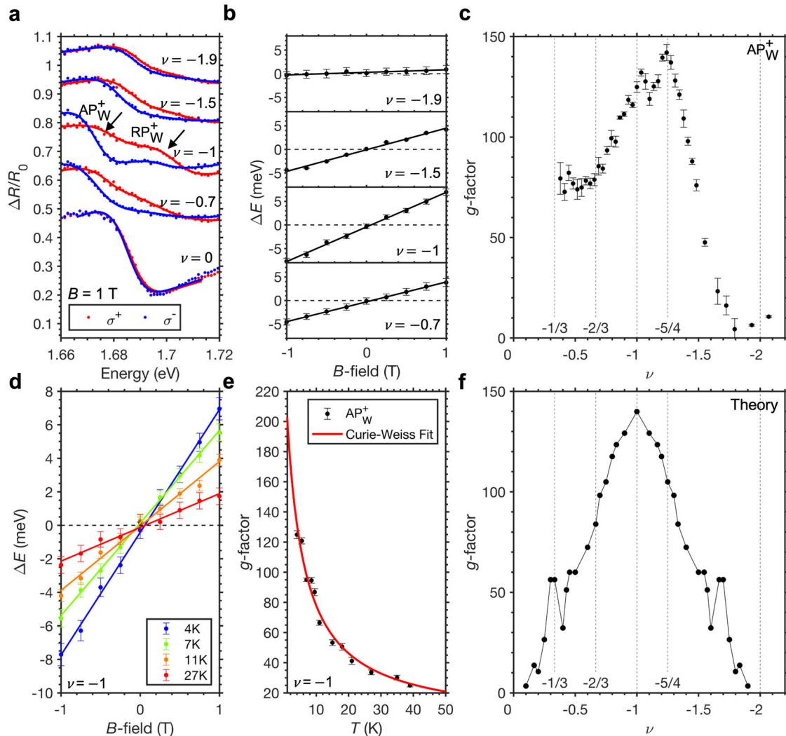
Fig. 4 Exciton-polaron magnetic interactions at different hole fractional fillings. a \sigma^- (blue) and \sigma^+ -resolved (red) \Delta R/R_0 spectra at representative hole \nu values under a B = 1 T. b B -field-dependent Zeeman splitting of \text{AP}_W^+ from -1 to 1 T at representative hole \nu values. c Evolution of the g -factor of \text{AP}_W^+ as a function of the hole \nu extracted from linear fits of \Delta E in the range |B| \leq 1 T (solid lines in panel b ). d Valley Zeeman splitting of the \text{AP}_W^+ resonance at \nu = -1 for different temperatures. e Evolution of the measured g -factor of \text{AP}_W^+ as a function of temperature for \nu = -1 in the temperature range for which the oscillator strength and linewidth of \text{AP}_W^+ are sufficient to enable a reliable estimate of the Zeeman splitting. The red solid line represents a fit of the experimental data (black dots) to a Curie–Weiss law from which the Weiss constant is estimated to be \theta = -4.6 \pm 0.9 K. The negative sign of the extracted Weiss constant reveals antiferromagnetic ordering of neighbouring hole spins. f Theoretical prediction of the \nu dependence of the g -factor based on a model that solves the Heisenberg Hamiltonian for charge-ordered hole states with antiferromagnetic exchange interactions between nearest neighbour spins. For all panels the error bars represent 68% confidence intervals.
