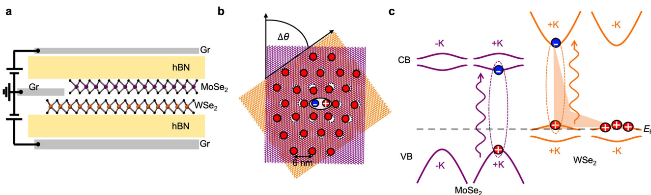
Fig. 1 Device structure. a Sketch of the dual-gated \text{WSe}_2/\text{MoSe}_2 hetero-bilayer. Graphene layers are used as top, bottom, and hetero-bilayer electrical contacts, while 18-nm-thick hBN layers are used as dielectric spacers 34 . b Illustration of the top view of a moiré superlattice with a twist angle \Delta\theta and fractional filling of one hole per moiré unit cell. Fermi-polarons form between the photo-excited electron-hole pair and charge-ordered Fermi sea. c Schematic type-II band structure of the \text{H-WSe}_2/\text{MoSe}_2 hetero-bilayer. Purple and orange curves denote bands from \text{MoSe}_2 and \text{WSe}_2 , respectively. The vertical wavy arrows represent the photon absorption by intralayer excitons in each monolayer. When the Fermi level ( E_F ) is tuned into the top valence band, the \text{WSe}_2 attractive polaron forms due to interactions between the exciton in one valley, dressed by holes in the opposite valley.
