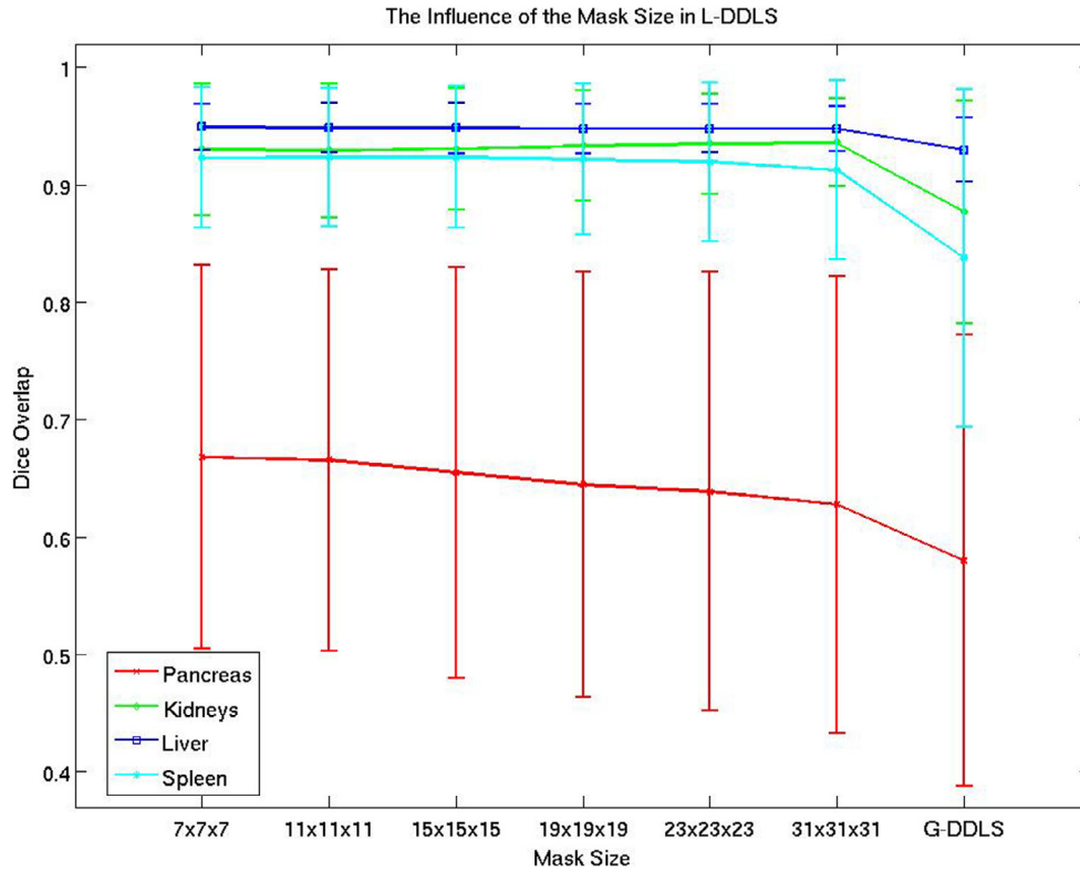
Fig. 6. Influence of the mask size on the segmentation accuracy of L-DDLS. The results were obtained by selecting the 5 most similar atlases in a leave-one-out procedure. G-DDLS is an extreme case of L-DDLS by increasing the mask size to the image size.
