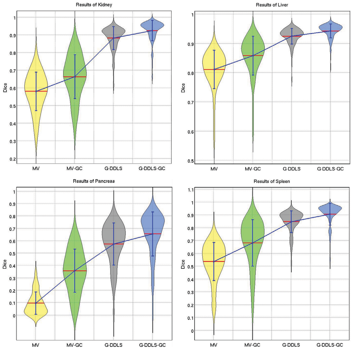
Fig. 4. Comparison of different approaches. The global atlas selection strategy was utilized and 20 atlases were selected for the segmentation of each target image.
