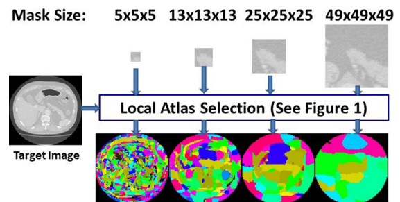
Fig. 2. Example demonstrating the local atlas selection for different local mask sizes. The color maps show the most similar atlas selected at different locations in the target image. Different colors mean that different atlases are selected at different locations. (For interpretation of the references to color in this figure legend, the reader is referred to the web version of this article.)
