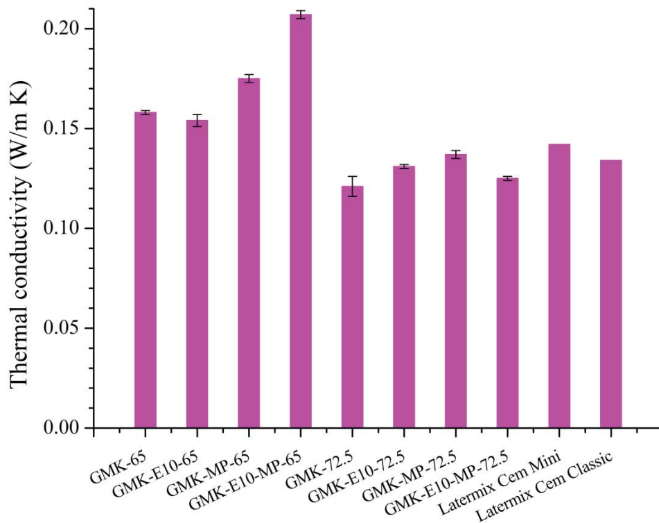
Fig. 5. Thermal conductivity of LWGC samples. Data for two commercial products (Laternix Cem Mini© and Laternix Cem Classic©), are also reported for comparison. [67]
