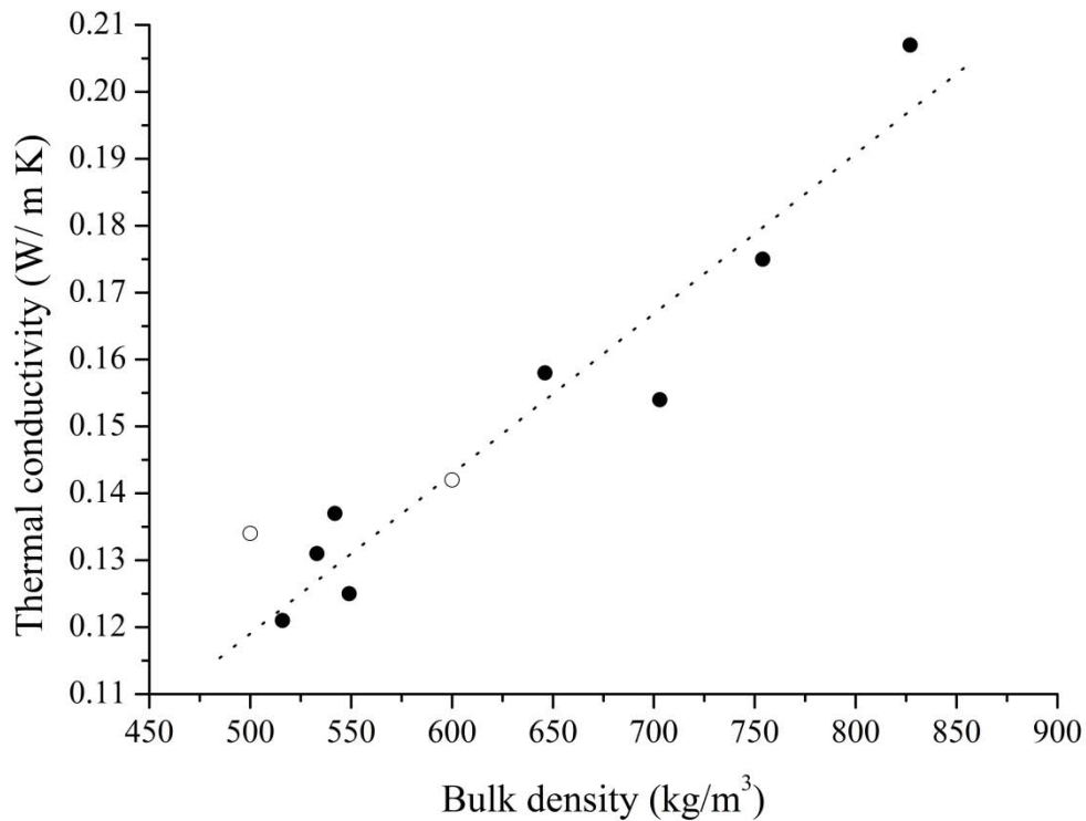
Fig. 6. Correlation between thermal conductivity and density of LWGC samples: full circles (●) are related to LWGC samples; empty circles (○) are related to two commercial products (Latermix Cem Mini© and Latermix Cem Classic©, [67]).
