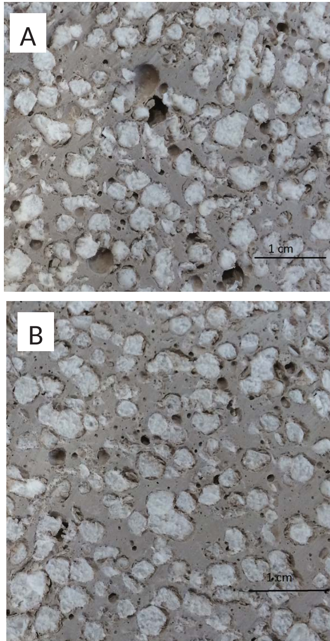
Fig. 2. Optical micrograph of polished surfaces of A) GMK-72.5 and B) GMK-E10-72.5.
