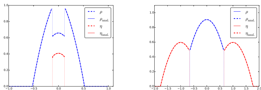
(a) Attractive-attractive cross interaction.
