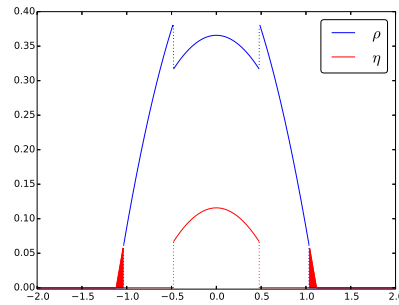
FIG. 4. For \epsilon > \epsilon^{(1)} a second kind of profile surfaces. In fact, there is a whole family of steady states parameterized by the mass fraction, p \in [p_{\min}, p_{\max}] , in the corners (filled in red).
