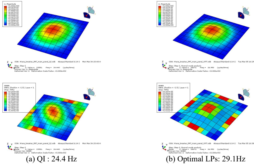
(a) QI : 24.4 Hz (b) Optimal LPs: 29.1Hz Figure 6 Fundamental vibration mode shapes (top) and modal strain energy density distribution (bottom) of the optimised laminated composite main panel
