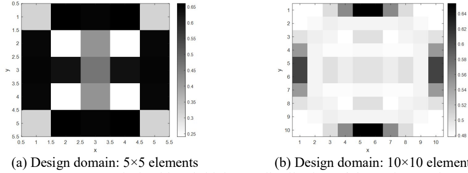
Figure 7 Optimised local thickness distribution of the main panel with 50% weight saving
