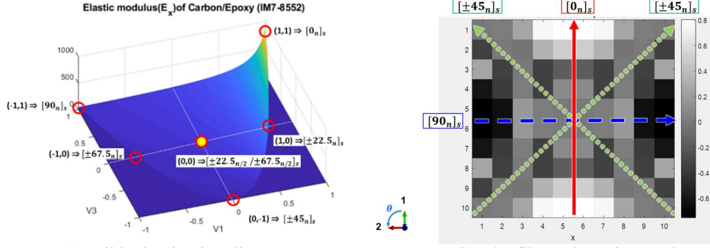
(a) Miki's lamination diagram (b) The fibre orientation angles of the optimised laminated composite main panel Figure 5 Miki's lamination diagram and the fibre orientation angles of the optimised laminated composite main panel
