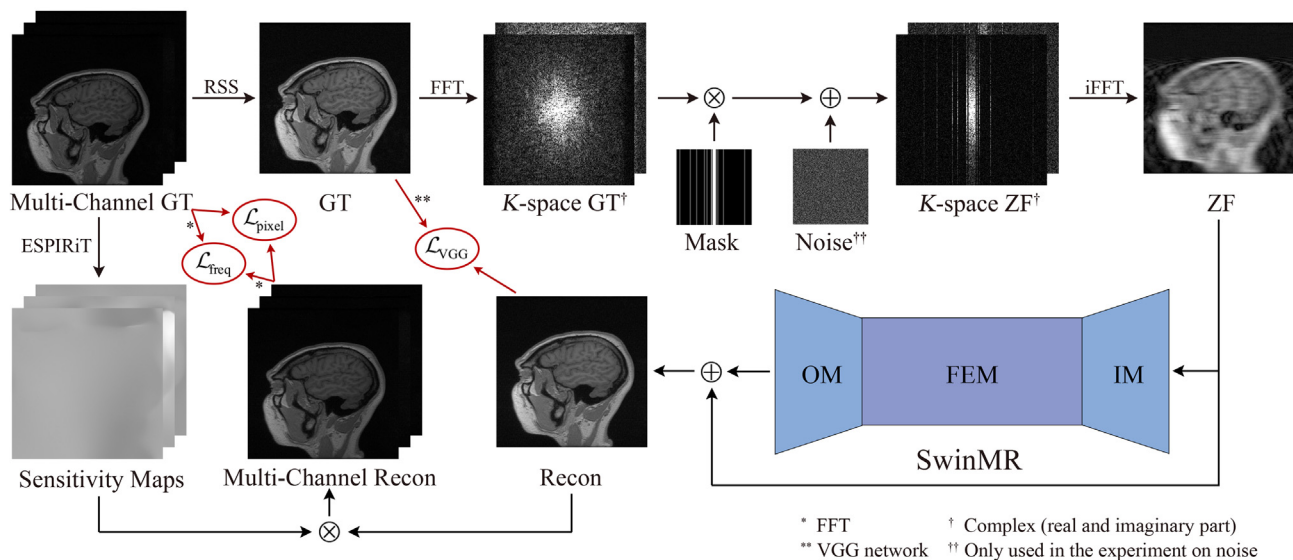
Fig. 2. The dataflow of proposed SwinMR. Root sum square (RSS) is applied to combine the multi-channel ground truth MR images (Multi-Channel GT) to single-channel ground truth MR images (GT). Undersampling and noise interruption are performed in k -space using fast Fourier transform (FFT) and inverse fast Fourier transform (iFFT) to convert the GT to undersampled zero-filled MR images (ZF) as the input of our proposed SwinMR. Multi-channel reconstructed MR images (Multi-Channel Recon) are calculated by the pixel-wise multiplication of single-channel reconstructed MR images (Recon), which are the output of the proposed SwinMR, and sensitivity maps, which are estimated by ESPIRiT from the Multi-Channel GT.
