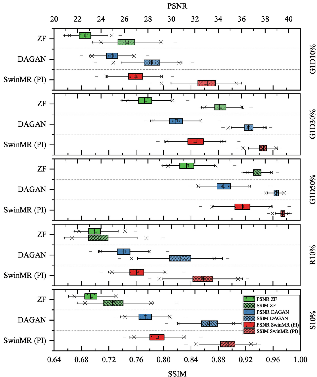
Fig. 5. Peak signal-to-noise ratio (PSNR) and Structural similarity index (SSIM) of the experiment on different masks. Five undersampling trajectories including Gaussian 1D 10% (G1D10%), Gaussian 1D 30% (G1D30%), Gaussian 1D 50% (G1D50%), radial 10% (R10%) and spiral 10% (S10%) were applied in this experiment. (Box range: interquartile range; x: 1% and 99% confidence interval; —: maximum and minimum; □: mean; |: median.) The SwinMR (PI) outperforms the DAGAN using different undersampling masks with significantly higher PSNR, SSIM ( p < 0.05 by paired t-Test).
