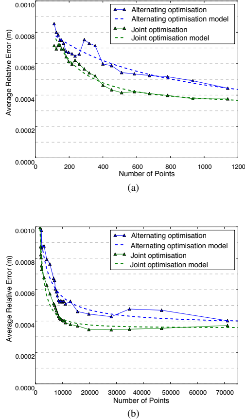
Fig. 2: Average relative error against number of points. The raw results from our experiments (solid lines) are shown together with fitted curves (dotted lines). We observe that the joint optimisation method decreases rapidly in both cases, but as more data are used in the optimisations, the alternating method slowly catches on. In (a) we observe a curve similar to [14] for the joint optimisation. The alternating optimisation error decreases at a slower rate, but we can see that the difference gets smaller with more data. In (b) the error rapidly decreases for both methods till around 15,000–20,000 points. We again observe a slightly steeper decrease for jointly-optimised minimisation compared to alternating optimisation, but this difference decreases with more data.
