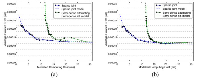
Fig. 5: Average relative rotation error against modelled computational cost when the algorithms are initialised using (a) LSD-SLAM[21] or (b) ground truth. The shape of these plots are almost identical to those for translation error.
