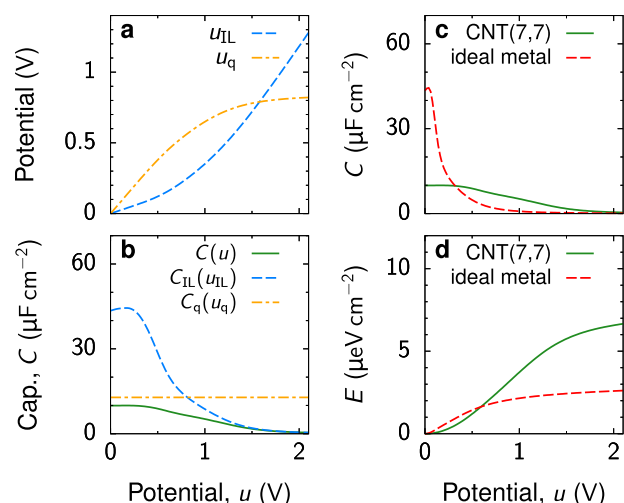
Figure 2. Charge storage in electrolyte-filled metallic CNTs. (a) Potentials u_{IL} and u_q = u - u_{IL} (see Figure 1a) as functions of voltage u applied to a (7,7) CNT with respect to the bulk electrolyte. (b) Quantum ( C_q ) and electrical double-layer ( C_{IL} ) capacitances evaluated at u_q and u_{IL} , respectively, showing that the total capacitance C is smaller than C_q and C_{IL} ; C is determined by eq 2. (c) Comparison of the capacitance of a (7,7) CNT and of a nanotube of the same radius as a (7,7) CNT but with perfectly metallic walls. (d) Energy stored in a (7,7) CNT and in the metallic nanotube of the same radius. Although the CNT stores slightly less energy at low voltages, it provides a few times higher stored energy densities at moderate and high voltages. In all plots, the ion radius a = 0.25 nm, the tube radius R = 0.47 nm, the in-pore dielectric constant \epsilon = 5 , and T = 300 K. The ion chemical potential \mu of -0.1 eV corresponds to a moderately ionophilic pore (inset of Figure 1c and Figure S1). For a comparison with ionophobic and strongly ionophilic pores, see Figure S3.
