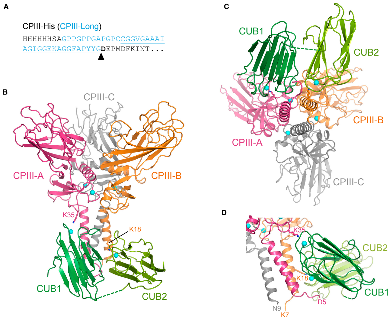
Figure 1. Overall Structure of the CPIII:C1C2 Complex
