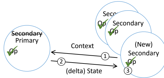
Figure 6.2: A diagram showing state copying in Fabric.
