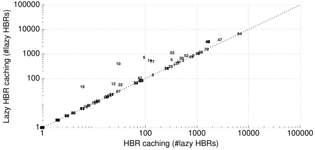
Figure 4.5: The number of terminal lazy HBRs explored by the first 100,000 terminal schedules of lazy HBR caching and HBR caching.
