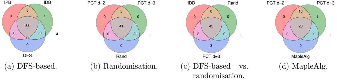
Figure 3.3: Venn diagrams showing number of benchmarks in which the bugs were found with the various techniques.
