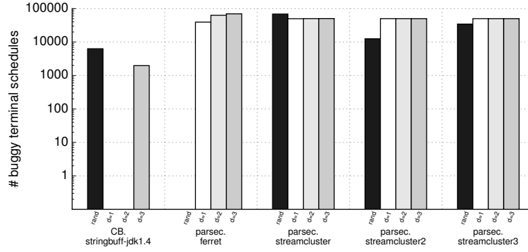
Figure 3.8: Shows, for the stringbuff-jdk1.4 and parsec benchmarks, the number of buggy schedules explored by Rand, and PCT for each value of d \in \{1, 2, 3\} . Each technique explored 100,000 schedules.
