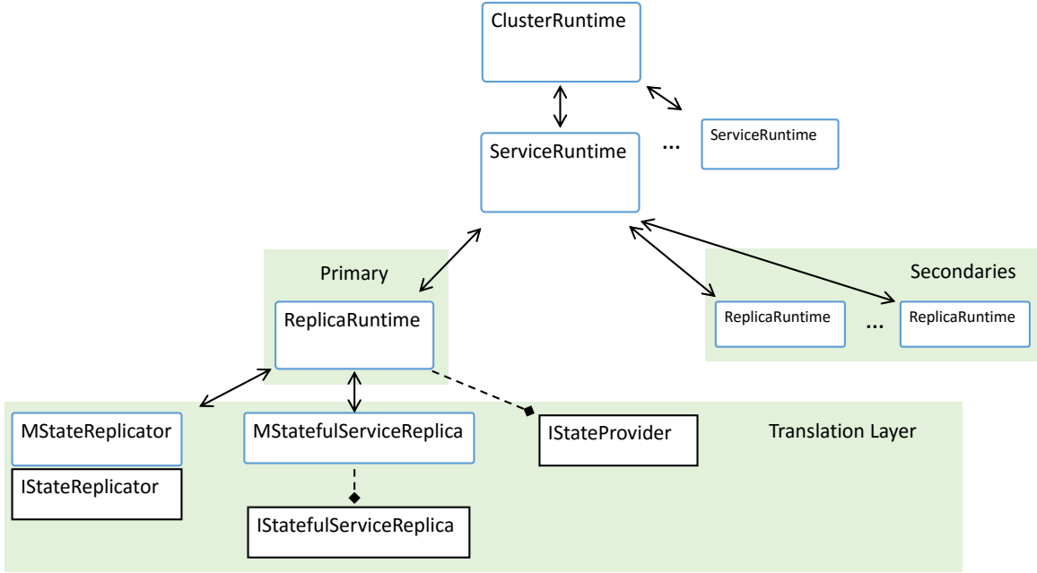
Figure 6.5: A diagram showing the design of the P# Fabric model. The rounded rectangles with a blue outline represent P# actors, while the rectangles with a black outline are C# classes that implement the interface given by the associated label. The solid lines indicate communication via messages. The dashed lines show composition, e.g. a ReplicaRuntime actor invokes methods on its IStateProvider object. Note that an MStateReplicator actor and its IStateReplicator object interact via shared-memory communication.
