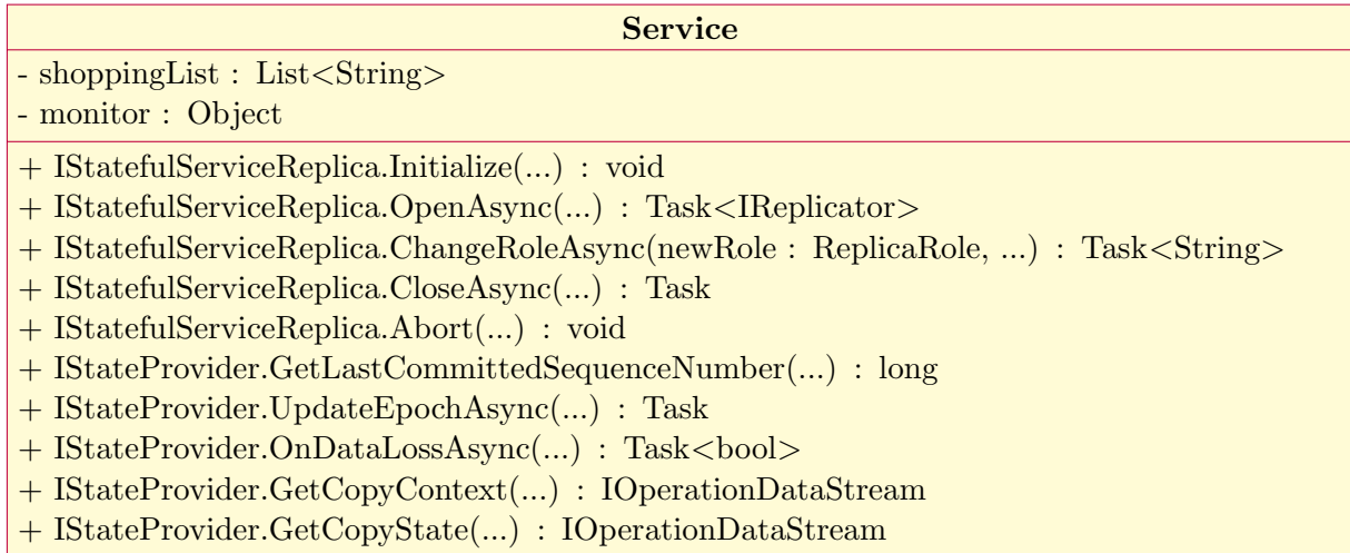
Figure 6.3: A class diagram of our C# Fabric shopping list service class. Many fields and methods are omitted so as to focus only on the key details. We use “...” to indicate omitted method parameters
