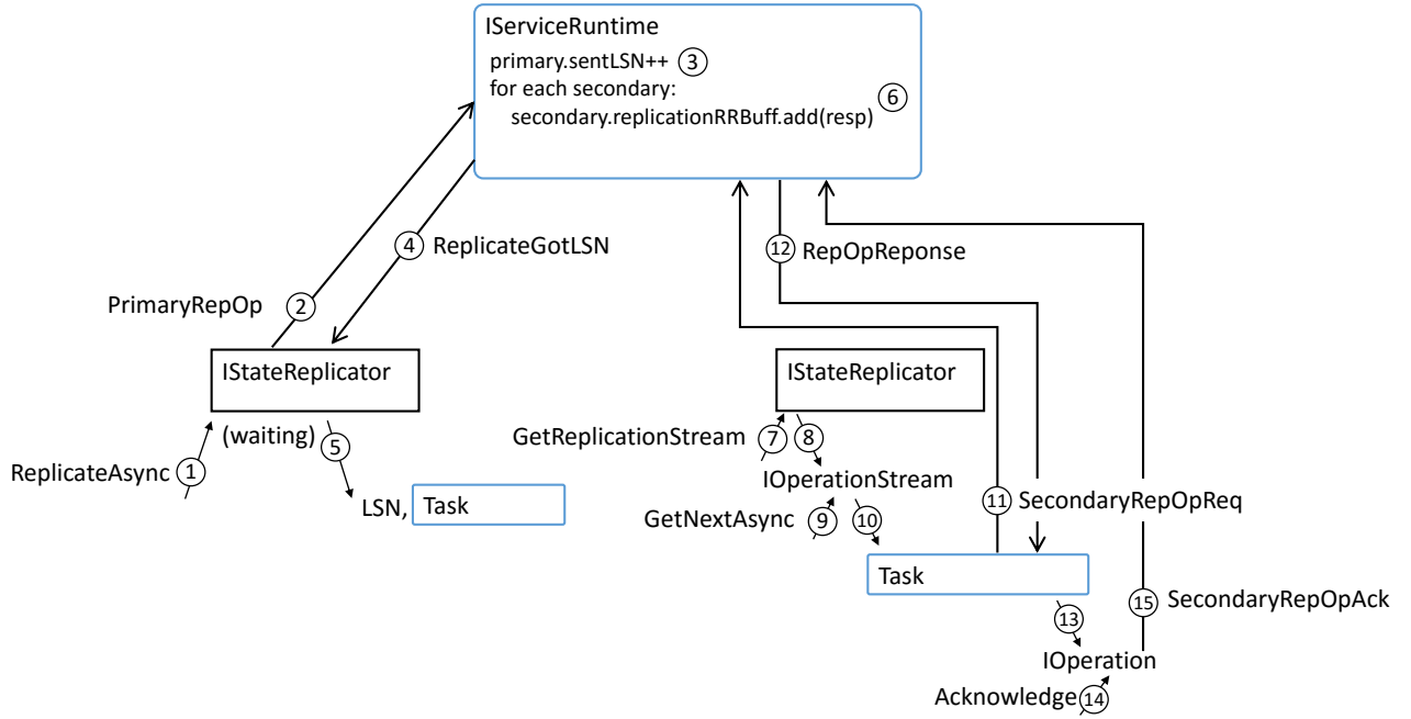
Figure 6.11: A diagram showing stage one and two of replication in version 2 of our Fabric model. The left IStateReplicator is the primary replica.
