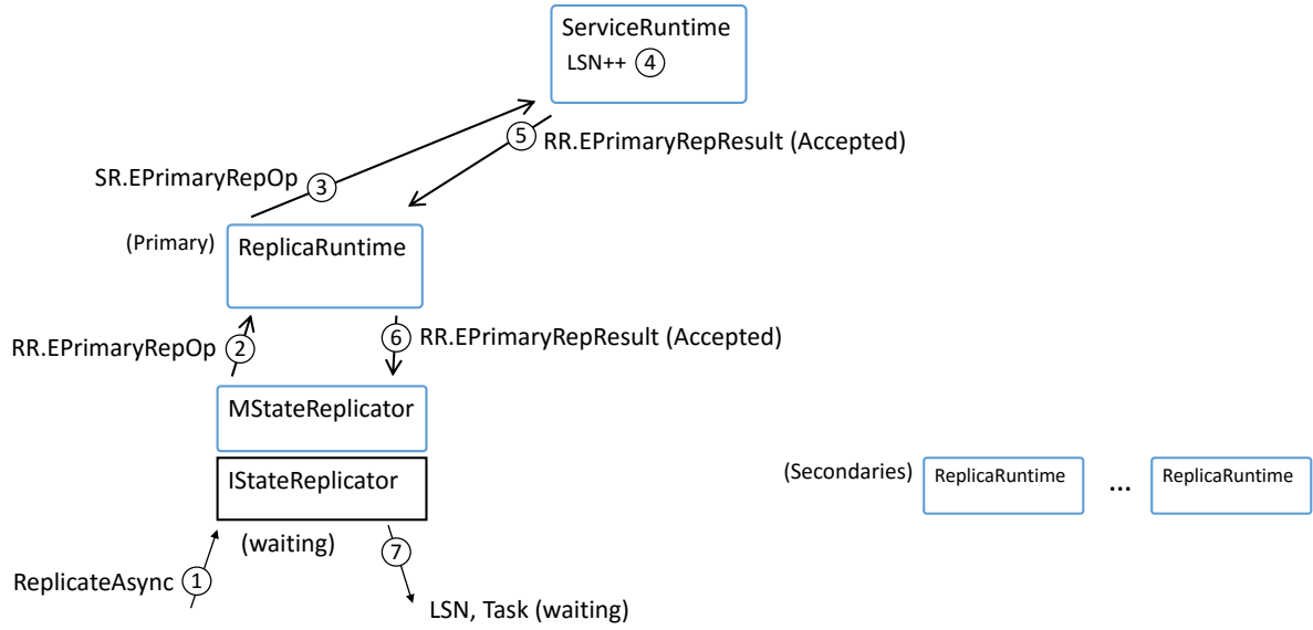
Figure 6.6: A diagram showing the first stage of replication in our Fabric model. The left ReplicaRuntime is the primary replica.
