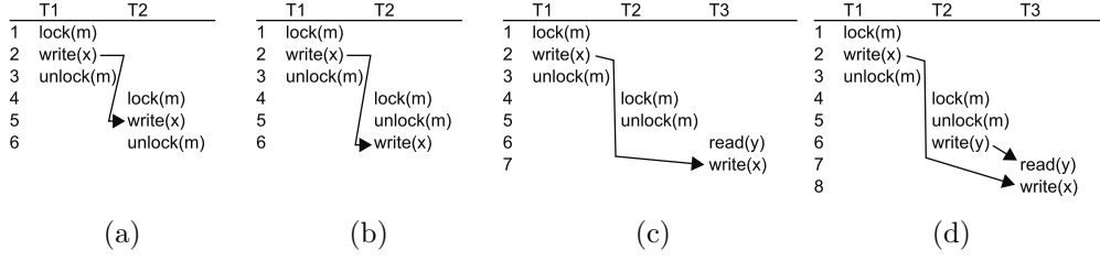
Figure 4.2: Four (unrelated) terminal schedules that we considered when designing lazy DPOR. The arrows indicate the lazy races.
