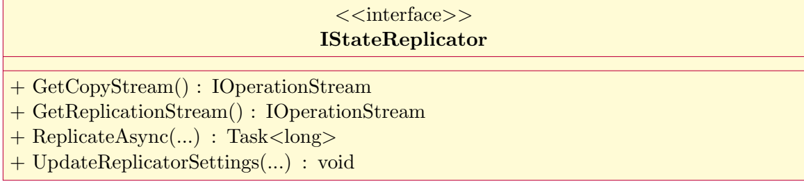
Figure 6.4: A class diagram of Fabric’s IStateReplicator interface.
