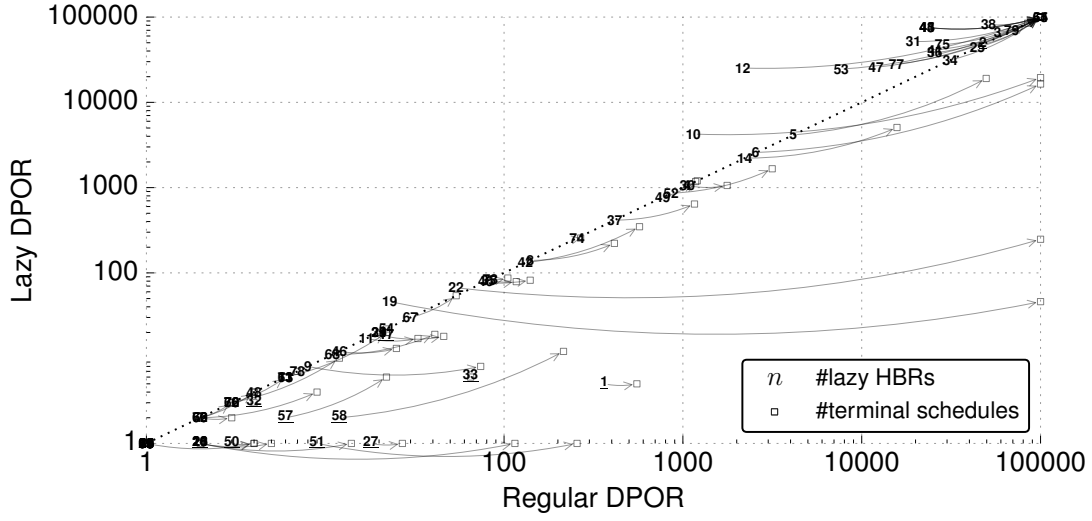
Figure 4.6: Number of terminal lazy HBRs (id) and terminal schedules (square) explored for each benchmark by the first 100,000 terminal schedules of regular and lazy DPOR.
