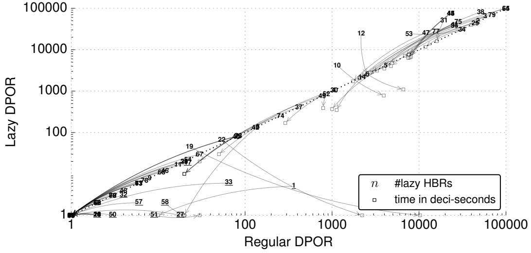
Figure 4.7: Number of lazy HBRs (id) explored and deci-seconds taken (square) for each benchmark with regular and lazy DPOR.
