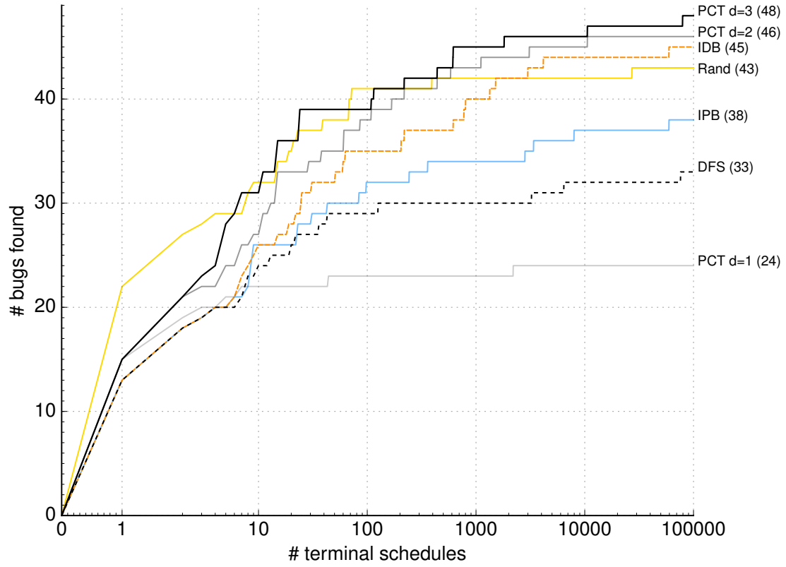
Figure 3.4: Cumulative plot, showing, for each SCT technique, the number of bugs found after x schedules over all the benchmarks. The plot is intended to be viewed in colour.
