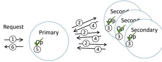
Figure 6.1: A diagram showing replication in Fabric.
