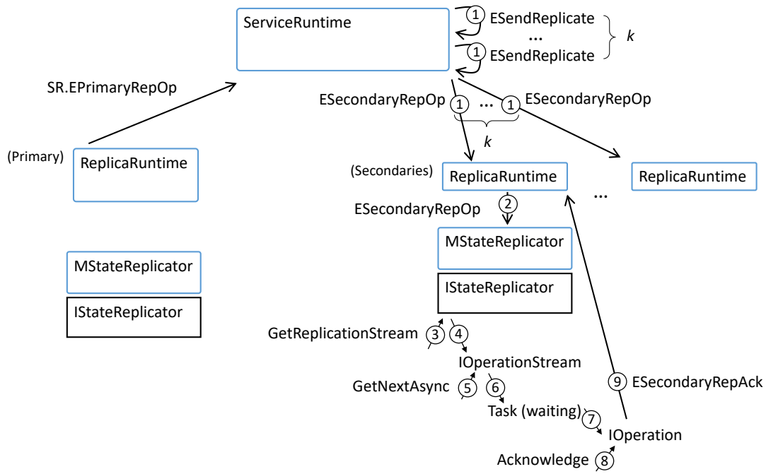
Figure 6.7: A diagram showing the second stage of replication in our Fabric model.
