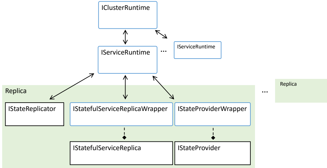
Figure 6.10: A diagram showing the design of our Fabric model V2. The rounded rectangles with a blue outline represent actors, while the rectangles with a black outline are C# objects that implement the interface given by the associated label. The solid lines indicate communication via messages. The dashed lines show composition (e.g. the IStateProviderWrapper actor invokes methods on its IStateProvider object).
