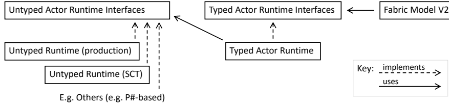
Figure 6.9: The assembly dependency diagram for our Adara actors framework and our Fabric model V2.
