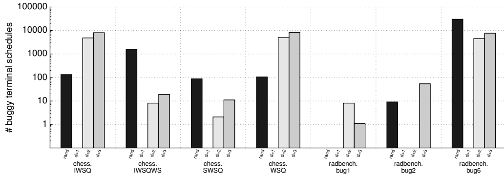
Figure 3.9: Shows, for the chess and radbench benchmarks, the number of buggy schedules explored by Rand, and PCT for each value of d \in \{1, 2, 3\} . Each technique explored 100,000 schedules (except for chess.IWSQWS and chess.SWSQ , which use a schedule limit of 10,000).
