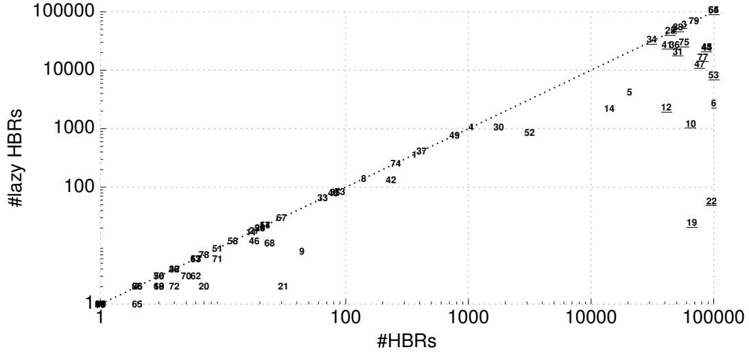
Figure 4.4: The number of terminal HBRs and terminal lazy HBRs explored by the first 100,000 terminal schedules of DPOR.
