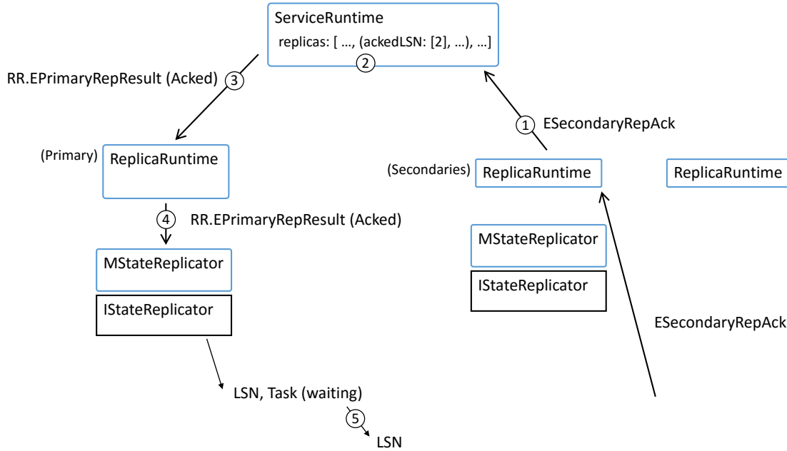
Figure 6.8: A diagram showing the third stage of replication in our Fabric model.
