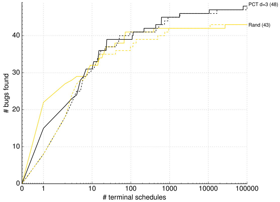
Figure 3.5: For PCT d=3 and Rand, compares the number of bugs found after x schedules as in Figure 3.4 (solid lines) with the average behaviour of the techniques (dashed lines). The plot is intended to be viewed in colour.
