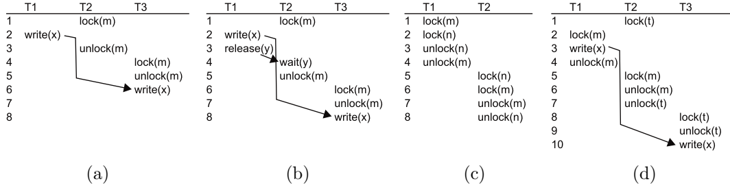
Figure 4.3: Several terminal schedules that demonstrate potential issues for lazy DPOR. The arrows indicate the lazy races.
