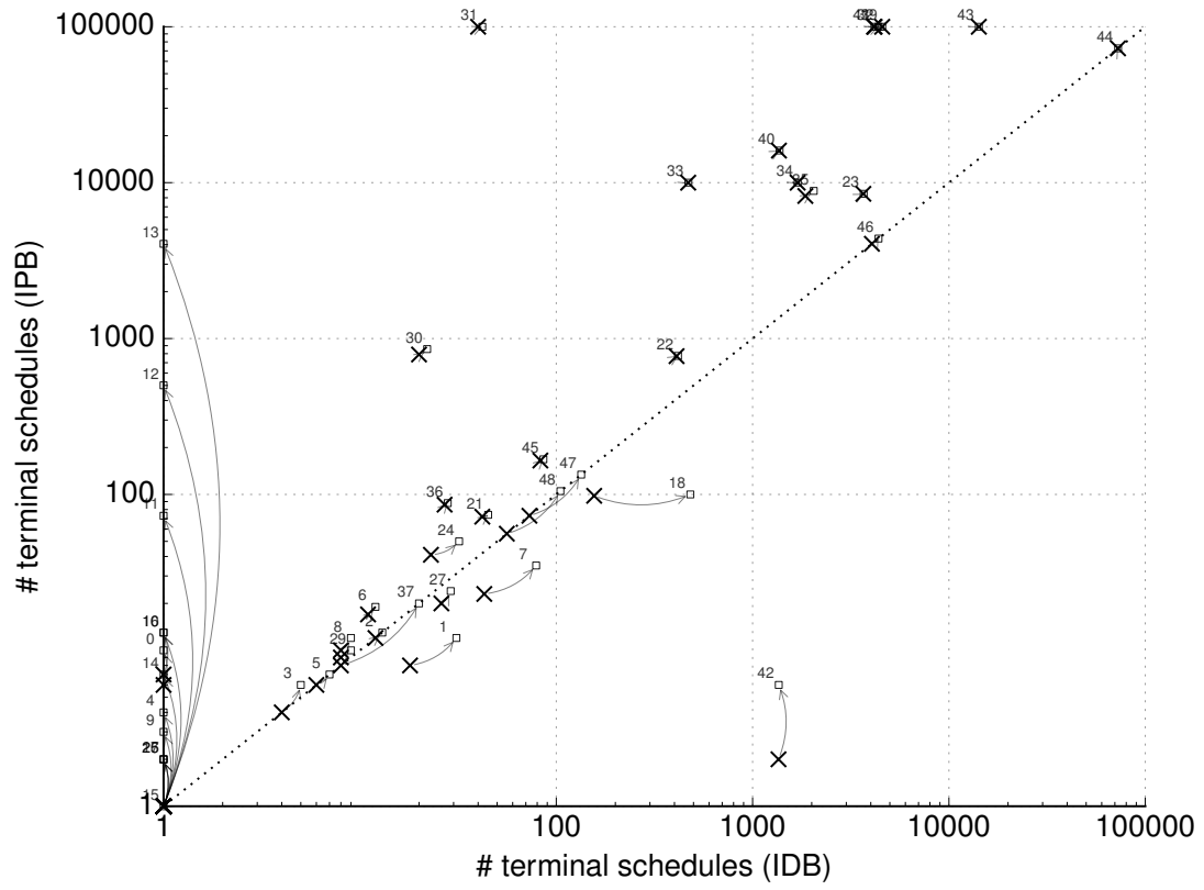
Figure 3.7: Comparison of IPB and IDB, showing total number of non-buggy schedules (cross) connected to the total number of schedules (square), up to the bound that found the bug. Squares are labelled with the benchmark id.
