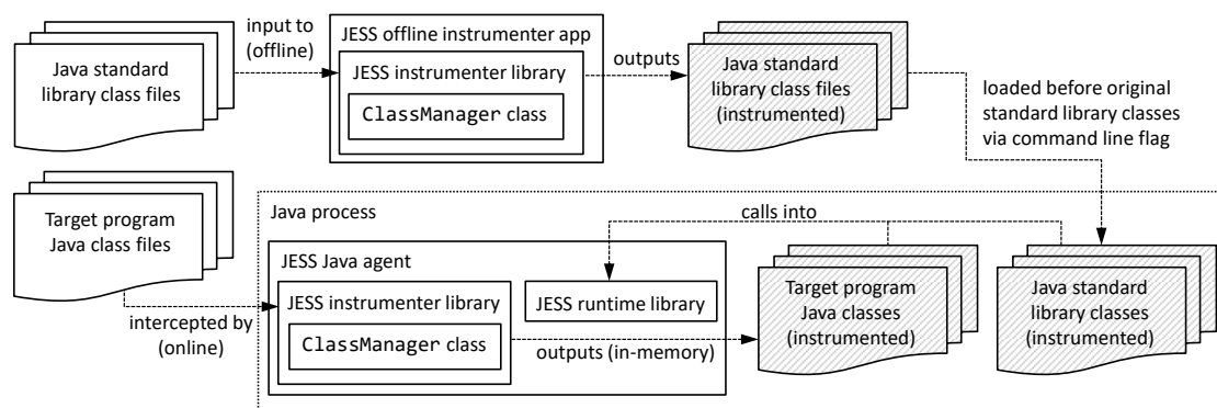
Figure 5.1: A diagram showing how our JESS tool instruments code offline and at run-time. The Java standard library class files are instrumented offline and then loaded via a command line flag. The target program class files are instrumented online (i.e. at run-time). The instrumented code calls into the JESS runtime library so that thread execution is controlled.
