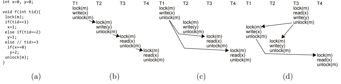
Figure 4.1: A simple multithreaded program (a), and several schedules (b-d). The arrows indicate the HBR; (b) uses the traditional HBR while (c) and (d) use a representation of our lazy HBR.
