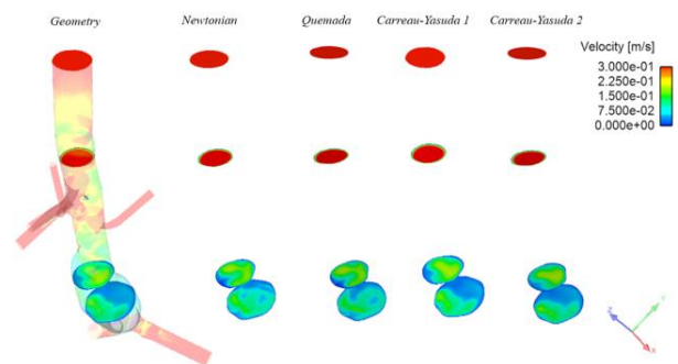
Figure 12 Geometry (left) & Velocity contours of the inlet, planes 1, 2, 3 (top to bottom) of Newtonian model (2 nd left), Quemada model (3 rd left), Carreau-Yasuda 1 model (4 th left), Carreau-Yasuda 2 model (right)
