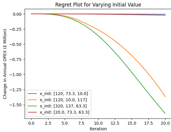
Figure 9: Annual Operational Expenditure (OPEX) convergence plot for Extremum Seeking Control given different initial values
