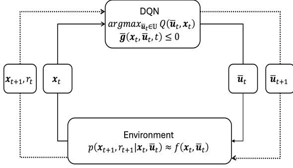
Figure 3: DQN process scheme
