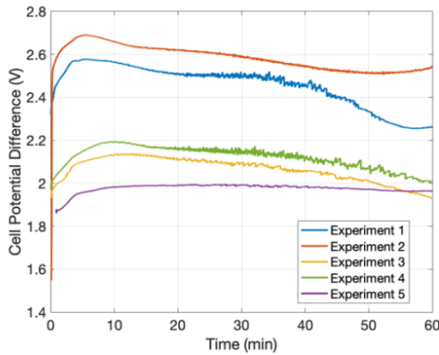
Figure 3. Cell potential difference of all experiments during the first hour electrolysis
