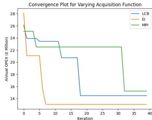
Figure 4: Annual Operational Expenditure (OPEX) convergence plot for Bayesian optimisation given different acquisition functions: Lower Confidence Bound (LCB), Expected Improvement (EI) and Maximum Probability of Improvement (MPI).
