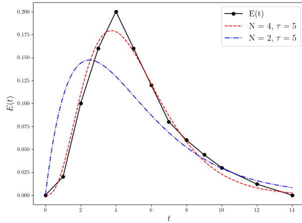
Figure 5.1.1: 3 different residence time distribution in experiments from 1) Fogler's book [4] 2) User2 block with 2 CSTRs and 3) User 2 block with 4 CSTRs
