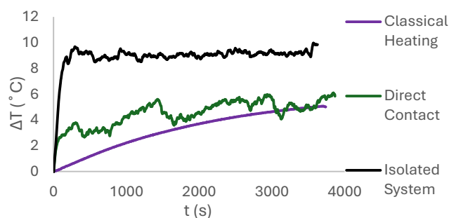
Figure 6: Temperature change for each heating system
