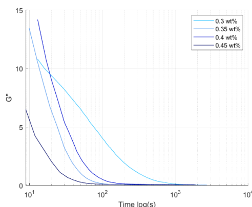
Figure 4.8 – Loss modulus against a log time axis over the relaxation period for LUDOX TM-50 gels at different PEO concentrations.
