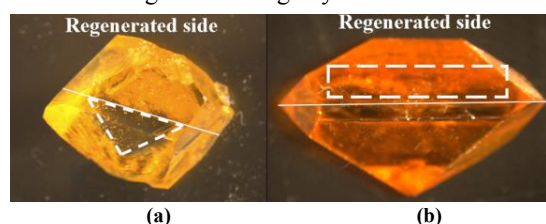
Figure 13 – Incorporation (a) and defect lines (b) in regenerated crystals
