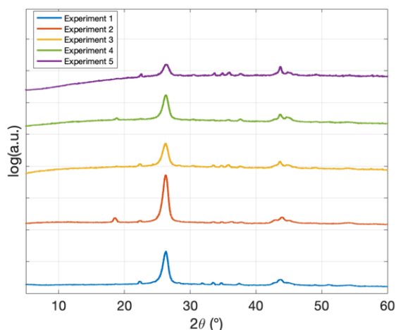
Figure 7. X-ray diffraction (XRD) of all experiments
