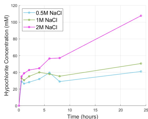
Figure 6: Plot of hypochlorite concentration (mM) over time at 75°C for various initial NaCl concentrations.
