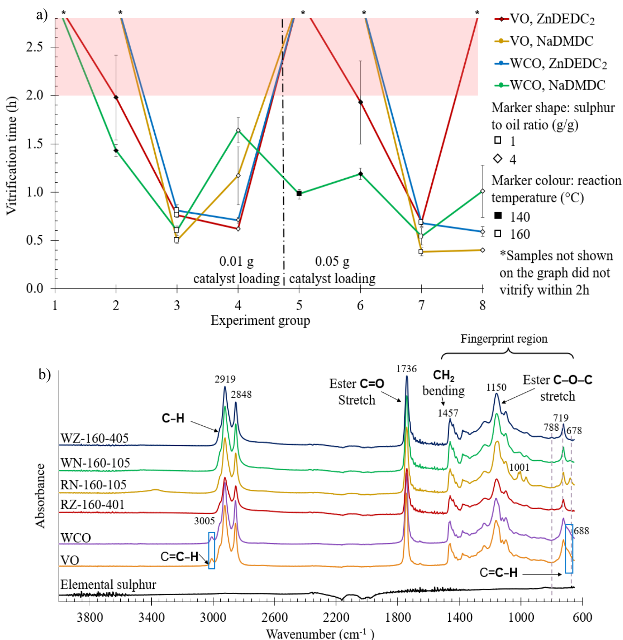
Figure 2 a) Summary of DOE results. b) FTIR spectrum of polysulphides and reactants
