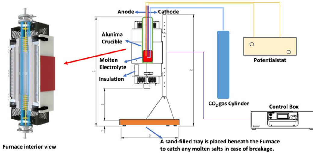
Figure 1. Experimental set-up & control system
