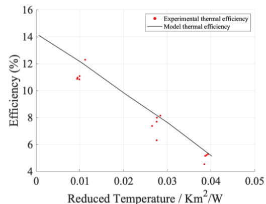
Figure 4.6. Bottom channel model validation with experimental data.
