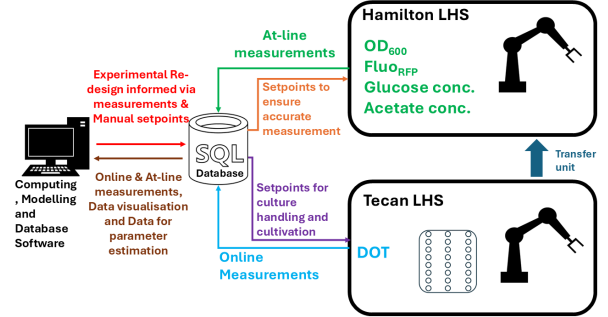
Figure 3: The KIWI-biolab platform integrates two robotic units: the Tecan LHS for managing MBR operations and the Microlab LHS for at-line analytical measurements. Connected by a transfer unit, the system automates microbial cultivation workflows, with online data integration into an SQL database for process monitoring and experimental redesign. Key measurements include optical density (OD), fluorescence, glucose concentration and DOT, adapted from [5].
