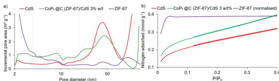
Fig. 10a-b: a) Differential area against logarithm of pore diameter plot and b) low pressure BET isotherms of CdS, CoP_x@C (ZIF-67)/CdS 3 w/t% and ZIF-67.
