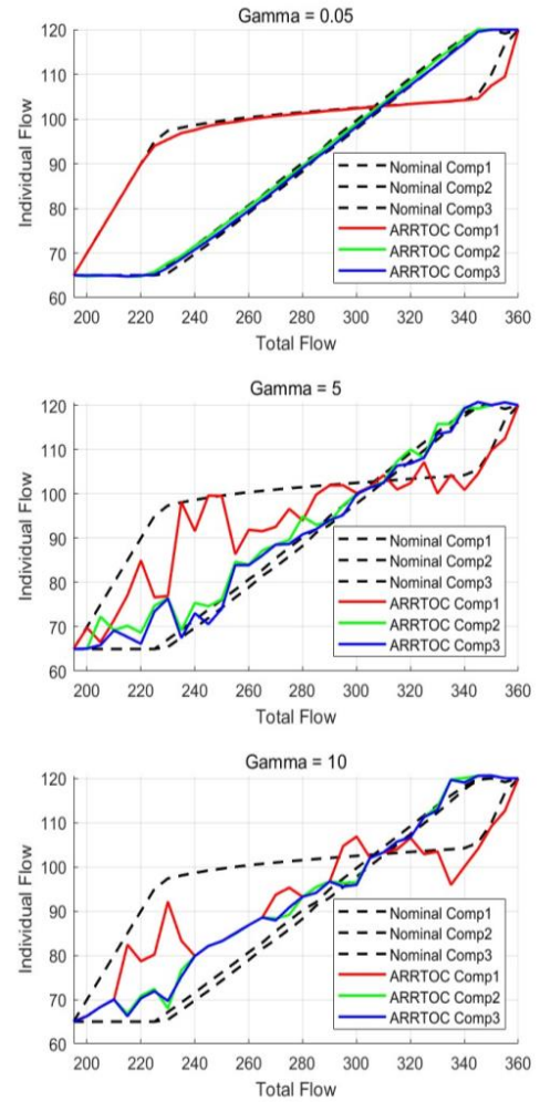
Figure 9. Nominal minimum individual flows versus ARRTOC minimum flows under varying \Gamma
