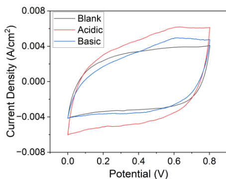
Figure 12. Cyclic Voltammograms of electro-deposited carbon papers with different pre-treatments at a scan rate of 10 mV/s.
