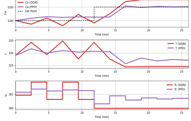
Figure 4: Unconstrained RL trajectories
