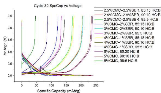
Figure 4.1-7: Specific Capacity vs. Voltage Graph for Cells of Different Composition from Cycle 30
