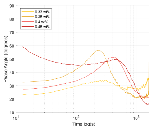
Figure 4.9 – Phase angle in degrees against a log time axis over the relaxation period for CS50-28 gels at different PEO concentrations.
