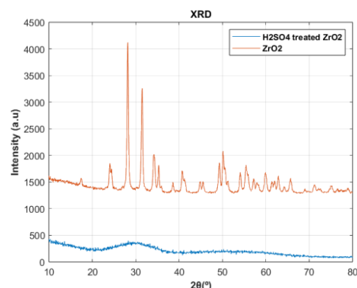
Figure 10. XRD patterns of ZrO 2 and H 2 SO 4 -treated ZrO 2 , highlighting the structural differences between the two.
