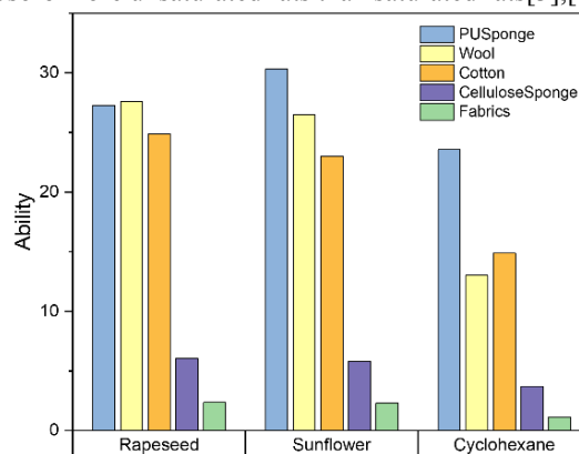
Figure 8. Oil Sorption Ability
