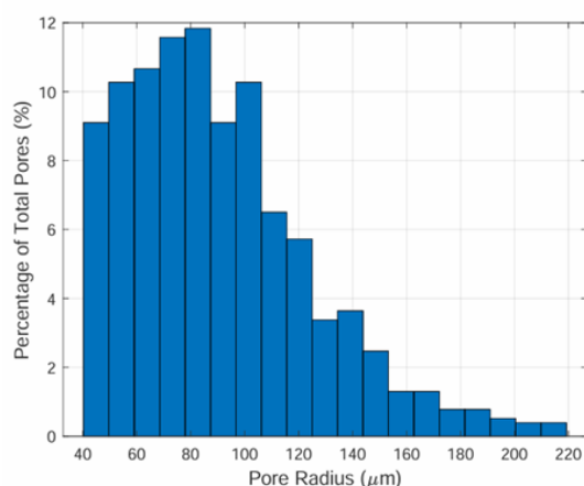
Figure 17. Histogram showing pore radii generated from the Pore Network Model function on Avizo.
