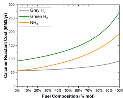
Figure 5. Calciner reactant Cost for all scenarios
