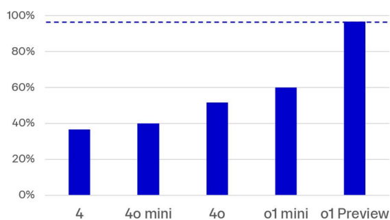
Figure 4.3.2.2.1 Average Performance Using Custom Mark Scheme
