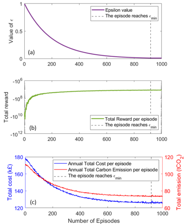
Figure 4: The training curve of the agent down the episode with nominal hyperparameters and a combination of reward weights of the best performance. (a) represents the exploration rate decay \epsilon down the episode; (b) shows the total reward convergence; (c) describes the annual electricity cost and carbon emission reduction down the episode
