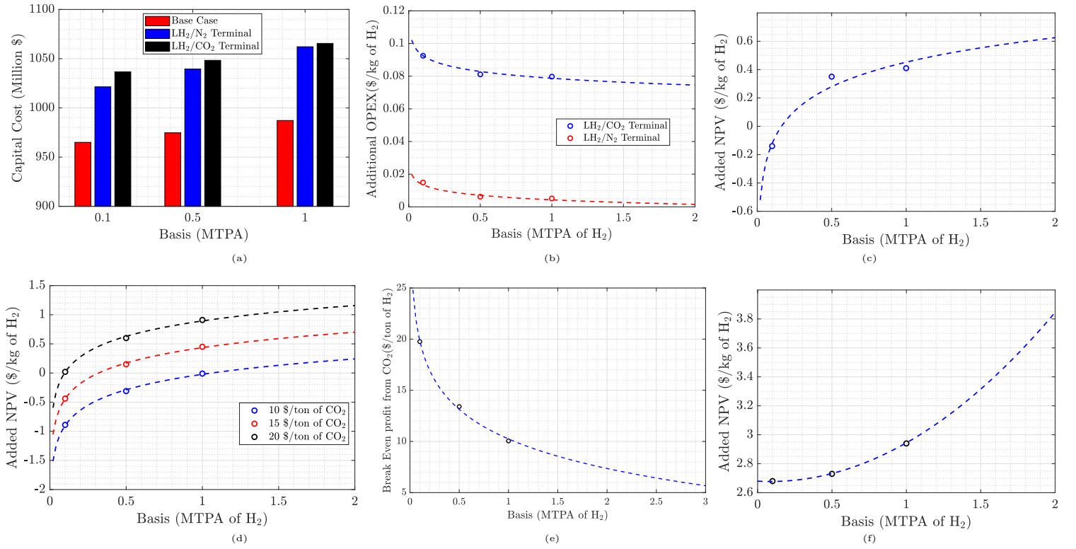
Figure 4: The X axis of all plots is the design basis of LH 2 throughput (MTPA of H 2 ) a = Capital Cost of Base Case, LH 2 /CO 2 and LH 2 /N 2 terminals. b = Added OPEX/kg of H 2 for LH 2 /CO 2 and LH 2 /N 2 terminals compared against the base case c = Added NPV per kg of H 2 for LH 2 /N 2 terminal d = Added NPV per kg of H 2 for different values of profit generated from CO 2 ($/tonneCO 2 ) - LH 2 /CO 2 terminal vs Base Case. e = Minimum required profit generated per tonne of CO 2 ($/tonneCO 2 ) to add value to the LH 2 /CO 2 terminal when compared against the base case. f = Added NPV per kg of H 2 for the integrated LH 2 /CO 2 when compared against two separate CO 2 and LH 2 terminals
