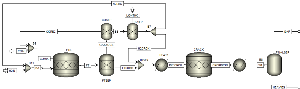
Figure 4.3: Full flowsheet for the FT unit with Syngas Recycling
