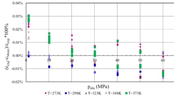
Figure 2. Deviation of toluene calibration experimental results from Meier's [9] data against absolute pressure
