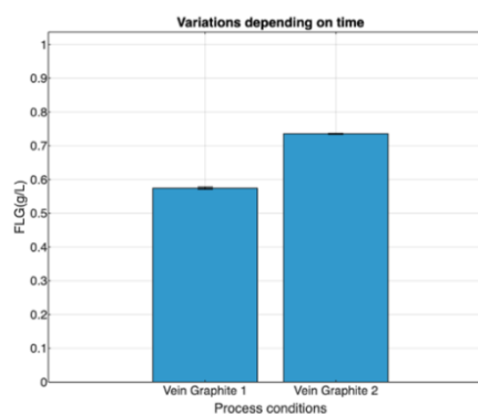
Figure 10 Variations of few-layer graphene concentration depending on time (left: 3 hours; right: 5 hours).
