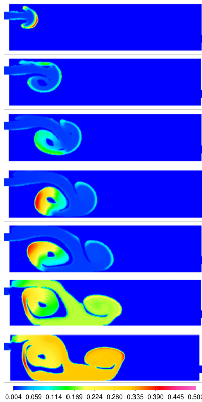
Fig. 7: Viscosity contour maps for static blood in units of [kg/m/s] varying with time for a 1 mm mesh size and 0.01 s time-step. The Onyx settles and hardens evenly after 2.5 s.
