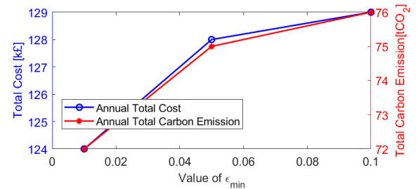
Figure 10: Cost and carbon analysis of minimum epsilon \epsilon_{min} , with fixed export penalty c_e of 0.55 and fixed cost coefficient w_1 of 80, trained through 1000 episodes
