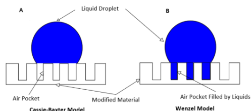
Figure 4. Cassie-Baxter Model and Wenzel Model
