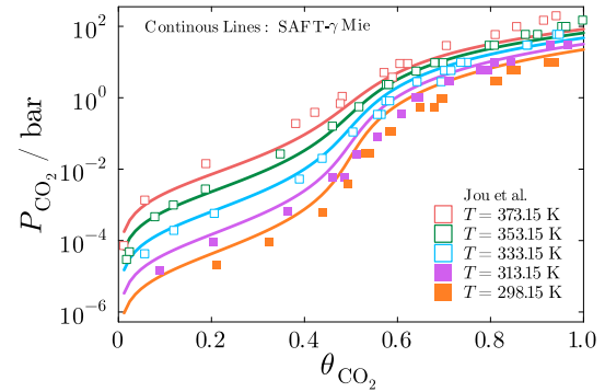
Figure 5: CO 2 loading in 30 w_{\text{MEA}}\% aqueous MEA [12]. Experimental data is depicted as square markers [40], with filled squares indicating the data was used in parameter estimation.
