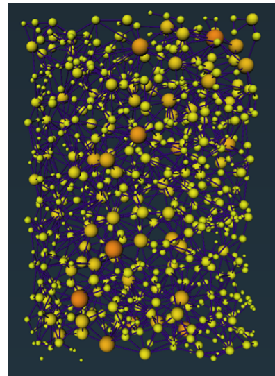
Figure 16. Visualisation of the macropore connectivity using the Generate Pore Network Model function in Avizo with dimensions of 1401 \times 2018 \times 500 \text{ voxels}^3 (width x height x depth)
