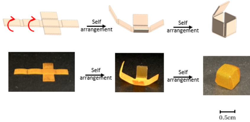
Figure 13: Self-assembly process of a 2D polymer into a 3D cube structure. The top panel illustrates the expected transformation from a flat 2D polymer sheet into a 3D enclosed cube structure via self-arrangement. The middle panel shows the actual sequential stages of self-arrangement for a 0.5 cm square side length and 0.1 cm hinge width structure. Scale bar: 0.5 cm.
