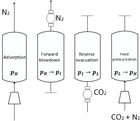
Figure 1. The PVSA Process
