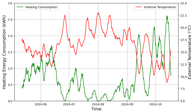
Figure 11: Heating energy consumption: actions selected by the trained DDPG agent.
