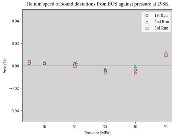
Figure 3: Speed of sound deviations of helium from the EOS
