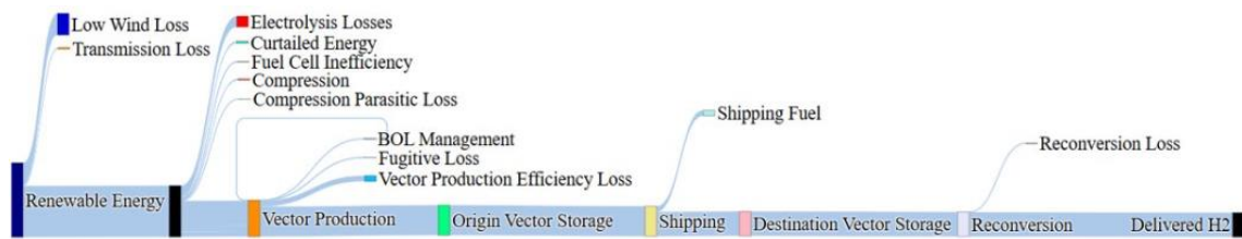
Figure 3. Detailed scaled breakdown of the energy flows, losses, and inefficiencies across the green hydrogen supply chain. Losses through each stage are highlighted, with wind energy conversion and electrolysis combined. Specific energy values are based on the output of the optimisation model [31].
