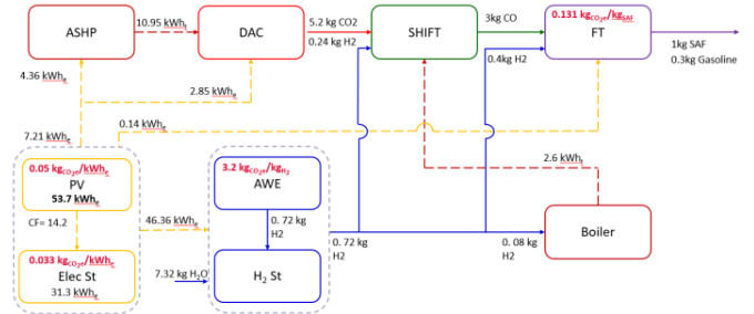
Figure 8 – Block Diagram for DAC route
