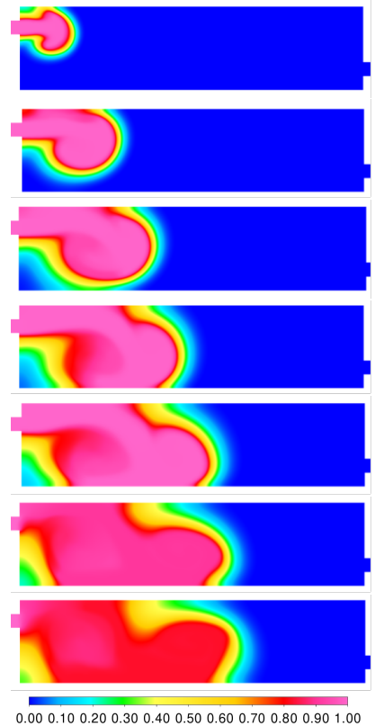
Fig. 8: Scalar maps for static blood varying with time for a 1 mm mesh size and 0.01 s time-step. As for scalar motion, it advances faster than glue in early stages, leading to high viscosities at the interface.
