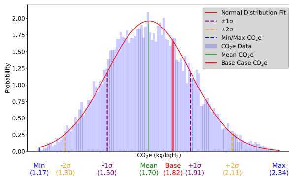
Figure 7. Results of the uncertainty analysis. 10,000 model iterations were compiled into a histogram and fitted with a normal distribution. Standard deviation percentiles have been indicated from the mean, with the base case value also being highlighted.
