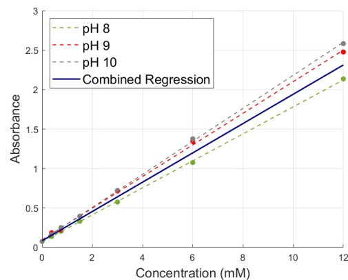
Figure 2: Linear regression relationship of concentration of hypochlorite ions against absorbance in the UV-Vis spectrum, at 292 nm varying the pH.
