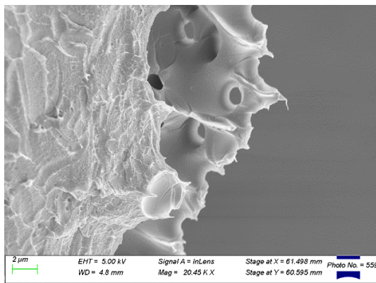
Figure 8 SEM image of a cross-section of polymer particle with composition of 8% w-w polystyrene, as seen with the interior of the particle in the foreground of the image.
