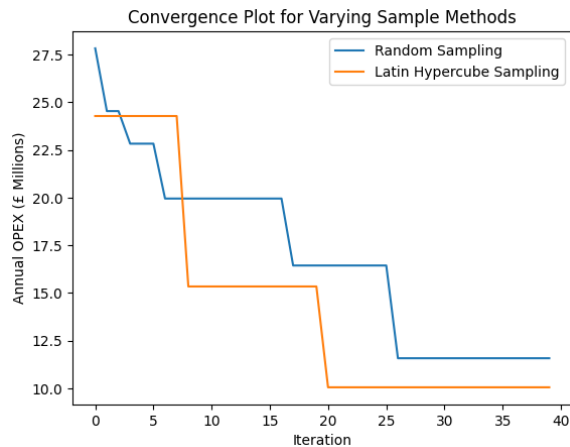
Figure 2: Annual Operational Expenditure (OPEX) convergence plot for Bayesian optimisation given different sampling methods: Random and Latin Hypercube Sampling.
