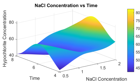
Figure 8: The combined effect of NaCl concentration and time on hypochlorite concentration
