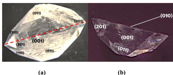
Figure 5 – Facet Miller indices and cleavage scheme for (a) an ethanol-grown paracetamol crystal and (b) a cleaved crystal.
