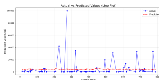
Figure 13 – Actual vs. Predicted Production Cost using XGBoost.
