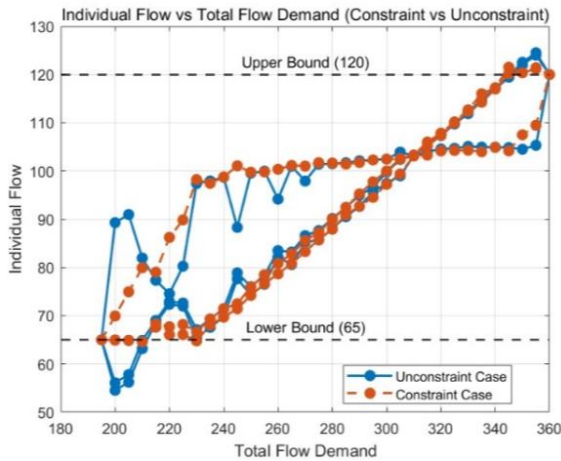
Figure 6. Individual flow versus total flow demand for unconstrained and constrained cases
