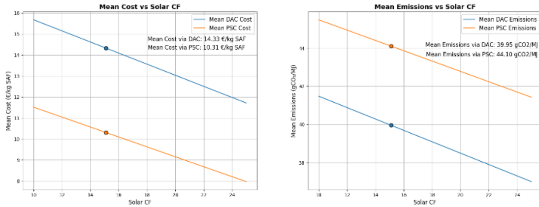
Figure 10 – Sensitivity analysis of solar capacity factor against cost and emission outputs via python model
