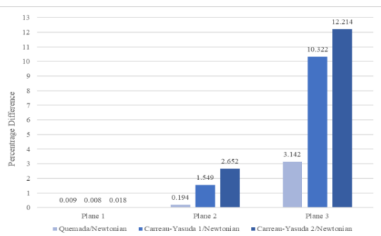
Figure 8.2 Percentage difference in maximum spatial mean velocity between non-Newtonian and Newtonian models
