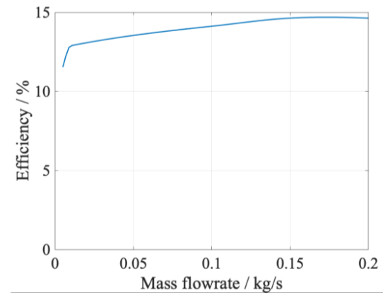
Figure 4.2. Effect of varied mass flowrate on bottom channel thermal efficiency. A rise in mass flowrate yields greater thermal efficiency.
