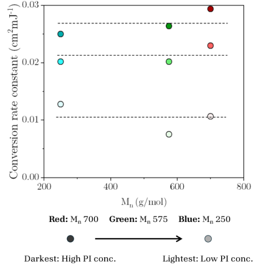
Figure 7: Effect of molecular weight ( M_n ) and photoinitiator concentration on the conversion rate constant, K ( \text{cm}^2\text{mJ}^{-1} ). Data points are colour-coded: red ( M_n=700 ), green ( M_n=575 ) and blue ( M_n=250 ). Darkness of markers corresponds to PI concentration, with darker shades indicating high PI concentrations. The plot shows that changing the PI concentration has a greater effect on K than changing the M_n of PEGDA. K increases as PI concentration increases.
