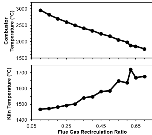
Figure 4 Effect of flue gas recirculation ratio on combustor temperature and kiln temperature.
