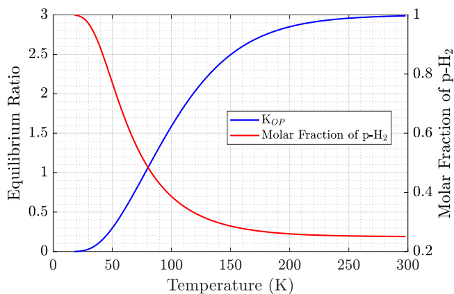
Figure 2: Equilibrium Ratio and Molar Fraction of p-H_2 vs Temperature
