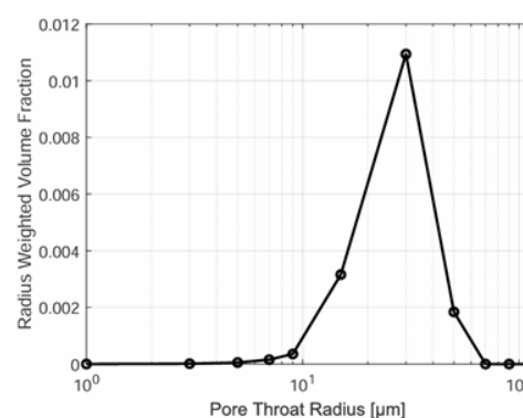
Figure 19. Pore throat size distribution
