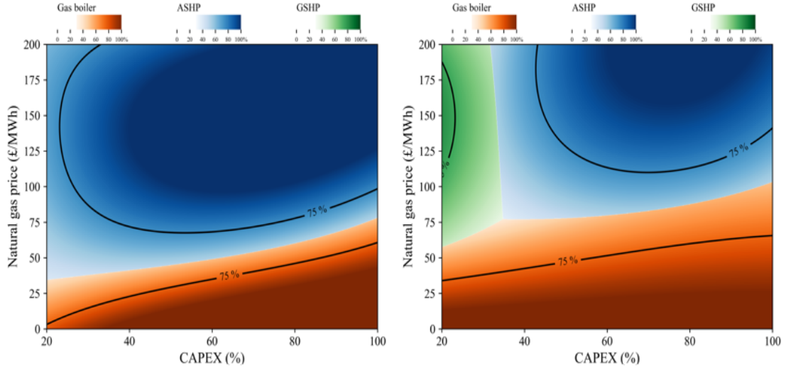
Figure 4: Natural gas price against CAPEX percentage graphs representing the competitive landscape of the domestic heating sector at grid cost factors of 0 and 750 m£/GW
