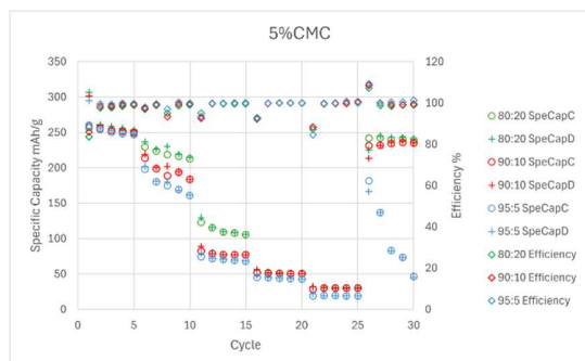
Figure 4.2-4: Cycle vs. Specific Capacity & Efficiency Graph for 5% CMC
