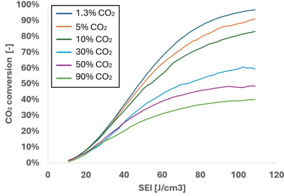
Figure 9. Plots of conversion against increasing specific energy input, determined via model sensitivity analysis, varying the initial CO 2 mol fraction. An S-curve have been traced at all CO 2 fraction, with a high initial increase and levelling at high SEI. Different conversion plateau has been reached, the highest (100% conversion) at 1.3% CO 2 inlet fraction, and the lowest (40% conversion) at 90% CO 2 inlet fraction.
