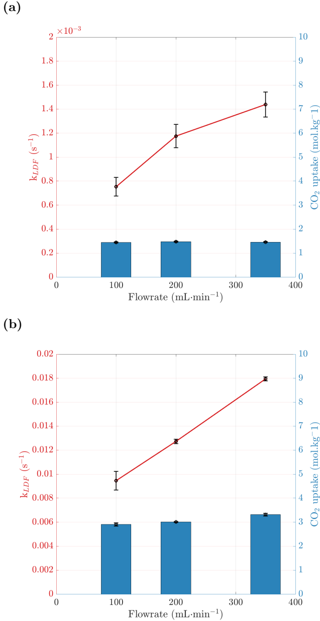
Figure 5: Quantitative analysis of the flowrate tests carried out gravimetrically at F = 100, 200 and 350 \text{ mL.min}^{-1} between p/p_0(\text{CO}_2) = 0.03 to 0.06 at 303 \text{ K} for: (a) Z50-B50 and (b) Z100-B0. In red: k_{LDF} obtained from the LDF fit; blue: \text{CO}_2 uptake at p/p_0(\text{CO}_2) = 0.06 .
