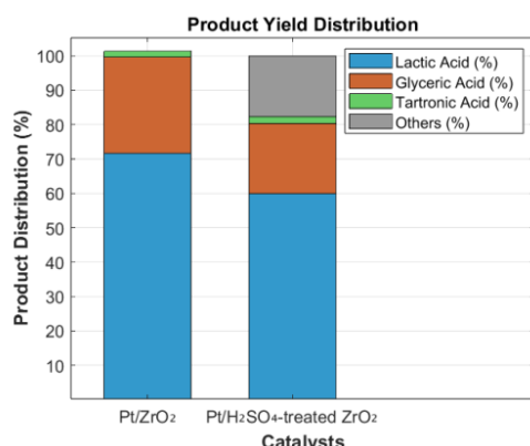
Figure 8. Product yield distribution of Pt/ZrO 2 and Pt/H 2 SO 4 -treated ZrO 2 in MEA setup.
