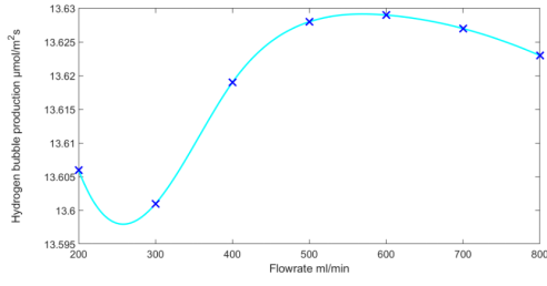
Figure 7: Hydrogen bubble production against flowrate
