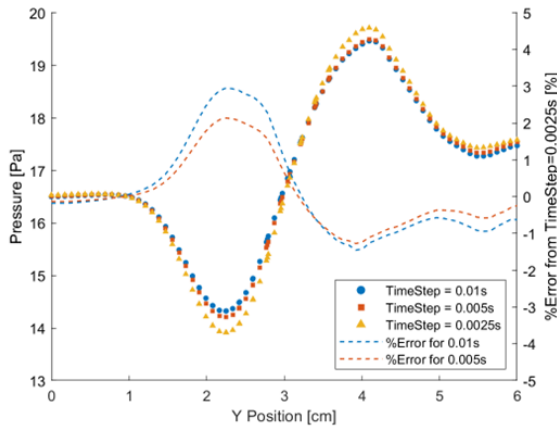
Figure 5: Pressure relationship graph with time-step and associated error
