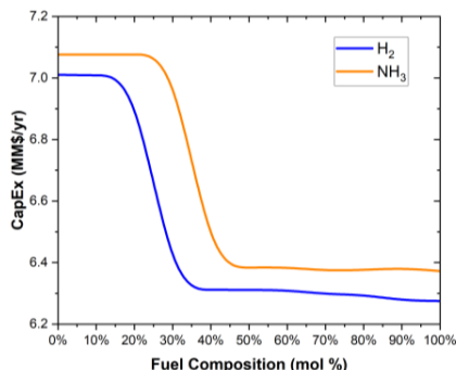
Figure 4. CapEx for both H 2 and NH 3 scenarios
