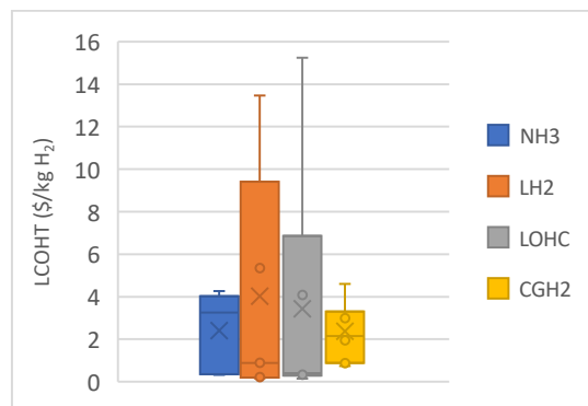
Figure 3. Cost ranges for trucks by conditioning
