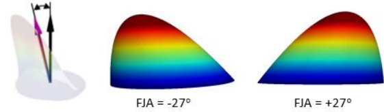
Figure 6.2 Flow jet angle of skewed parabolic velocity profiles
