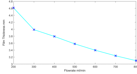
Figure 5: Hydrogen gas film thickness against inlet flowrate of electrolyte
