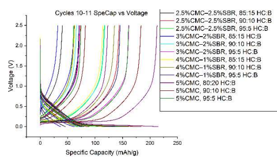
Figure 4.1-3: Specific Capacity vs. Voltage Graph for Cells of Different Composition from Cycle 10-11
