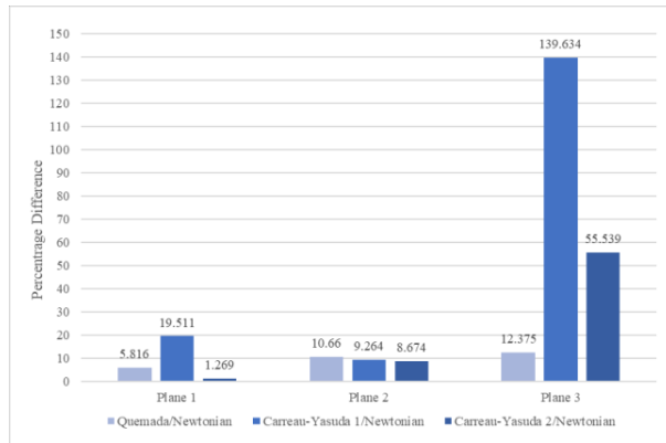
Figure 10.1 Percentage difference in maximum WSS between non-Newtonian and Newtonian models
