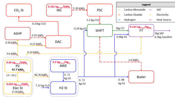
Figure 7 – Block Diagram for PSC route
