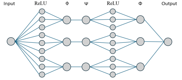
Figure 2: Our Multi-Layer Perceptron Network
