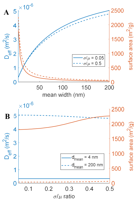
Figure 5: A) Effective straight pore diffusivity and surface area as a function of mean pore width at different \sigma/\mu ratios B) Effective straight pore diffusivity and surface area as a function of \sigma/\mu ratio at different mean pore widths
