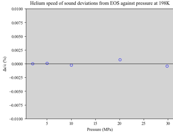
Figure 5: Speed of sound deviations of helium from the EOS by Ortiz-Vega et al.[22] at 198K
