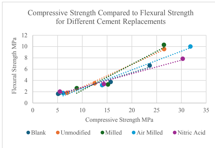
Figure 5. Compressive Strength Compared to the Flexural Strength
