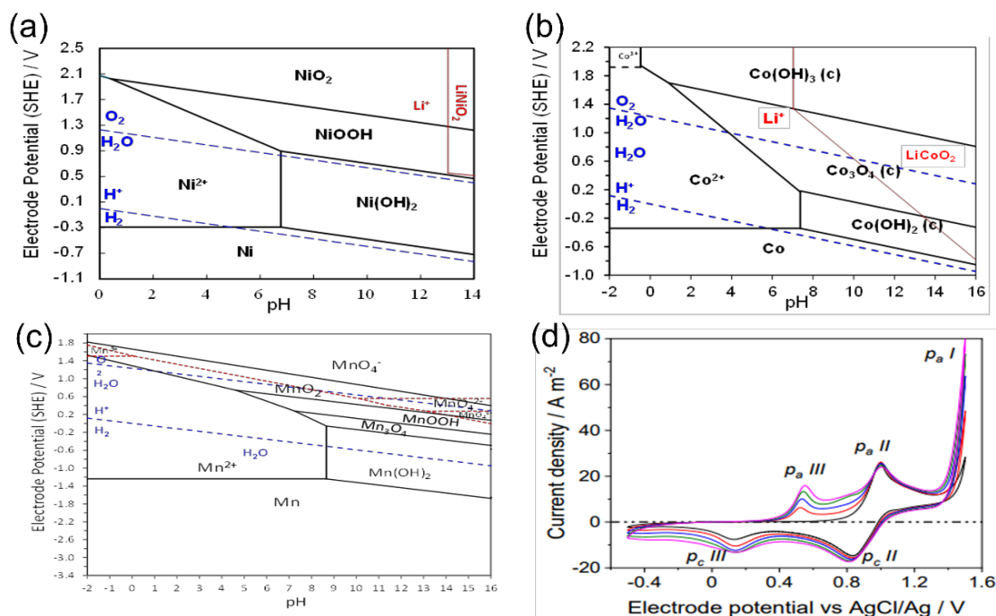
Figure 1. (a), (b), (c) Pourbaix Diagram of nickel-water, cobalt-water and manganese-water solutions. (d) Cyclic voltammetry Diagram for solution made by \text{NiSO}_4 , \text{MnSO}_4 and \text{CoSO}_4 , all fixed at 0.01 M, using 0.25 M \text{Li}_2\text{SO}_4 as electrolyte [19].
