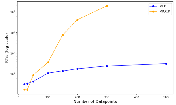
Figure 7: Runtime Comparison of MLP and MIQCP Models
