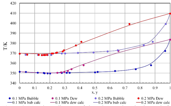
Figure 9 (a). Phase diagram of the toluene-ethanol mixture before parameters tuning
