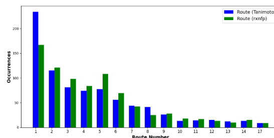
Figure 6 - AZF Top 15 Routes Identical Matches with Both Methods
