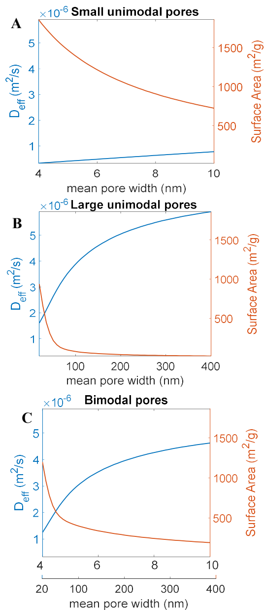
Figure 6: Effective straight pore diffusivity and surface area as a function of mean pore width for A) a unimodally distributed material with small pores B) a unimodally distributed material with large pores C) a bimodally distributed material with both small and large pores
