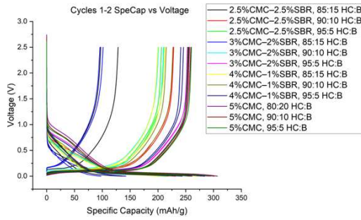
Figure 4.1-1: Specific Capacity vs. Voltage Graph for Cells of Different Composition from Cycle 1 to 2
