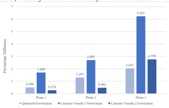
Figure 8.1 Percentage difference in maximum velocity between non-Newtonian and Newtonian models
