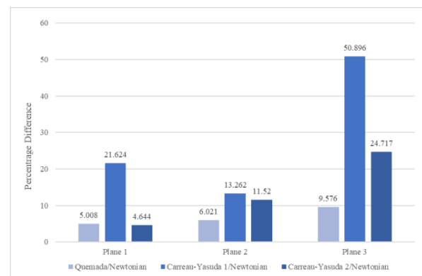
Figure 10.3 Percentage difference in maximum TAWSS between non-Newtonian and Newtonian models
