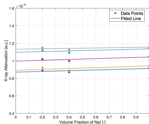
Figure 13. X-ray attenuation against volume fraction of NaI for 5 grain-size rubber sub volumes plotted from Matlab
