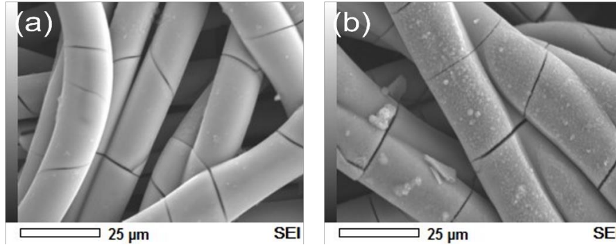
Figure 10. SEM images electrodeposited carbon paper under different pre-treatments: (a) Acidic treatment (b) Basic treatment.
