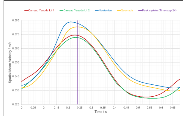
Figure 9.1 Plane 3 spatial mean velocity as a function of time between all 4 non-Newtonian models
