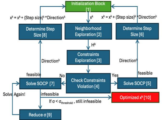
Figure 2. High-level schematic of the ARRTOC Framework
