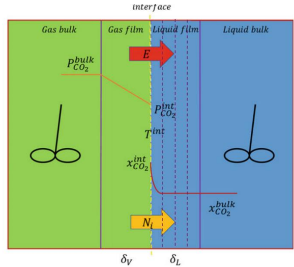
Figure 2 Concentration profile gas-liquid interface.[13]
