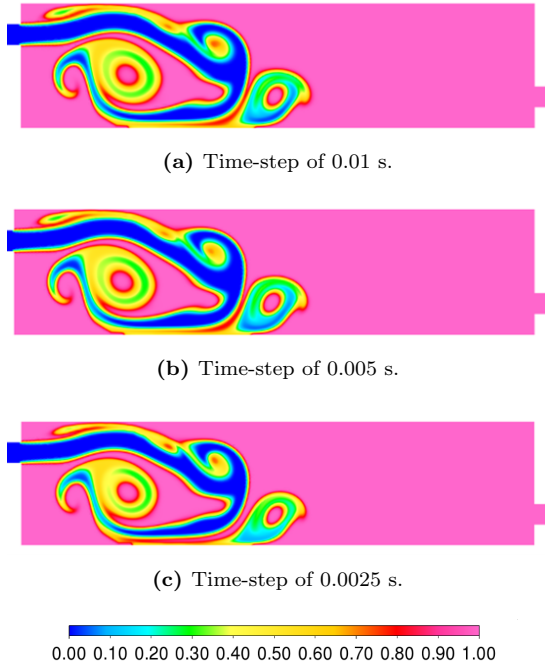
Figure 4: Concentration maps taken at a flow time of 2.5 s for different time-steps. The colorbar below illustrates the scale used in the analysis.
