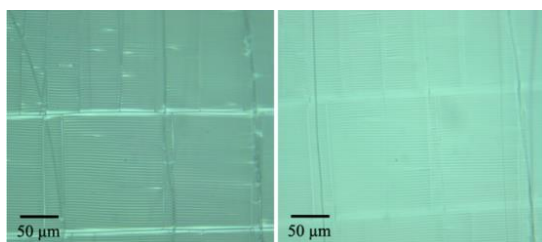
Figure 3: 3.7 \pm 0.3 \mu\text{m} sample before (left) and after (right) exposure to 60s of 99W plasma.
