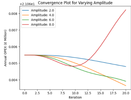
Figure 11: Annual Operational Expenditure (OPEX) convergence plot for Extremum Seeking Control given different initial values
