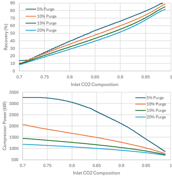
Figure 8. Liquefaction Process Purge Sensitivity
