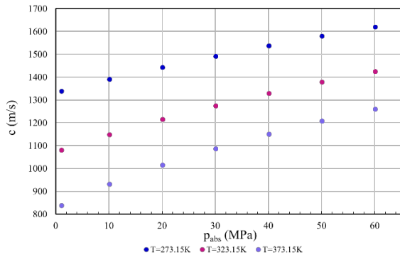
Figure 4. Sound speed against absolute pressure in pure cyclopentane
