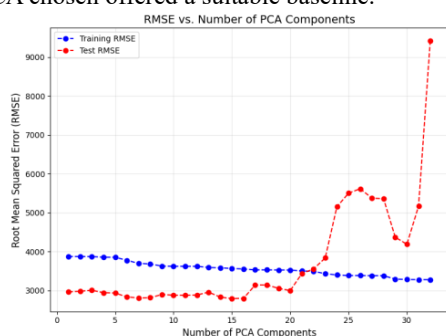
Figure 8 - Test and Validation RMSE Plot against Number of PCA Components
