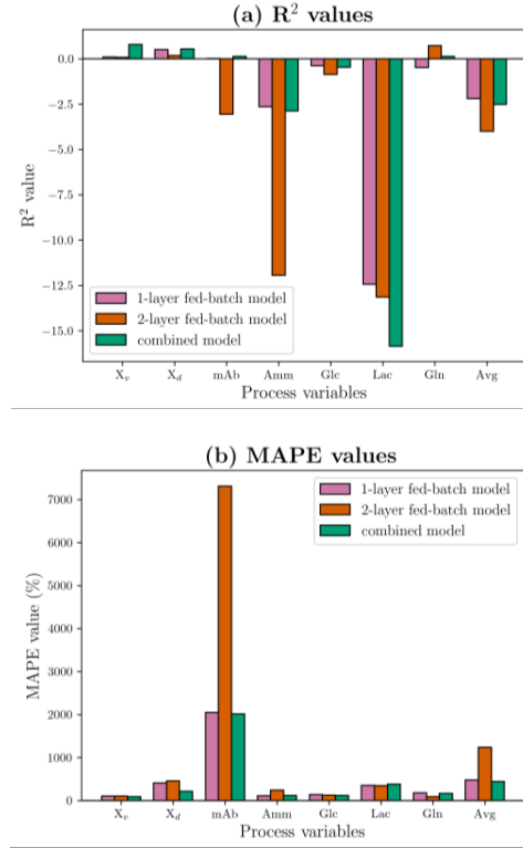
Fig. 5. Bar charts of metrics for fed-batch data predictions, broken down by process variable. (a) R^2 values. (b) MAPE values.
