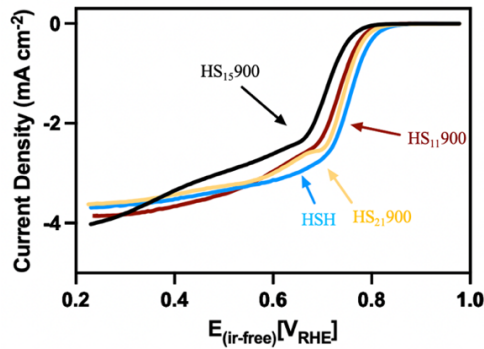
Figure 2: The RRDE results for sample of HS 11 900 HS 21 900, and the reference sample HSH900 without S atom doping, Capacitance-corrected cathodic scan
