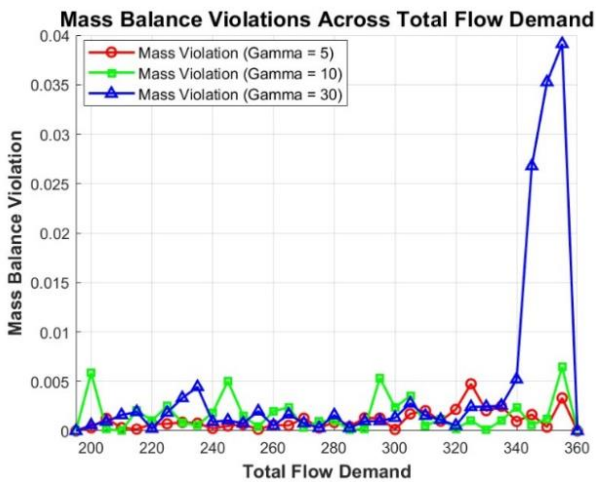
Figure 11. MV under varying \Gamma values across different total flow demands
