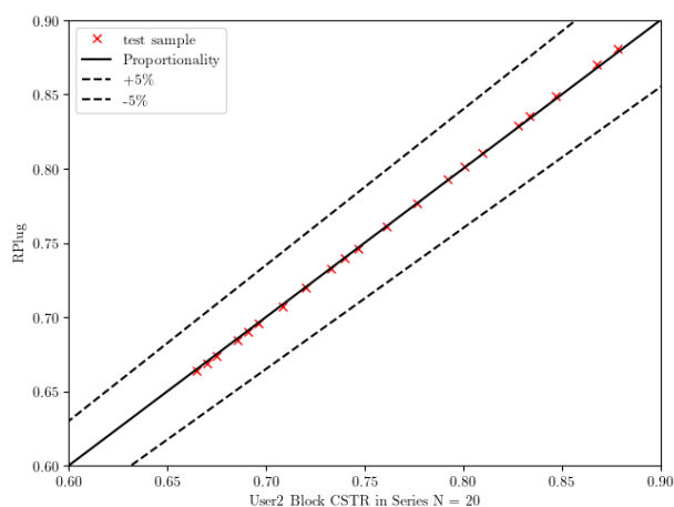
Figure 4.1.1: Parity Plot on Comparing a Set of Results on DEC Selectivity From a Aspen User2 Block against Aspen RPlug Block
