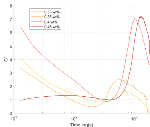
Figure 4.10 – Storage modulus against a log time axis over the relaxation period for CS50-28 gels at different PEO concentrations.
