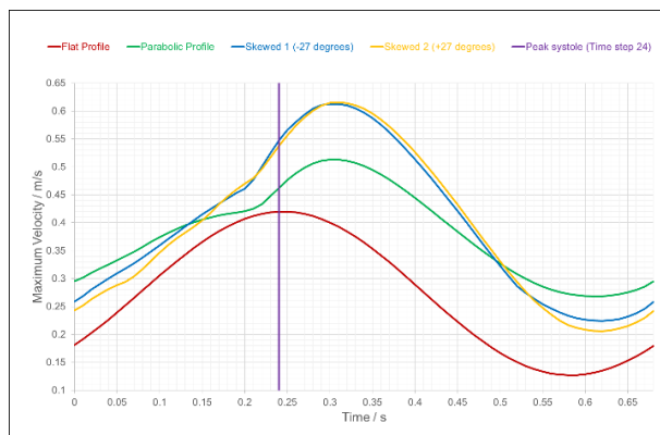
Figure 13.1 Plane 1 maximum velocity as a function of time between all 4 varying inlet boundary condition models
