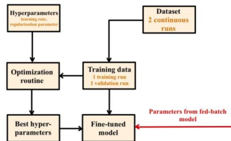
Fig. 2. Model development workflow for transfer models.
