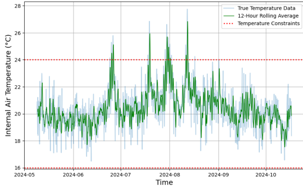
Figure 10: Internal Air Temperature as a result of actions selected by the trained DDPG agent.
