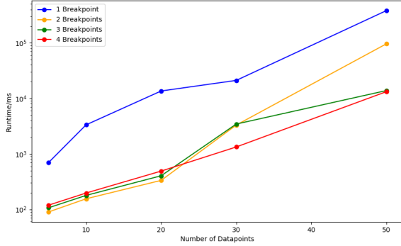
Figure 5: Runtime vs Breakpoints Across Datapoints
