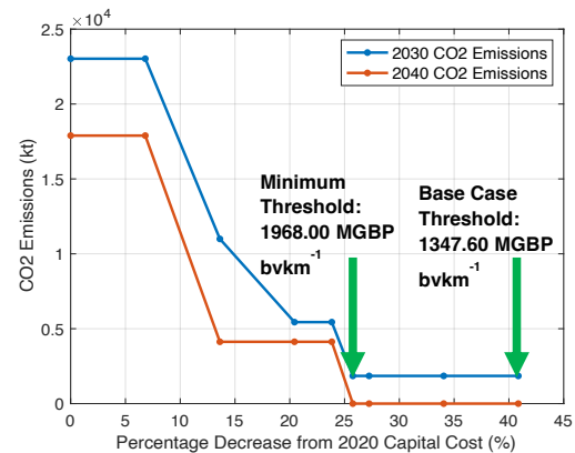
Figure 9. Sensitivity analysis on capital costs for years 2030 and 2040, with minimum threshold and base case threshold capital costs
