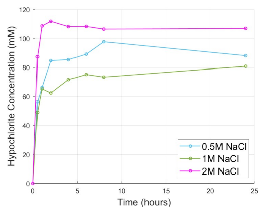
Figure 4: Plot of hypochlorite concentration (mM) over time at 25°C for various initial NaCl concentrations.
