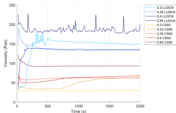
Figure 4.1 – The viscosity against time for a selection of shake gels with different PEO concentrations under 800 \text{ s}^{-1} constant shear rate. LUDOX TM-50 in blues, CS50-28 in reds/oranges.
