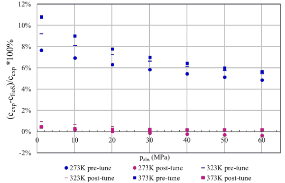
Figure 8. Deviation of measured sound speed in toluene-ethanol mixture from the EoS predictions against absolute pressure before and after parameters tuning
