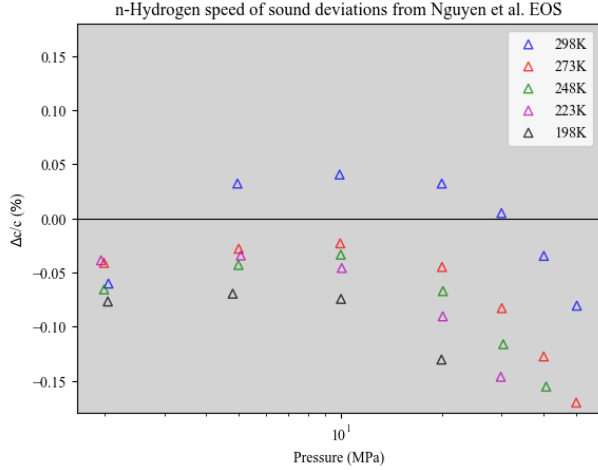
Figure 7: Deviations of n-hydrogen data from Nguyen et al. [9]
