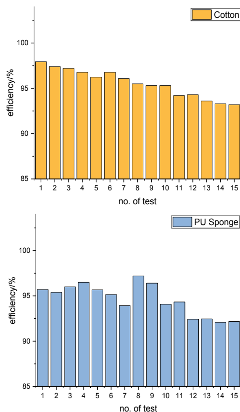
Figure 14&15. Oil Sorption Efficiency of Cotton and PU Sponge through 15 cycles
