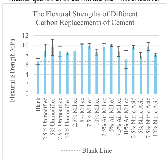
Figure 2. The Flexural Strength After 28 Days
