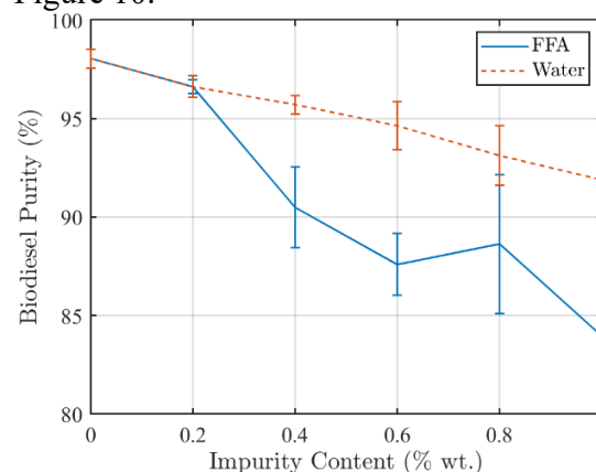
Figure 10: Effect of Impurity Concentration on Biodiesel Purity.
