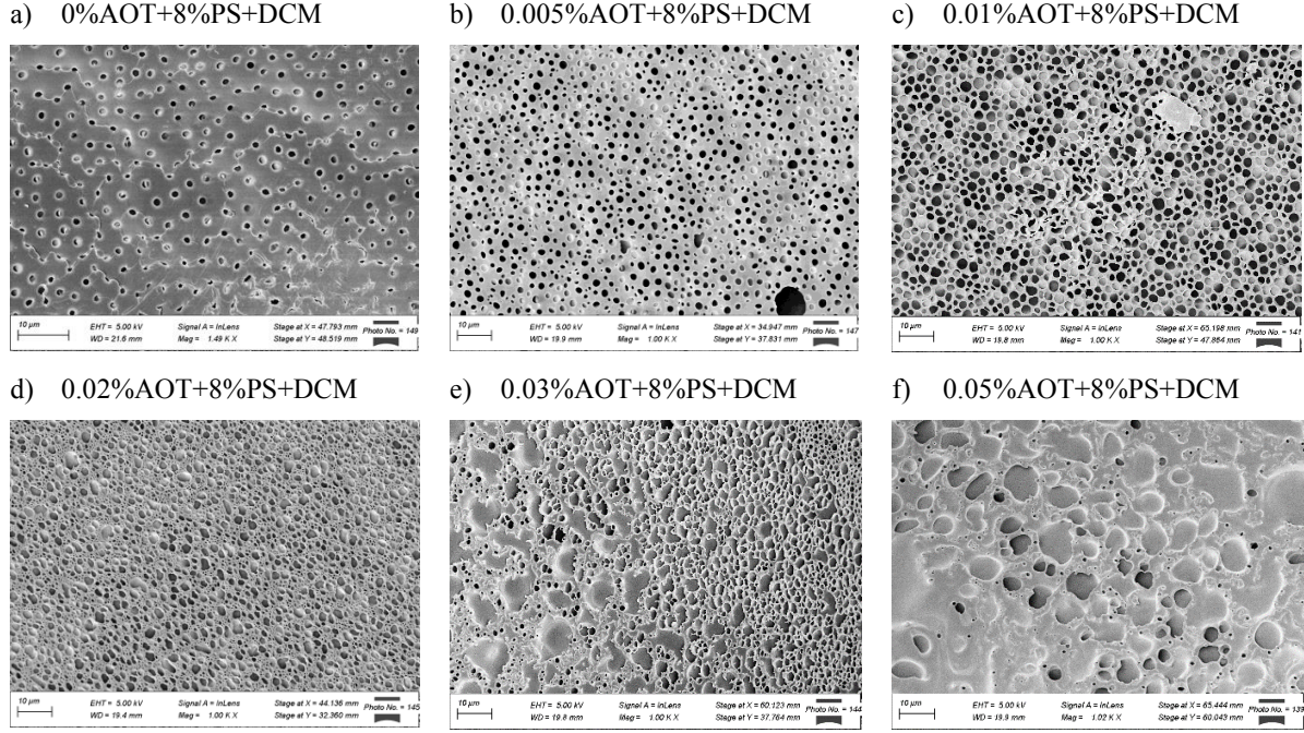
Figure 3 Scanning Electron Microscopy (SEM) results of different surfactant added samples (all samples prepared in 40%RH, 21°C and constant polystyrene concentration). These images characterise the surface morphology of polystyrene (PS) samples prepared with varying surfactant (AOT) concentrations in the solvent, dichloromethane. The subfigures arranged from a) to f) represent increasing surfactant concentrations from 0 to 0.05 w/w%.
