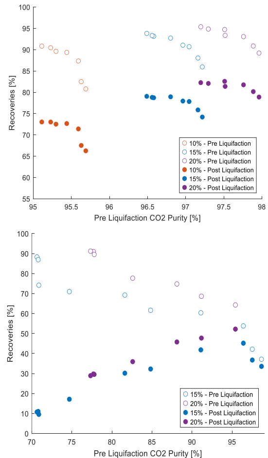
Figure 6. Z13X (top) and AC (bottom) Recovery Pareto Fronts
