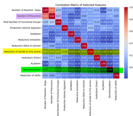
Figure 16. Correlation matrix of selected features. Highlighted rows correspond to the top 3 features in Figure 15
