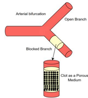
Figure 2. Schematic representation of the arterial bifurcation, with the behaviour in the occluded artery (blocked branch) represented by the local PD model.
