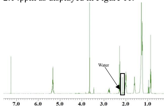
Figure 11: NMR Spectrum Showing Water Peak (Units of ppm).
