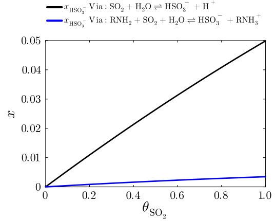
Figure 8: Predicted mole fractions of \text{HSO}_3^- in 30 w_{\text{MEA}}\% aqueous MEA at T = 298.15 K, accounting for the two different speciation routes.
