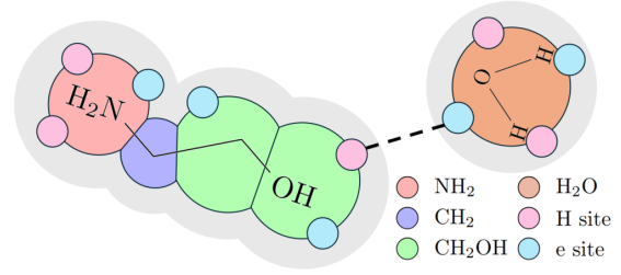
Figure 1: MEA + H 2 O, described for a SAFT- \gamma Mie GC approach. The dotted line shows CH 2 OH H site associating with H 2 O e site, with grey shading marking a chain of segments.
