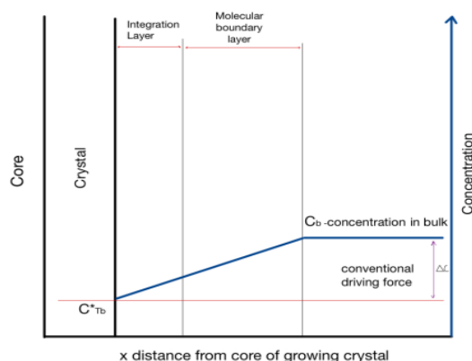
Figure 1 - Linearised profiles of conventional crystallisation driving forces, displaying the layers of crystallisation
