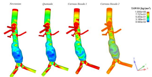
Figure 11 TAWSS contours of geometry wall of Newtonian model (left), Quemada model (left centre), Carreau-Yasuda 1 (right centre), Carreau-Yasuda 2 (right)
