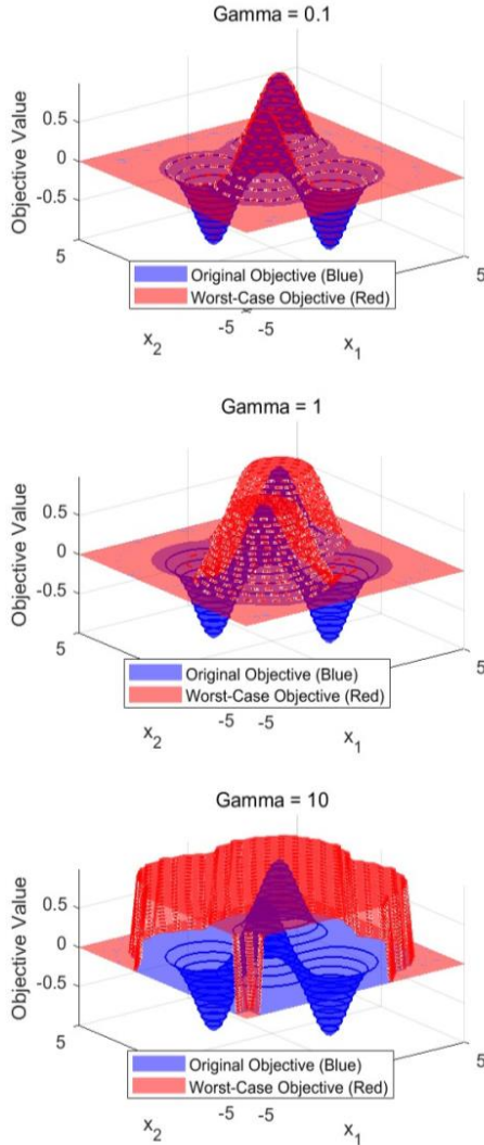
Figure 4. 3D comparison of nominal and worst-case objective functions under varying \Gamma values for f(x_1, x_2) = e^{-(x_1-1.5)^2+(x_2-1.5)^2} + e^{-(x_1+1.5)^2+(x_2+1.5)^2} - e^{-(x_1-1.5)^2+(x_2+1.5)^2} - e^{-(x_1+1.5)^2+(x_2-1.5)^2}
