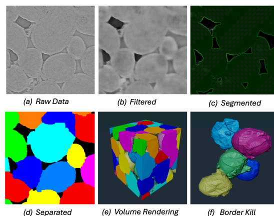
Figure 2. Workflow showing the different image processing steps performed for 500^3 voxels 3
