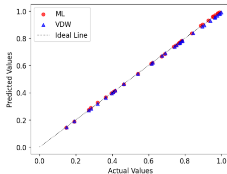
Figure 9: ML vs Van der Waals equation
