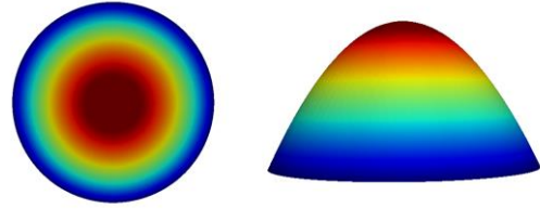
Figure 6.1 Standard parabolic velocity profile implemented
