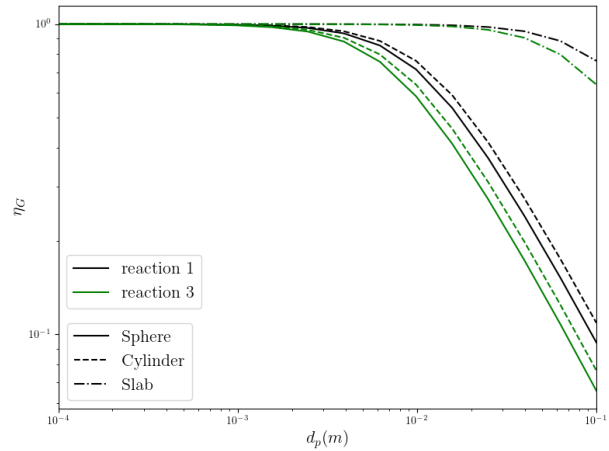
Figure 5.3.1: The relationship of the global effectiveness factor on catalyst particle diameter and geometry, shown on a log-log scale
