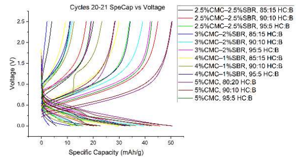
Figure 4.1-5: Specific Capacity vs. Voltage Graph for Cells of Different Composition from Cycle 20-21
