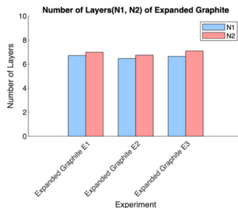
Figure 8 Number of layers (N1, N2) of expanded graphite
