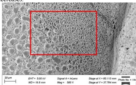
Figure 10: Zoomed out SEM image taken of polystyrene particle from a solution of 8% Polystyrene, 0.03% AOT in DCM.
