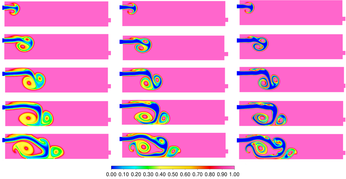
Figure 2: Concentration contours for course mesh size of 2 mm (left column), medium mesh size of 1 mm (central column), and fine mesh size of 0.5 mm (right column).
