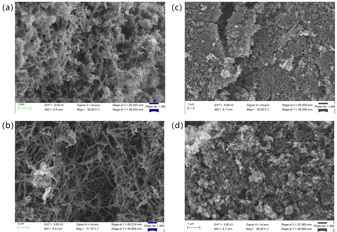
Figure 9. Scanning electron microscopy (SEM) images of carbon products. (a) SEM image from Experiment 1 (b) SEM image from Experiment 2 (c) SEM image from Experiment 3 (d) SEM image from Experiment 5,. Scale bars indicate 1–2 \mu\text{m} as labeled.
