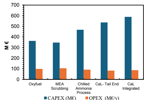
Figure 6 Comparison of CAPEX and OPEX of different CCS technologies
