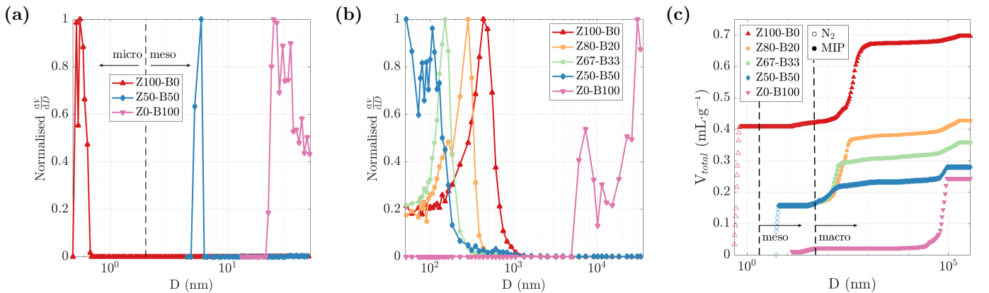
Figure 3: Pore size distributions (PSD) of the samples: (a) normalised differential PSD in the micro- and mesopore range for Z100-B0, Z50-B50 and Z0-B100 obtained from \text{N}_2 physisorption at 77 K; (b) normalised differential PSD in the macropore range for Z100-B0, Z80-B20, Z67-B33, Z50-B50 and Z0-B100 obtained from MIP; and (c) cumulative PSD for Z100-B0, Z80-B20, Z67-B33, Z50-B50 and Z0-B100 obtained from \text{N}_2 physisorption at 77 K and MIP combined.
