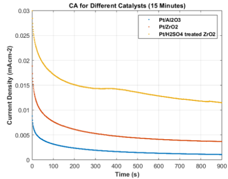
Figure 3. CA curves of Pt-based Al 2 O 3 , ZrO 2 , and H 2 SO 4 -treated ZrO 2 for 15 minutes.
