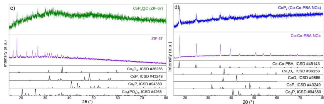
Fig. 6a-d: XRD of a) \text{CoP}_x ( \text{CoCl}_2 ), b) \text{CoP}_x ( \text{Co}_3\text{O}_4 ), c) \text{CoP}_x @C (ZIF-67) and ZIF-67, d) \text{CoP}_x (Co-Co-PBA NCs) and Co-Co-PBA NCs.
