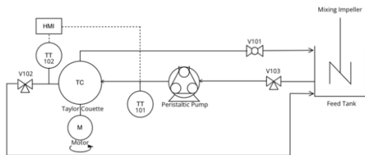
Figure 3 Schematic showing the experimental setup
