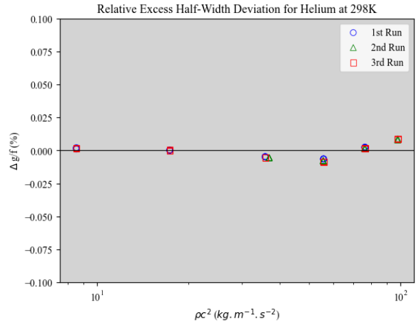
Figure 4: Excess half-widths of helium at 298K
