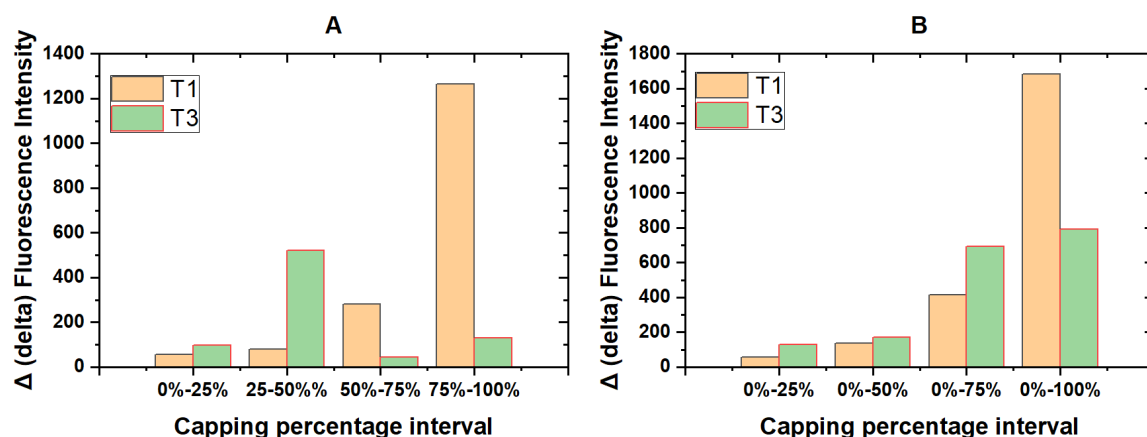
Figure 7 The graphs illustrate the \Delta (delta) fluorescence intensity, calculated by subtracting fluorescence values based on the capping percentage intervals shown on the x-axis. The baseline is set at 0% capping, and the delta values represent the changes in fluorescence relative to this reference point. In the A graph, the differences are calculated between consecutive intervals (e.g., 25%-50%), highlighting the sensitivity of T1 and T3 to incremental capping changes. The cumulative graph B shows fluorescence intensity changes from the baseline, 0% capping, to each interval, demonstrating the overall fluorescence behaviour across the full capping range.
