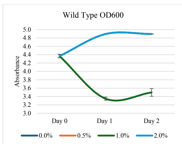
Figure 5. Line graph for Wild Type OD 600 absorbance throughout the induction period. Some concentrations are hidden beneath other lines – can be better seen in figure 5 .
