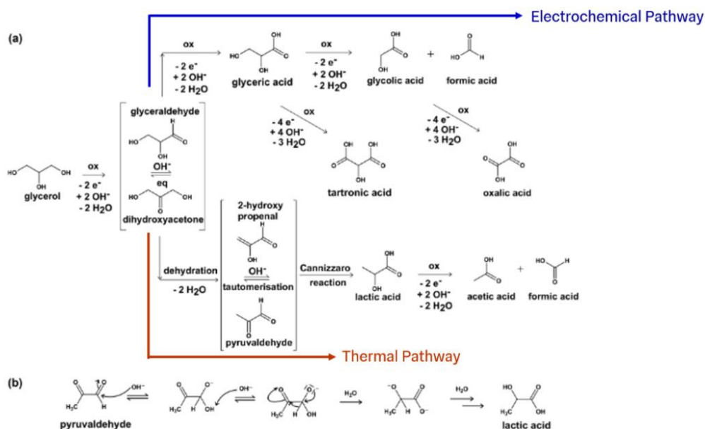
Figure 1. (a) GEOX reactions, illustrating the formation of key intermediates, and their subsequent transformations into products. (b) Mechanism of pyruvaldehyde conversion into lactic acid via the Cannizzaro reaction, driven by hydroxide-assisted tautomerization and hydration steps (Dai, et al., 2017).
