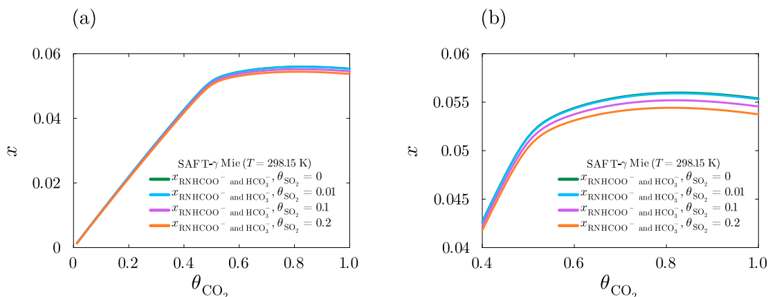
Figure 10: Predicted mole fractions of \text{RNHCOO}^- at variable \text{CO}_2 loading in 30 w_{\text{MEA}} % solution, with lines of fixed \text{SO}_2 loading. Unmagnified plot (a), magnified plot (b)
