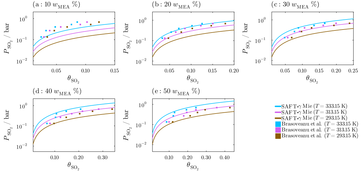
Figure 7: SO 2 loading in 10-50 w_{\text{MEA}} % in H 2 O . Experimental data is depicted as square markers [43], with filled squares indicating the data was used in parameter estimation.
