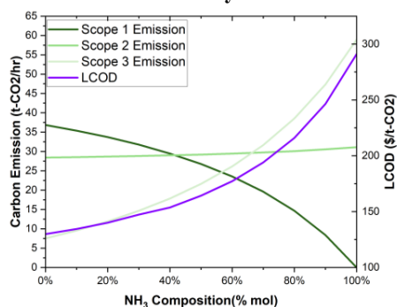
Figure 8. Carbon emission for NH 3 scenarios
