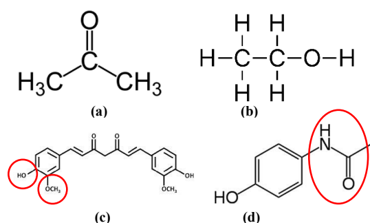
Figure 2 – Chemical structure of (a) acetone, (b) ethanol, (c) curcumin and (d) paracetamol with relevant functional groups highlighted
