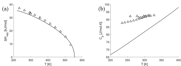
Figure 3. SAFT- \gamma Mie predictive calculations: (a) vaporisation enthalpy \Delta H_{vap} (b) isobaric liquid heat capacity c_p . The symbols correspond to experimental data, sourced from [34,35] for vaporisation enthalpy and [36–41] for isobaric heat capacity. The continuous curves represent the SAFT- \gamma Mie calculations.
