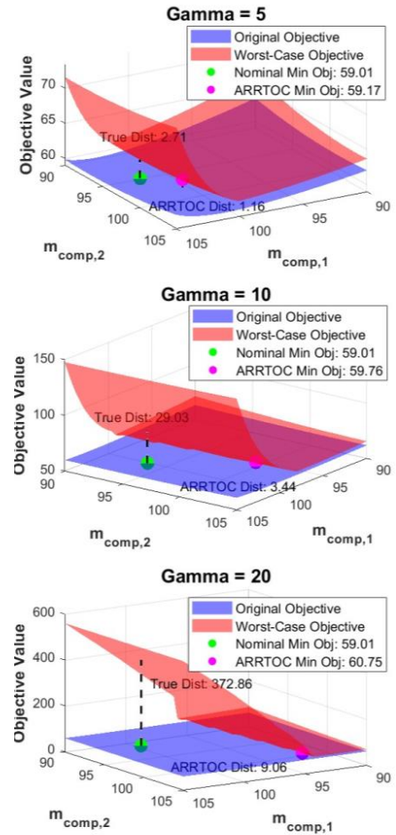
Figure 7. 3D comparison of nominal and worst-case objective functions under varying \Gamma values for the multi-compressor problem
