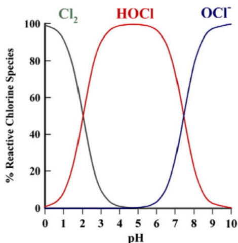
Figure 3: Diagram demonstrating the relationship between pH and the concentrations of hypochlorite and hypochlorous acid in equilibrium.(13)
