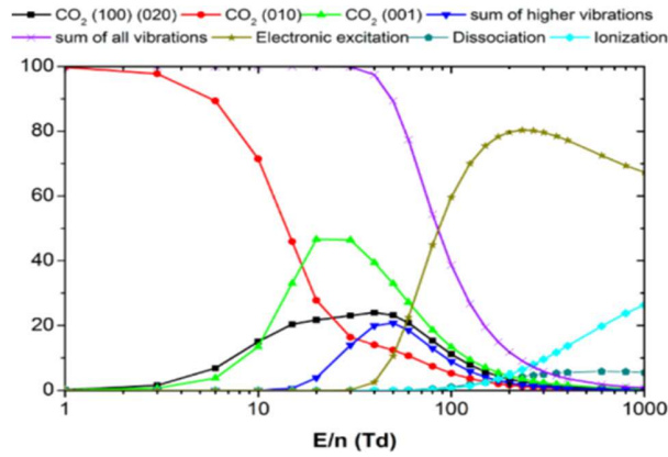
Figure 2. Diagram representing the relative abundance of CO 2 excitation states against reduced electric field strength (Aerts et al.). 14
