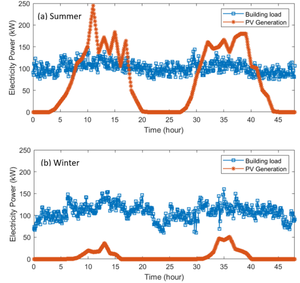
Figure 2: The Building load and PV generation profiles of the sampled two days during (a) summer and (b) winter
