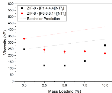
Figure 3.2.3: Viscosity (cP) against mass loading(%) trend for ZIF-8-[P 1,4,4,4 ][NTf 2 ] , ZIF-8-[P 6,6,6,14 ][NTf 2 ] dispersions with comparison to theoretical predictions derived from the Batchelor equation
