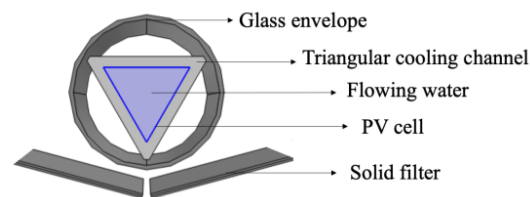
Figure 1.2 Schematic diagram of the top channel
