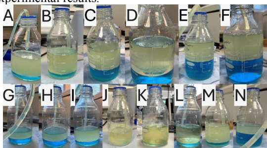
Figure 13. Flowmeter tests with Various Conditions. A–F show the water and oil levels in the flowmeter test at flow rates of 2.5, 5, 7.5, 10, 15, and 20 rpm, respectively. G–J display the water levels at mixing rates of 500, 300, 200, and 100 rpm, respectively. K demonstrates the oil-water separation under the optimized path: 10 rpm, 5 rpm, and 2.5 rpm, with stirring maintained during the 2.5 rpm phase. L shows the water and oil levels under the same conditions as K but without stirring, while M represents the levels with continuous stirring across all states. N provides a comparison, showing the water level at 10 rpm with stirring for an unmodified PU sponge.
