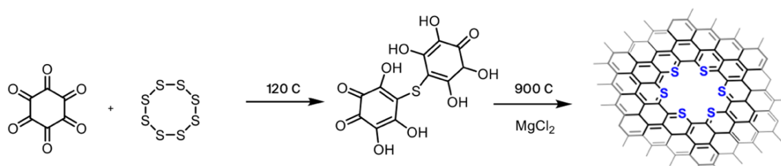
Scheme 1: Reaction scheme of making sulfur based carbon materials.
