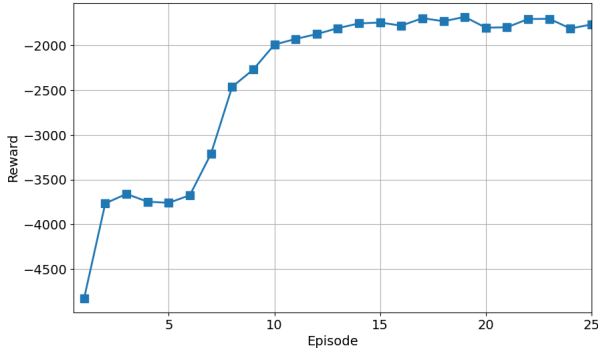
Figure 6: Learning curve for DDPG in energy environment, with window length = 5.
