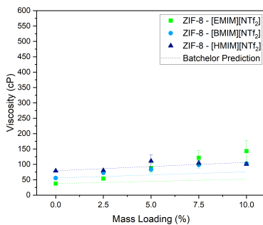
Figure 3.2.1: Viscosity (cP) against mass loading(%) trend for ZIF-8-[EMIM][NTf 2 ], ZIF-8-[BMIM][NTf 2 ] and ZIF-8-[HMIM][NTf 2 ] dispersions with comparison to theoretical predictions derived from the Batchelor equation
