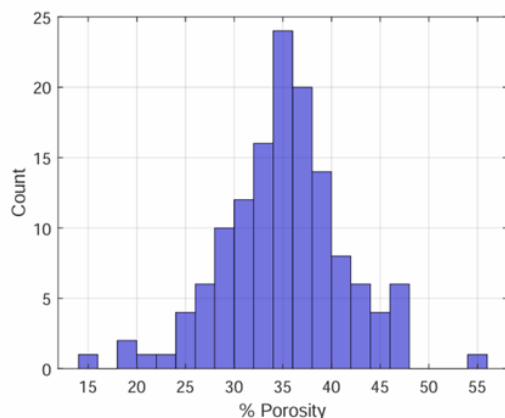
Figure 11. Histogram distribution of microporosities on a grain-by-grain basis for the 136 grains
