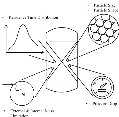
Figure 1.0.1: Outline of the four non-ideal reactor behaviors in commercial scale
