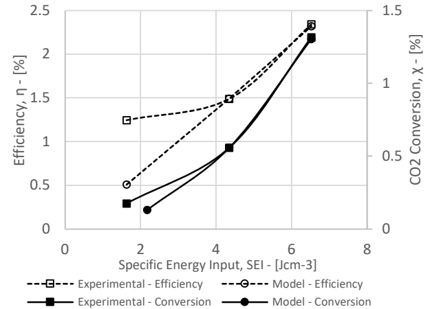
Figure 8. Plots of conversion and efficiency against increasing specific energy input, contrasting model performance (circle markers) against experimental data (square markers). Dashed lines are polynomial fits to the efficiency data (white markers) [%]. Solid lines are polynomial fits to the conversion data (black markers) [%].
