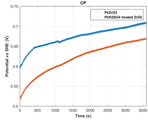
Figure 5. CP curves of ZrO 2 and H 2 SO 4 -treated ZrO 2 under a constant current of 100mA.
