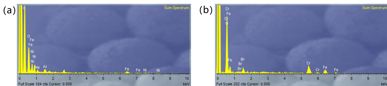
Figure 11. Energy Dispersive X-ray Analysis(EDS) of carbon products after STA. (a) SEM image from Experiment 1 (b) SEM image from Experiment 2
