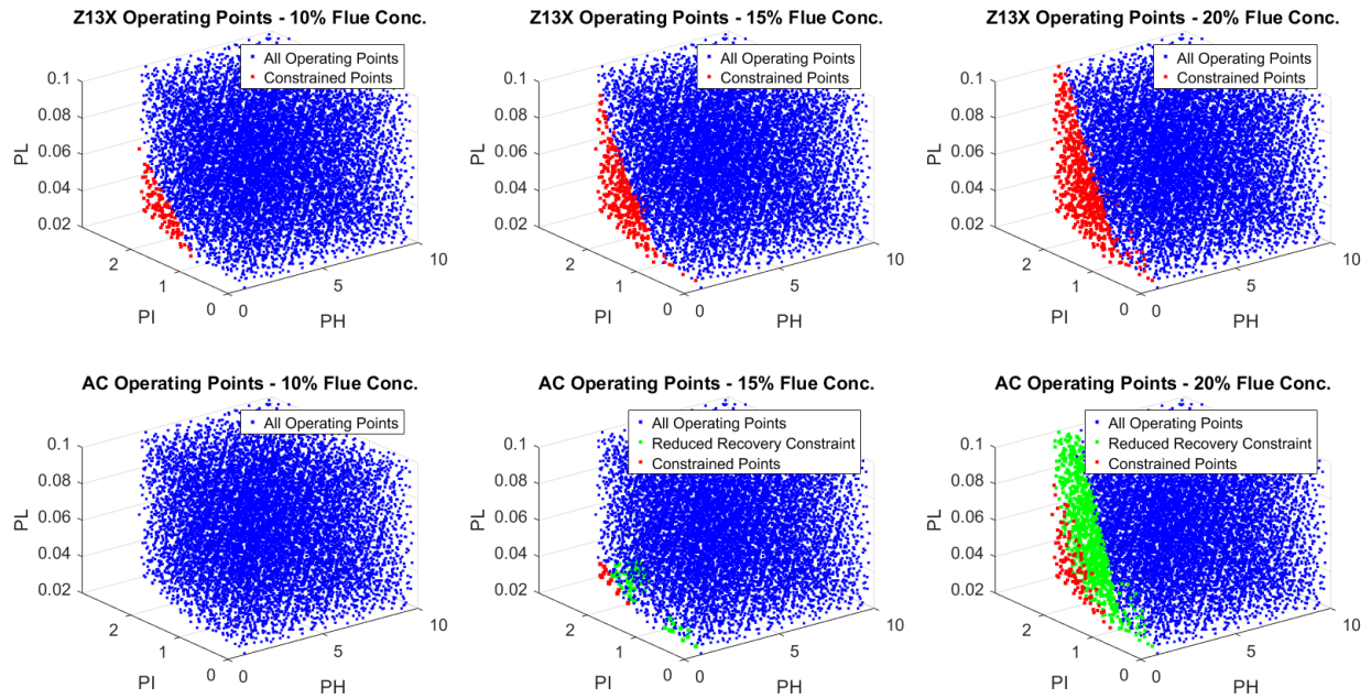
Figure 5. Z13X (top) and AC (bottom) performance at varying flue gas compositions
