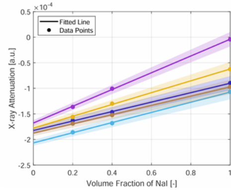
Figure 10. X-ray attenuation against volume fraction of NaI for 5 out of 570 pores plotted from Matlab
