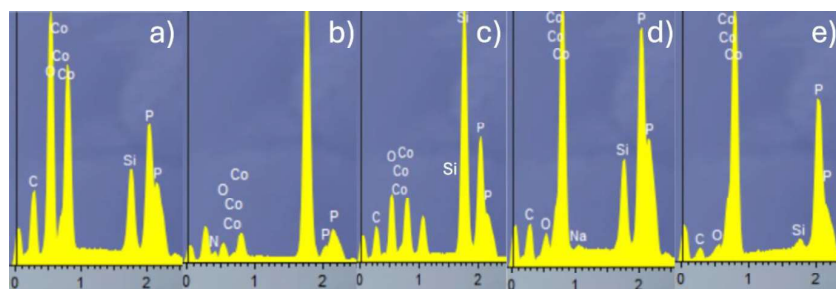
Fig. 8a-e: EDX spectra of a) \text{CoP}_x ( \text{CoCl}_2 ), b) \text{CoP}_x ( \text{Co}_3\text{O}_4 ), c) \text{CoP}_x@\text{C} (ZIF-67), d) \text{CoP}_x (Co-Co-PBA NCs), e) \text{CoP}_x ( \text{Co}_3(\text{PO}_4)_2 )
