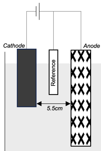
Figure 1: Schematic of Electrolysis Set Up.
