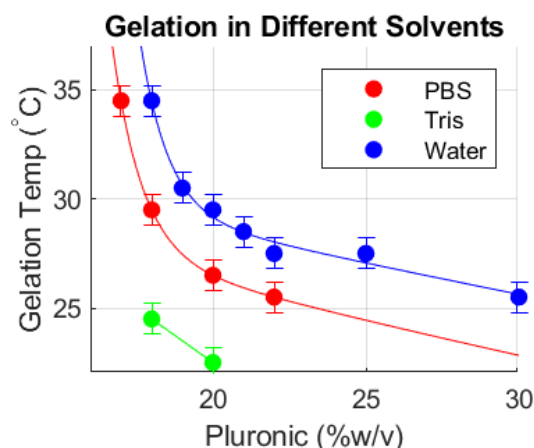
Figure 4. Gelation temperature of Pluronic in various solvents
