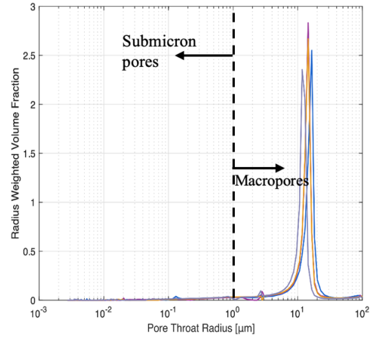
Figure 5. Bentheimer pore throat size distribution obtained through Mercury Injection Capillary Pressure (MICP)
