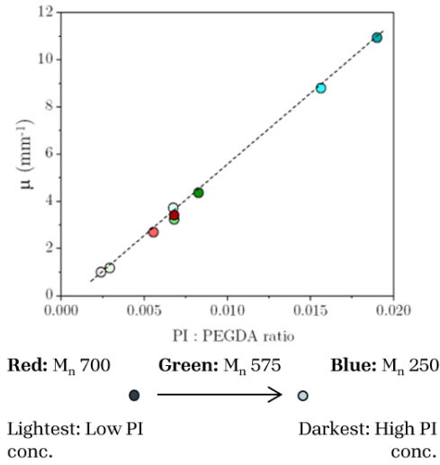
Figure 6: Optical attenuation coefficient ( \mu ) as a function of PI:PEGDA mass ratio. Data points are colour-coded according to molecular weight: red ( M_n=700 ), green ( M_n=575 ) and blue ( M_n=250 ). Marker darkness indicates the PI concentration, with darker shades representing higher PI concentrations. A linear trend is seen; as PI mass concentration increases, the light attenuation increases linearly.
