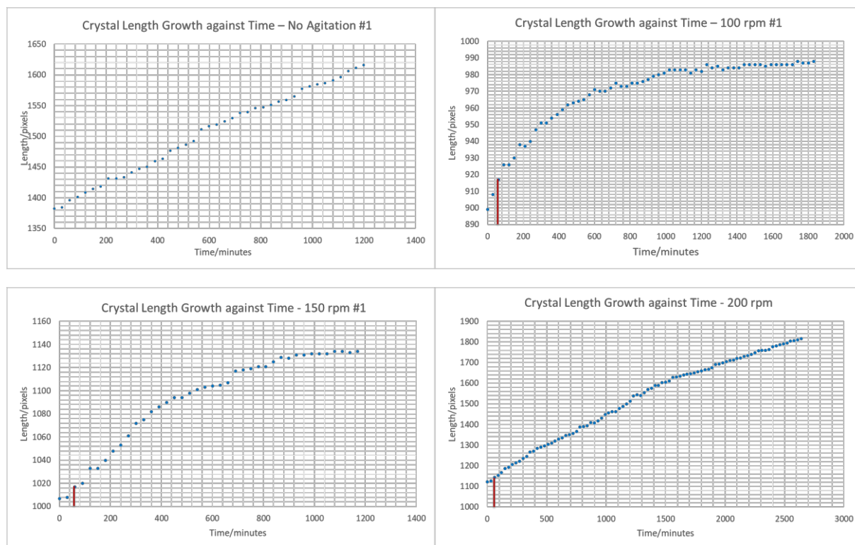
Figure 8-11 - Length against time for first run at 0 rpm (8, top-left), 100 rpm (9, top-right), 150 rpm (10, bottom-left), and 200 rpm (11, bottom-right). The red line indicating when secondary nucleation began.
