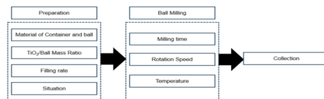
Figure 4: Ball milling steps and parameters
