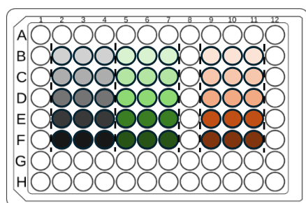
Figure 3. Example of the layout of a 96-well plate used in the encapsulation experiment. Wild Type (grey) is depicted from columns 2-4, GFP (green) in columns 5-7 and mCrimson (red) in columns 9-11. The gradient for each colour represents the methanol concentration beginning at 0% for the lighter shades progressing to 0.5%, 1%, 2% and 3% for the darkest shade. 3% methanol was tested too for further verification of results.
