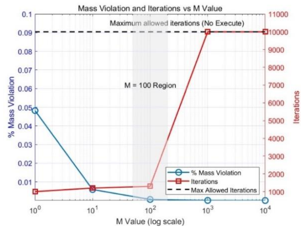
Figure 5. Mass violation and number of iterations versus M value at \Gamma = 0.6 (log scale)
