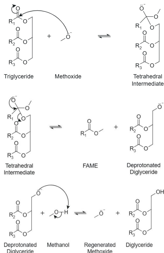
Figure 5: Reaction Mechanism for Methanolysis of Triglycerides. Adapted from Jr et al. (2018).
