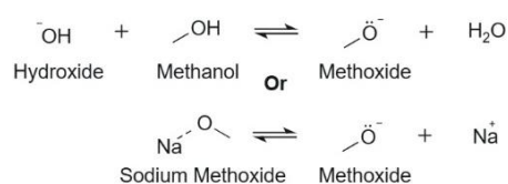
Figure 4: Methoxide Nucleophile Formation. Adapted from Pullen and Saeed (2015).
