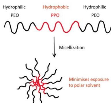
Figure 2. Pluronic structure and micellization
