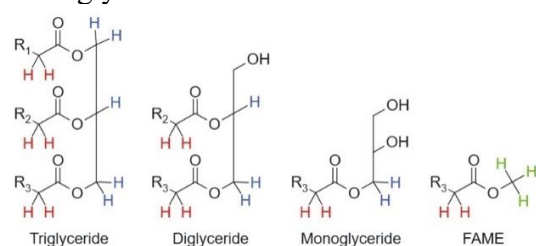
Figure 8: Hydrogen Environments in Reactants, Intermediates and Products.
