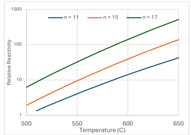
Figure 4.2: Relative reactivity based on temperature and chain hydrocarbon chain length
