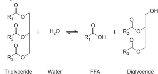
Figure 7: Hydrolysis of Triglycerides. Adapted from Pullen and Saeed (2015).
