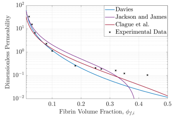
Figure 4. Log-linear plot of dimensionless fibrin permeability functions – Davies' equation (blue), Jackson and James' (purple), and Clague et al.'s (red) – and experimental data (cross) of Wufsus et al. [20-24].
