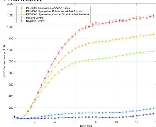
Figure 4.5.1 GFP Fluorescence Over Time for Different Additive Combinations in a Cell-Free System with the AAAAAA Kozak Sequence
