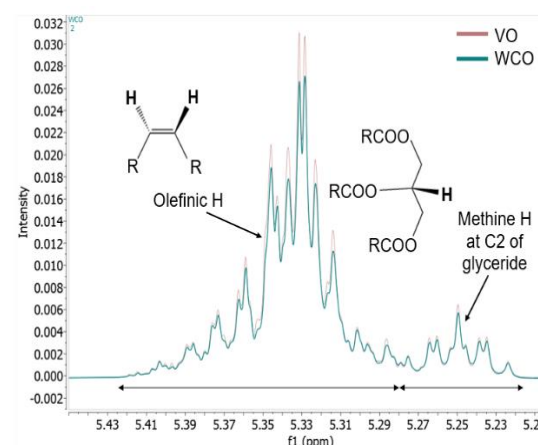
Figure 1 Section of NMR spectrum of VO and WCO showing the olefinic H and C2 glyceride Methine H peaks and the range integrals were calculated
