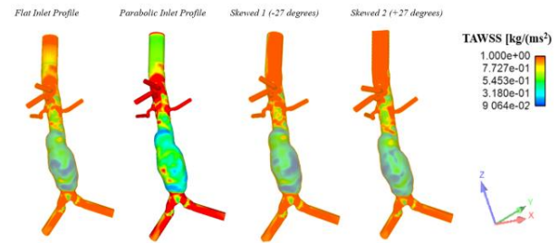
Figure 14 Images of the aneurysm section, highlighting TAWSS for flat (left), parabolic (left centre), skewed 1 (right centre) and skewed 2 (right) inlet velocity profiles
