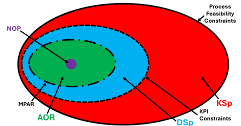
Figure 4: Venn diagram showing the hierarchical relationships between the KSp, DSsp and AOR. The red KSp is created by varying DDs within feasible ranges, bounded by process constraints given by the solid black boundary around the KSp. The blue DSsp, a subset of the KSp, is formed by applying KPI constraints given by the black dashed boundary around the DSsp. The green AOR, centred around a specified NOP in purple, is bounded by the MPAR given by the black dotted boundary around the AOR.
