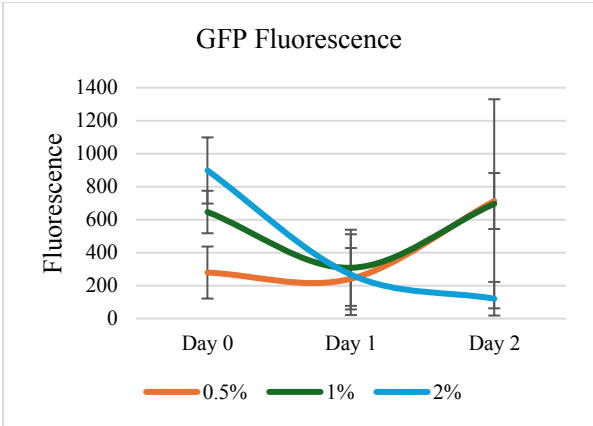
Figure 14. Line graph representing GFP fluorescence for encapsulated Pichia – note smaller values as these readings are relative due to alginate beads. Long overlapping error bars support high invariability and statistical insignificance found with T-tests in table 1 .
