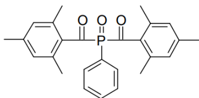
Figure 1: Molecular structure of Irgacure 819, the photoinitiator used in experiments [13]. It induces a high polymerisation initiation rate due to the generation of highly reactive phosphinoyl radicals upon UV exposure, which then go on to react with the acrylate double bonds in PEGDA [14].
