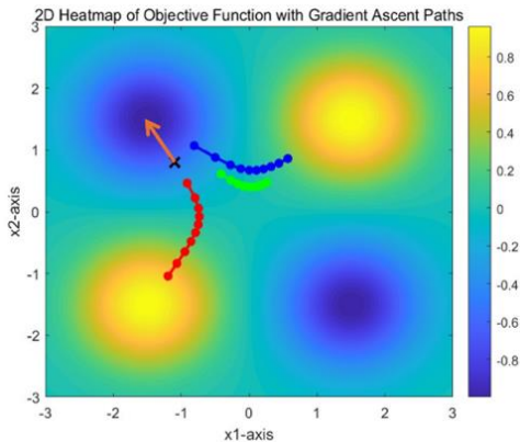
Figure 3. Visual illustration of gradient ascent search paths
