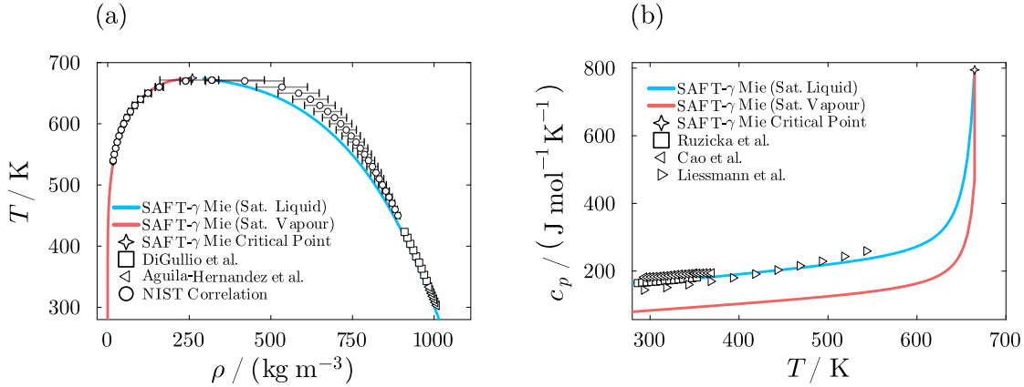
Figure 3: SAFT- \gamma Mie predictions for MEA: (a) temperature-density VLE envelope and (b) isobaric heat capacity as a function of temperature. The SAFT- \gamma Mie critical point is represented by a star marker in both cases. Experimental data [32–36] is shown using unfilled markers, including data from a NIST correlation used for validation at high temperatures in (a).
