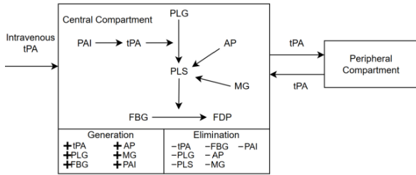
Figure 1. Two-compartment systemic PKPD model.
