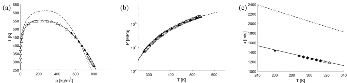
Figure 2. SAFT- \gamma Mie calculations for pure acetonitrile alongside data used in parameter estimation: (a) vapour-liquid coexistence density \rho_{sat} (b) vapour pressure P_{vap} (c) liquid speed of sound u . The open symbols correspond to experimental data not used in parameter estimation, sourced from [23] for saturated vapour density, [23,28–30] for saturated liquid density, [24,31] for vapour pressure and [25,32,33] for speed of sound. The filled upwards pointing symbols correspond to experimental data used in parameter estimation for both the associating and non-associating models, sourced from [23] for saturated liquid density and [24] for vapour pressure. The filled downward pointing symbols correspond to experimental speed of sound data used in fitting the associating model only, sourced from [25]. The dashed curves represent SAFT- \gamma Mie calculations with the non-associating model and the continuous curves represent those with the associating model.
