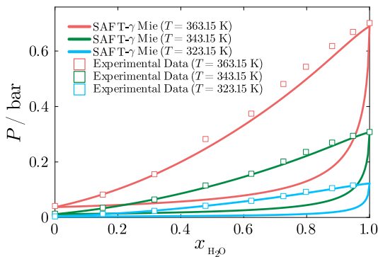
Figure 4: Isothermal pressure-composition slices of the vapour-liquid equilibria for a binary mixture of MEA + H 2 O. Experimental data [39] is shown using unfilled square markers.
