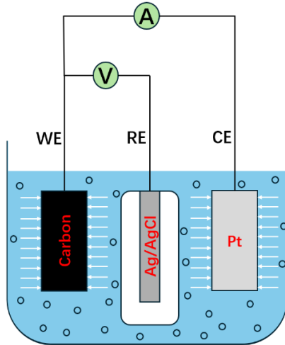
Figure 2. Electrodeposition and GCD test experimental lay-out.
