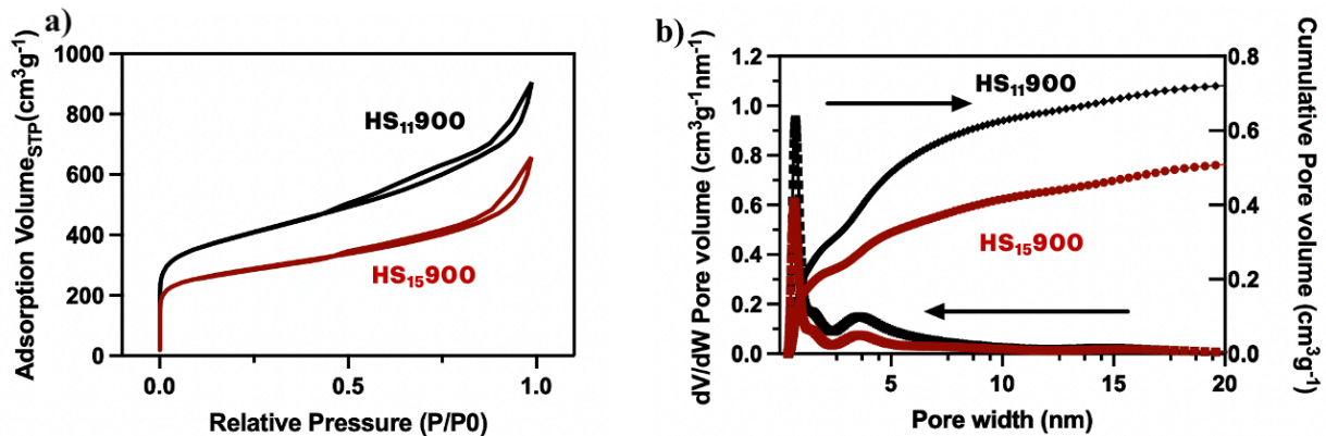
Figure 3. Nitrogen sorption isotherms with labelled BET specific surface areas (a) and the corresponding pore size distributions and cumulative pore volumes, calculated using the 2D-NLDFT heterogeneous surface carbon model in SAIEUS software (b) for the sample HS 11 900 and HS 15 900.
