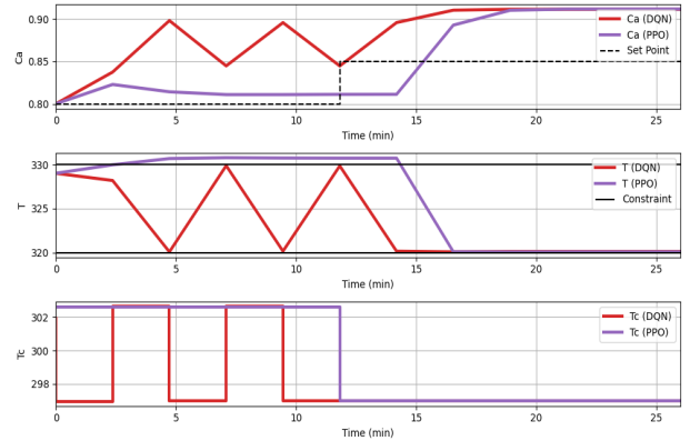
Figure 5: Constrained RL trajectories
