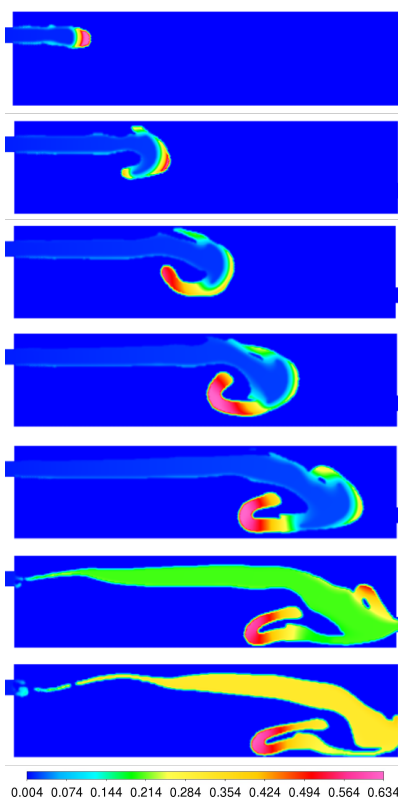
Fig. 10: Viscosity contour maps for transient blood flow in units of [kg/m/s] varying with time for a 1 mm mesh size and 0.01 s time-step.
