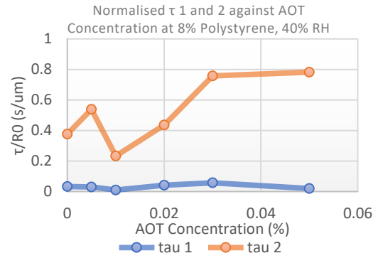
Figure 6 Key drying profile parameters normalised by initial radius ( R_0 ) and characterised against surfactant concentrations.
