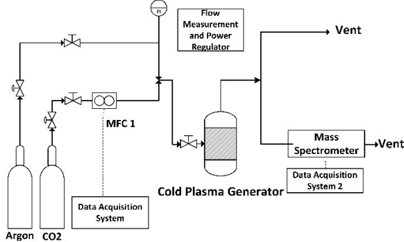
Figure 6 PFD of experimental set-up
