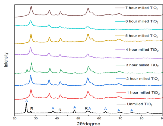
Figure 10: XRD results of milled \text{TiO}_2 samples
