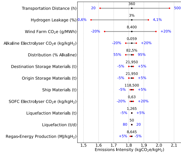
Figure 6. OVAT sensitivity analysis results demonstrating the impact of varying each parameter individually on the overall CO 2 e intensity of the green hydrogen supply chain.
