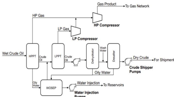
Figure 1: Block flow diagram of a gas-oil separation facility (GOSP) showing how crude oil, natural gas and water are separated (Bahamdan et al., 2024)
