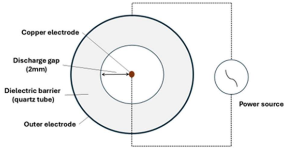
Figure 5 Bird-eye cross-sectional view of the DBD reactor
