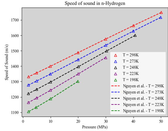
Figure 6: Speed of sound in n-hydrogen against pressure
