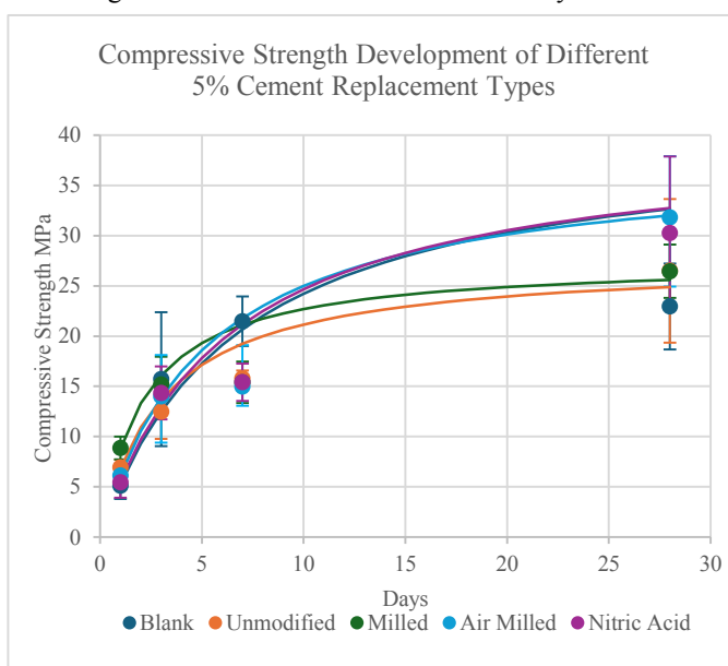
Figure 3. Compressive Strength Development Over 28 Days.
