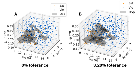
Figure 6: Initial DSps with 512 points used as input into DSp identification program, A: DSp obtained with 0% tolerance this results in 4 disjointed regions, B: DSp obtained with 3.20% tolerance this results in 1 unified region.
