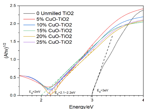
Figure 14: Tauc plots of milled (Above) and doped (Below) TiO 2 samples
