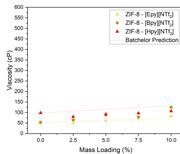
Figure 3.2.2: Viscosity (cP) against mass loading(%) trend for ZIF-8-[Epy][NTf 2 ], ZIF-8-[Bpy][NTf 2 ] and ZIF-8-[Hpy][NTf 2 ] dispersions with comparison to theoretical predictions derived from the Batchelor equation
