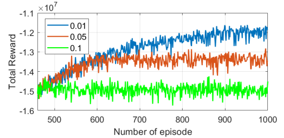
Figure 9: Reward analysis of minimum epsilon \epsilon_{min} , with fixed export penalty c_e of 0.55 and fixed cost coefficient w_1 of 80, trained through 1000 episodes
