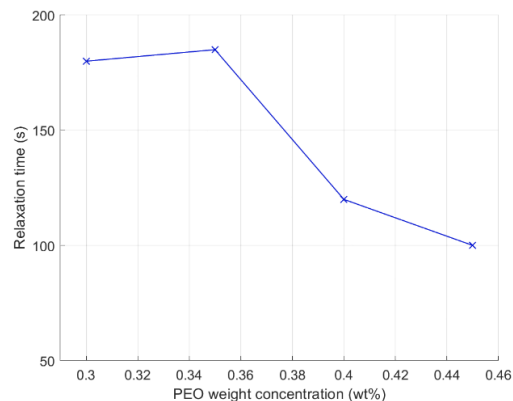
Figure 4.3 – Relaxation time (taken as time for viscosity gradient to reach zero) for LUDOX TM-50 gels compared with PEO concentration.
