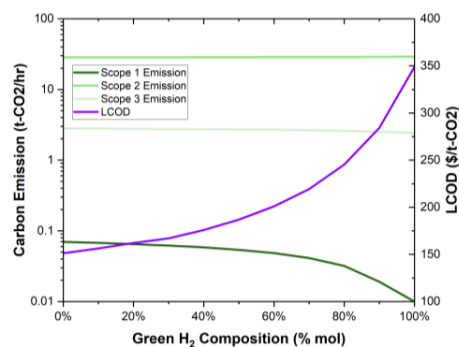
Figure 10. Carbon emission for green H 2 scenarios
