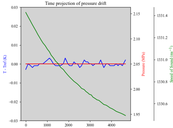
Figure 10: Time series data for n-hydrogen measurement at T = 298\text{K} and P = 2\text{ MPa}
