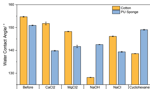
Figure 16. Water Contact Angle after Chemical tests
