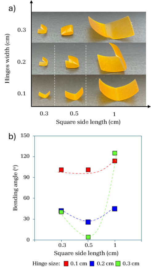
Figure 10: (a) Grid of hinge images with varied hinge and face dimensions. 0.1, 0.2 and 0.3 cm hinges with 0.3, 0.5 and 1 cm square side length faces are tested. Different bending regimes are observed: controlled, gravity-dominant and gravity failure (b) Bending angles of hinges seen in Figure 10a (°) with square side length (cm). Data points are colour-coded according to hinge size: red (0.1 cm), blue (0.2 cm), green (0.3). 0.1 and 0.2 cm hinges show little variation in bending, 0.3 has no observable trend.
