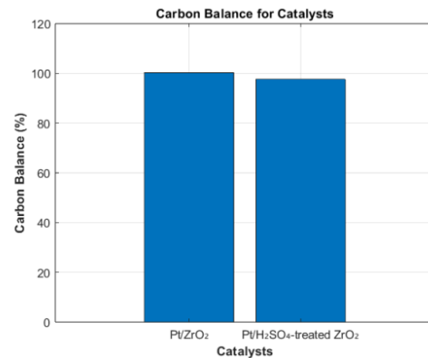
Figure 7. Carbon balance of Pt/ZrO 2 and Pt/H 2 SO 4 -treated ZrO 2 in MEA setup.
