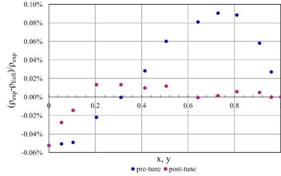
Figure 12 (b). Deviation of literature density data in toluene-cyclopentane mixture from the EoS predictions against toluene composition before and after parameters tuning
