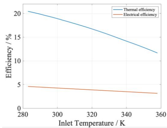
Figure 4.3. Effect of varied inlet temperature on top channel efficiencies. A rise in inlet temperature causes reductions in thermal and electrical efficiency.
