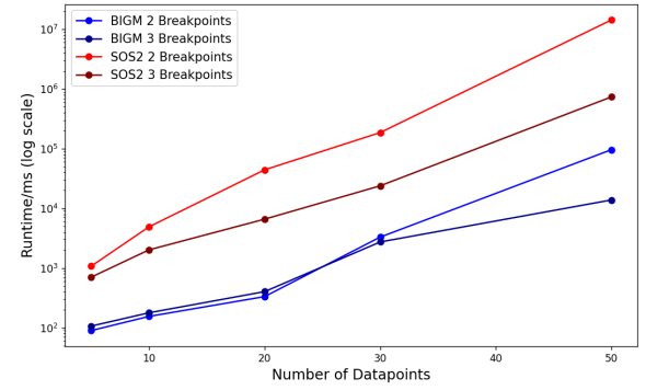
Figure 4: Runtime comparison - Big M and SOS2
