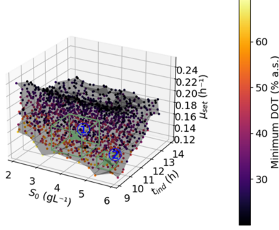
Figure 11: Nominal operating points within the design space.
