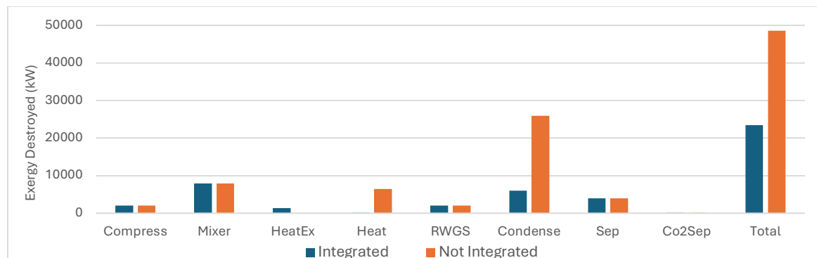
Figure 3.2: Comparison bar charts for final exergy analysis on heat integrated and non-integrated flowsheet
