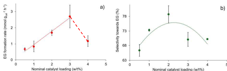
Fig 5a-b: MTEG a) activity and b) selectivity of \text{CoP}_x\text{@C} (ZIF-67)/CdS catalysts with variable \text{CoP}_x\text{@C} loadings.
