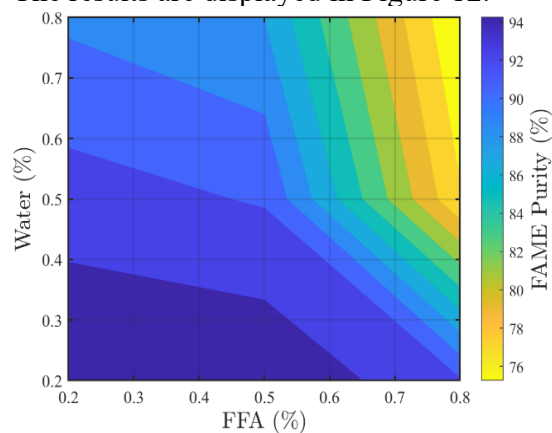
Figure 12: Combined Effect of FFA and Water Impurities on Biodiesel Purity.
