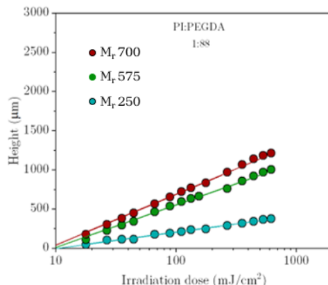
Figure 5: Variation of polymerised height as a function of irradiation dose on a log scale for 1:88 PI:PEGDA mol/mol ratio. Solid lines indicate linear fits to the data. The plot shows a logarithmic increase in height with higher irradiation doses. The rate of this change of height with dosage increases with PEGDA molecular weight. For comparison of M_n solution solutions at other PI concentrations see Supplementary Information Section 2.1.
