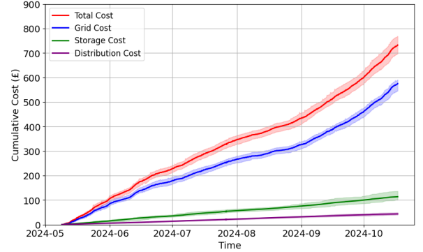
Figure 7: DDPG mean cumulative costs for 10 prosumers.
