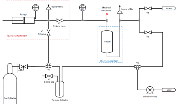
Figure 3. Process flow diagram of the apparatus involved
