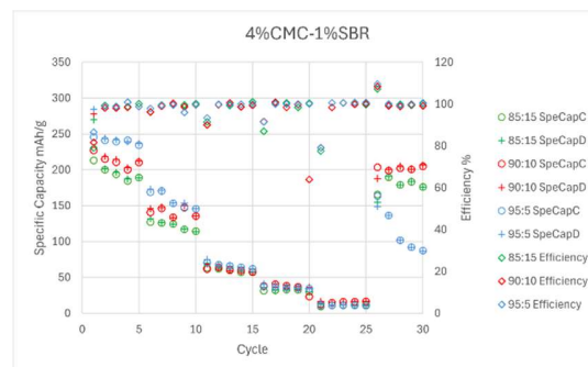
Figure 4.2-3: Cycle vs. Specific Capacity & Efficiency Graph for 4% CMC: 1% SBR
