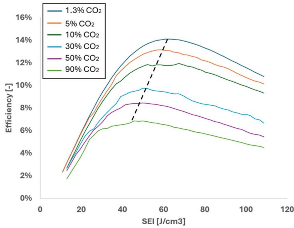
Figure 10. Plots of efficiency against increasing specific energy input, determined via model sensitivity analysis, varying the initial CO 2 mol fraction. The dashed black line crests the locus of stationary points, delineating the maximum efficiencies at each mol fraction. Decrease in critical SEI (obtained at peak efficiency) with increases CO 2 fraction is effected by the increasing collision cross section detailed in section 6.3
