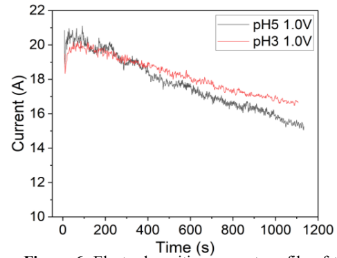
Figure 6. Electrodeposition current profile of the carbon paper under 1.0V applied potential at different pH.
