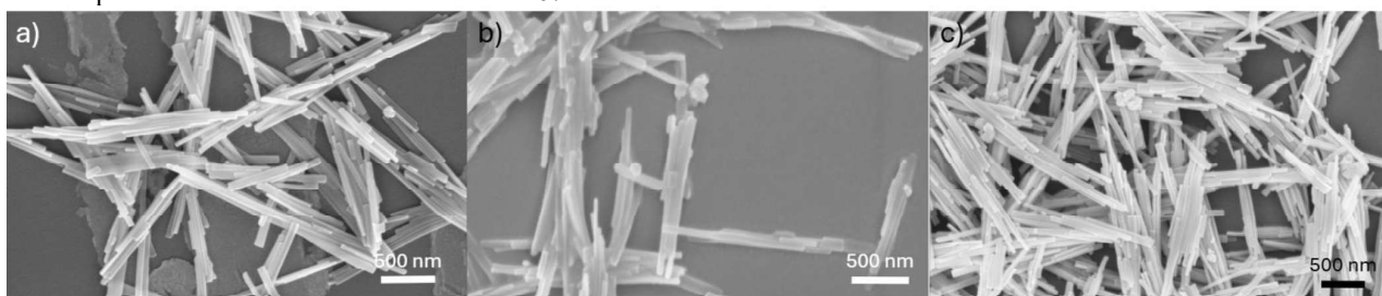
Fig. 9a-c: SEM of a) CoP_x@C (ZIF-67)/CdS 1 w/t%, b) CoP_x@C (ZIF-67)/CdS 3 w/t% and c) CoP_x@C (ZIF-67)/CdS 4 w/t%.
