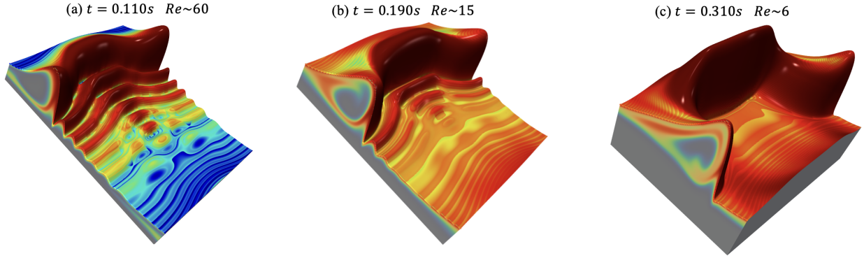
Figure 3: DNS results for a) case 1a, b) case 2a, and c) case 3a, for normalised global concentration of \text{CO}_2 in liquid film at \sim 0.2 .
