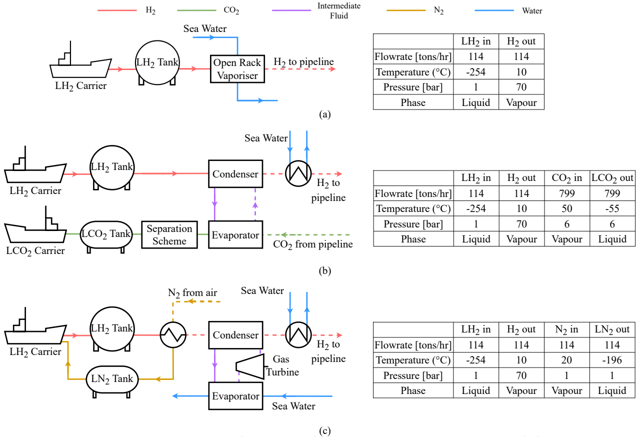
Figure 1: Block flow diagrams and stream tables for a) the base case (using of an open-rack vaporiser to regasify H 2 ) b) a dual-use LH 2 import / CO 2 export terminal c) a dual-use LH 2 import / N 2 export terminal
