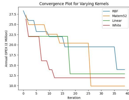
Figure 3: Annual Operational Expenditure (OPEX) convergence plot for Bayesian optimisation given different kernels: Radial Basis Function (RBF), Matern52, Linear and White
