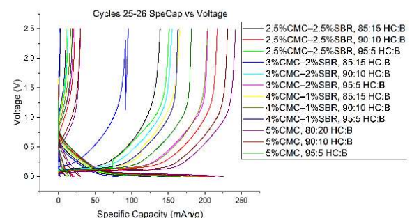
Figure 4.1-6: Specific Capacity vs. Voltage Graph for Cells of Different Composition from Cycle 25-26
