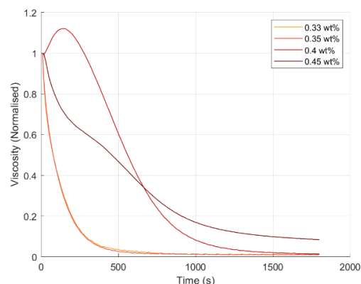
Figure 4.4 – Normalised viscosity against time for CS50-28 gels of different PEO concentrations during relaxation.
