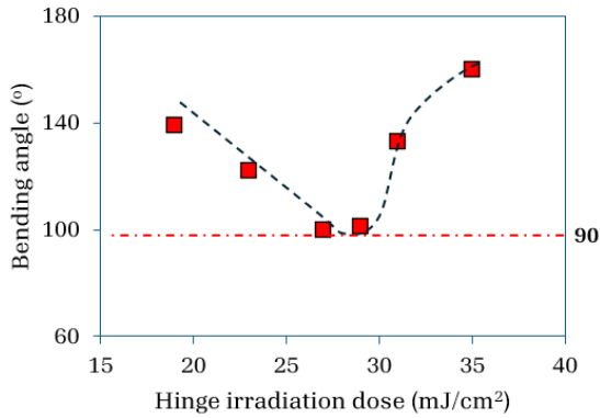
Figure 9: Variation in bending angle of hinge (°) with hinge dosage (mJ/cm 2 ). The dosage applied to the face is kept constant at 90 mJ/cm 2 . A 90° angle is met at 29 mJ/cm 2 and this dosage is taken as the optimum. Either side of this the hinge flattens, due to dominant effect of gravity.
