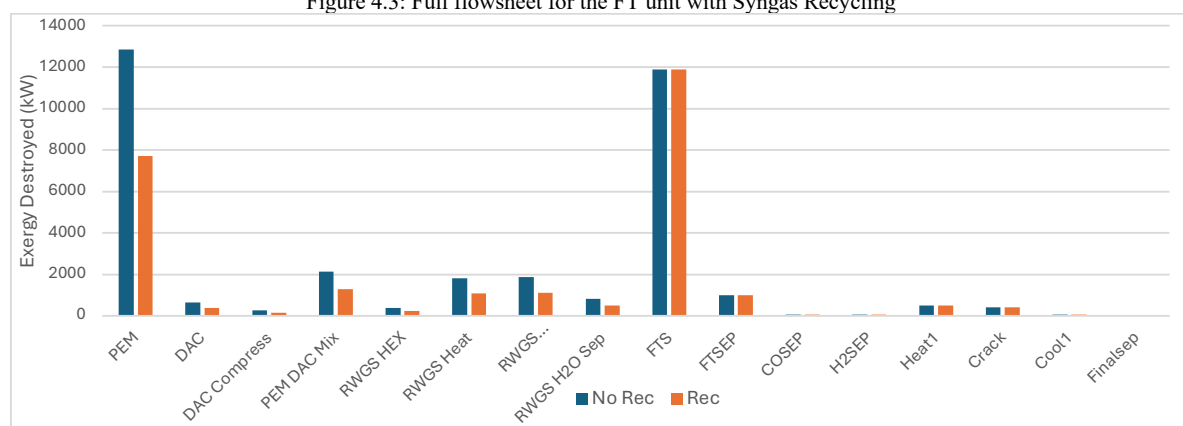
Figure 4.4 Exergy destroyed per tonne of SAF produced of whole integrated process depending on FT recycling
