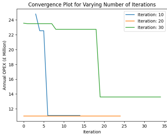
Figure 5: Annual Operational Expenditure (OPEX) convergence plot for Bayesian optimisation given different number of iterations: 10, 20, 30 (excluding initial sampling)
