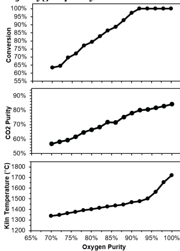
Figure 3 Effect of oxygen purity on conversion, CO 2 purity and kiln temperature.
