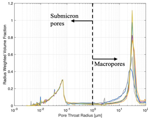
Figure 4. Ketton pore throat size distribution obtained through Mercury Injection Capillary Pressure (MICP)
