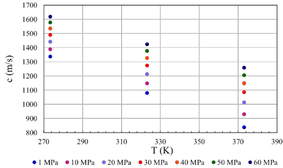
Figure 5. Sound speed against temperature in pure cyclopentane
