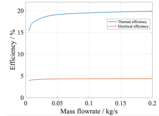
Figure 4.1. Effect of varying mass flowrate on top channel thermal and electrical efficiencies. As mass flowrate increases efficiency increases.
