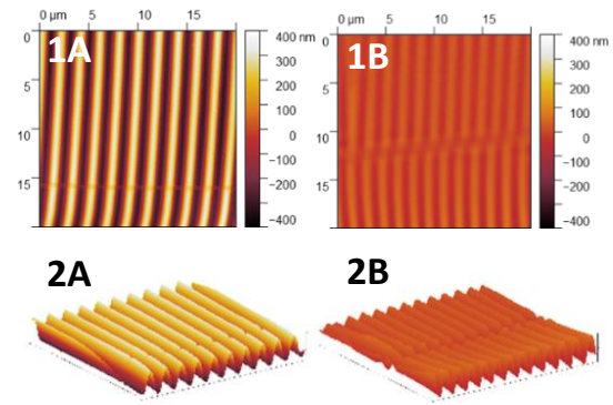
Figure 6: 1A presents the colour topography of a 1.3\mu\text{m} wrinkle before plasma oxidation, with 2A being the 3-Dimensional visualisation of 1A. 1B and 2B are the results after the 1.3\mu\text{m} wrinkle was exposed to plasma for 10 seconds.
