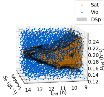
Figure 9: DSp obtained with 4096 points obtained from emulator with a tolerance of 23.91% to obtain a single DSp, with satisfied (Sat) points in orange, violated (Vio) points in blue and the DSp shown in grey.
