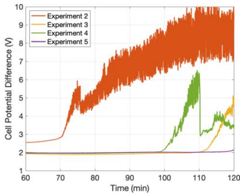
Figure 4. Cell potential difference of all experiments after 1 hour of electrolysis
