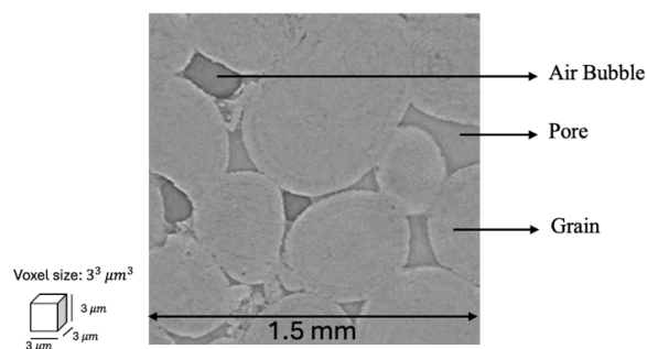
Figure 1. Slice of the extracted sub volume obtained through Avizo, with dimensions of 500 x 500 voxels 2
