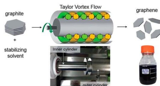
Figure 1 Schematic of exfoliation process and Taylor Vortex Flow Reproduced with permission from Ref. 12. Copyright 2016 The Royal Society of Chemistry.
