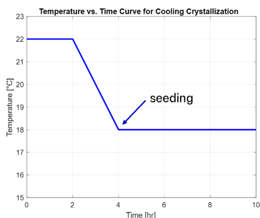
Figure 8 – Cooling profile of mother liquor in cooling regeneration
