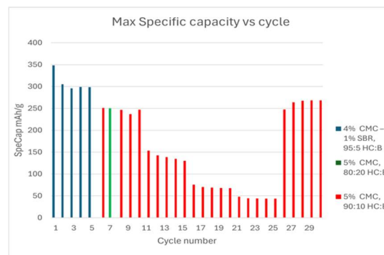
Figure 4.2-5: Cycle Number vs. Specific Capacity Graph
