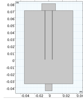
Figure 1: Geometry of the 2D COMSOL model implemented
