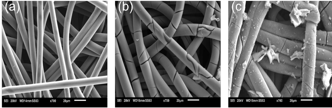
Figure 5. SEM images of carbon paper at x700 magnification: (a) Blank (no electrodeposition) (b) Electrodeposited at 1.0V (c) Electrodeposited at 1.1V.
