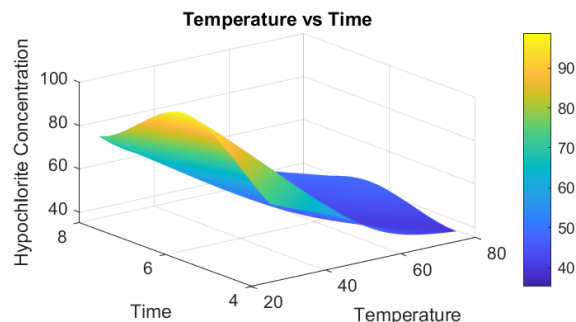
Figure 9: The combined effect of temperature and time on hypochlorite concentration
