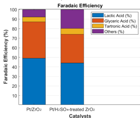
Figure 9. Faradaic efficiency of Pt/ZrO 2 and Pt/H 2 SO 4 -treated ZrO 2 in MEA setup.
