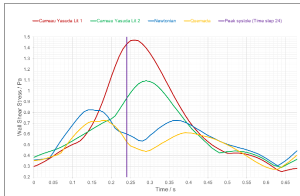
Figure 10.2 Plane 3 maximum WSS as a function of time between all 4 non-Newtonian models
