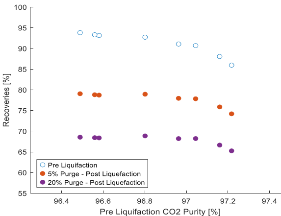
Figure 9. Z13X Recovery Pareto Fronts with varying Purge
