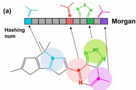
Figure 1 – Morgan Fingerprint Binary Vector Representation [11]
