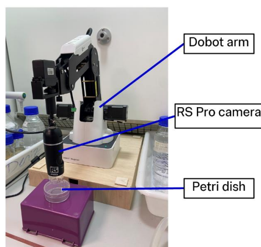
Figure 4 – Dobot rig setup for evaporative regeneration of ethanol-impurity systems.
