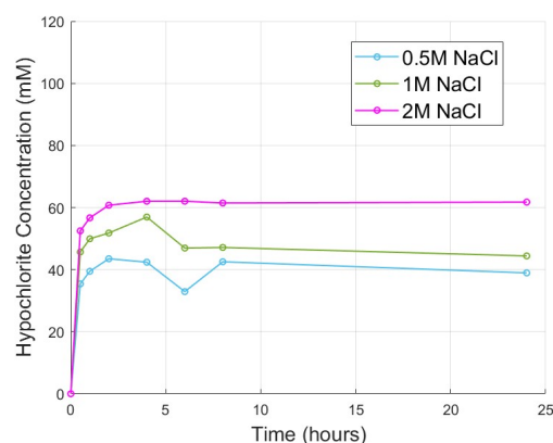
Figure 5: Plot of hypochlorite concentration (mM) over time at 50°C for various initial NaCl concentrations.
