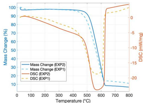
Figure 8. Simultaneous thermal analysis (STA) of Experiment 2
