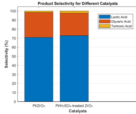
Figure 6. Selectivity towards LA, glyceric acid and tartronic acid in MEA setup.
