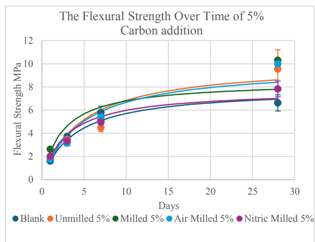
Figure 4. Flexural Strength Development Over 28 Days
