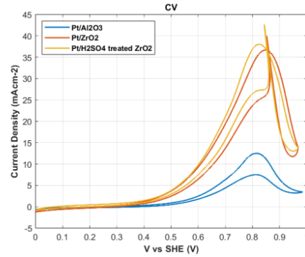
Figure 2. CV curves of Pt-based Al 2 O 3 , ZrO 2 , and H 2 SO 4 -treated ZrO 2 .
