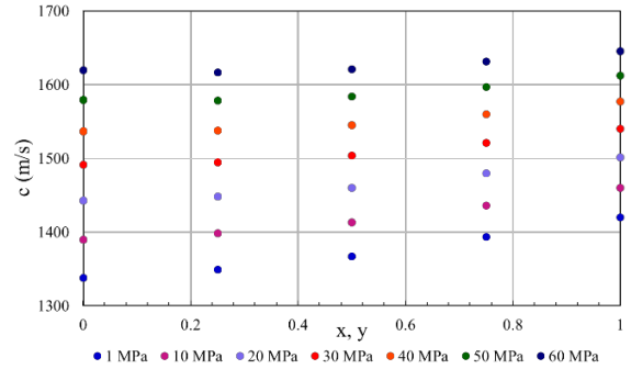
Figure 10. Sound speed in toluene-cyclopentane mixture against toluene composition at constant temperature of 273K
