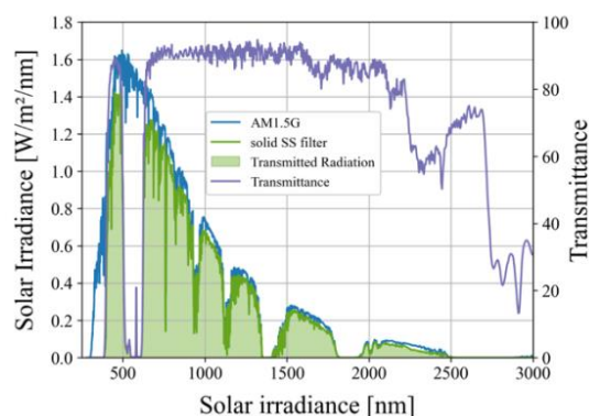
Figure 1.3: AM1.5G spectrum and transmittance profile of the solid SS filter
