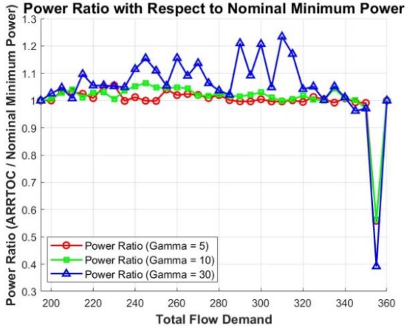
Figure 10. Power ratio relative to nominal minimum power under varying \Gamma values across different total flow demands
