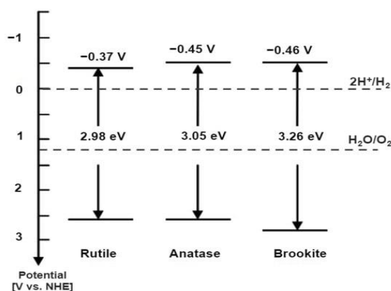
Figure 2: Bandgaps of TiO 2 phases [5]
