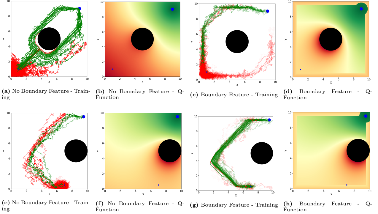
Figure 4: Comparison of training and Q-functions for scenarios 1 (a)-(d) and 2 (e)-(h) with and without boundary features. The small blue circle is the starting location of the agent and the larger blue circle is the goal. The large black circle is the obstacle. In the training plots, green paths denote episodes that ended with the goal being reached, and red paths denote a failed episode. The opacity of the paths increase with later episodes. In the Q-function visualisations, the red to green gradient represents increasing Q-values of the LFA.
