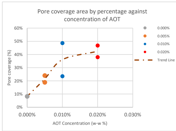
Figure 7 Pore coverage % against concentration change
