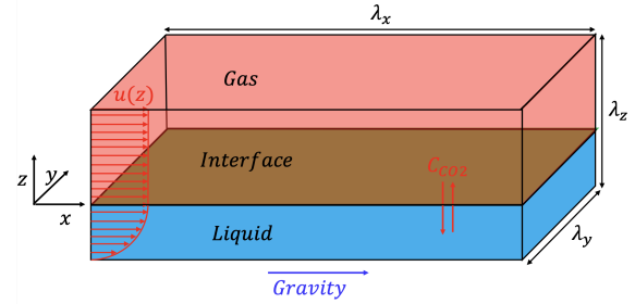
Figure 1: Computational domain of a 3D falling film configuration with gas absorption.
