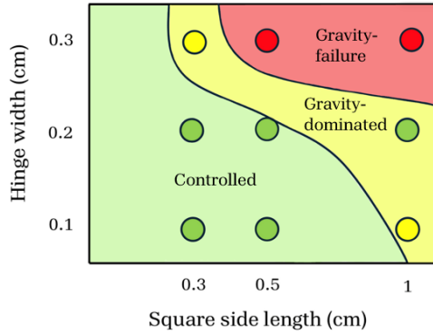
Figure 11: Morphology map representing regions of different bending regimes for hinges of varying dimensions. Circles represent experimental data points (see Figure 10a): green is the controlled regime, yellow is the gravity dominated regime, red is the gravity failure regime. The background colours represented proposed thresholds for each regime.
