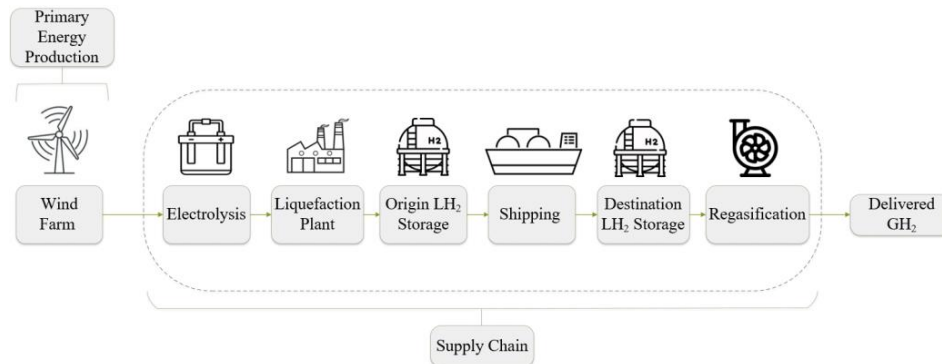
Figure 2. Schematic representation of the green hydrogen supply chain, illustrating the key stages from renewable energy production via wind energy, through electrolysis and liquefaction, to intercontinental shipping and regasification with storage, for delivery of gaseous hydrogen.
