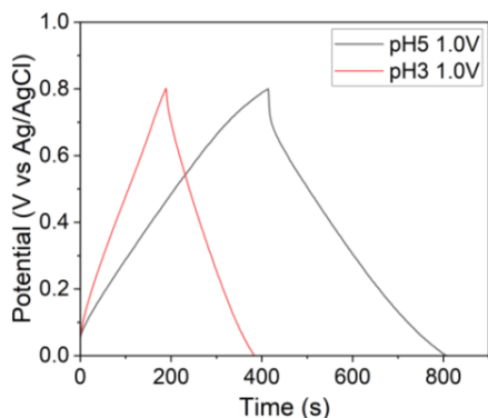
Figure 7. GCD curves compare the charge-discharge performance of the electro-deposited carbon paper under 1.0V at pH3 and pH5 (10 th Cycle).
