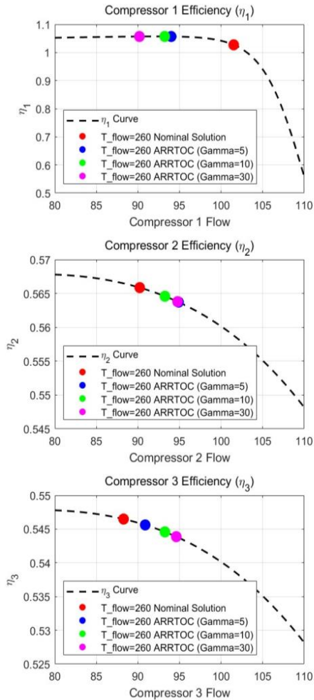
Figure 8. Nominal minimum versus ARRTOC minimum (at varying \Gamma ) shown on the efficiency maps of compressor 1 to 3
