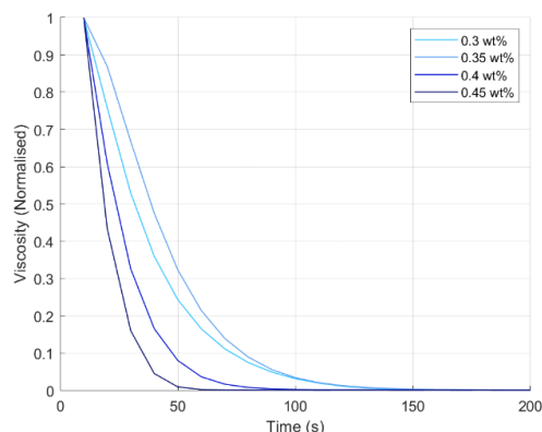
Figure 4.2 – Normalised viscosity for LUDOX TM-50 gels at different PEO concentrations during relaxation under a shear rate of 1 \text{ s}^{-1} .
