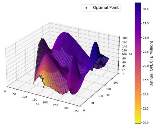
Figure 8: Uses observed data from Bayesian Optimisation (BO) to show how Annual Operational Expenditure (OPEX) changes with (x_1, x_2, x_3) which are crude oil, sour gas and water flowrates respectively. The optimal value for final BO model is (180, 1.67, 42.8) labelled with a red point, given at \epsilon = 200 t_{CO_2} .
