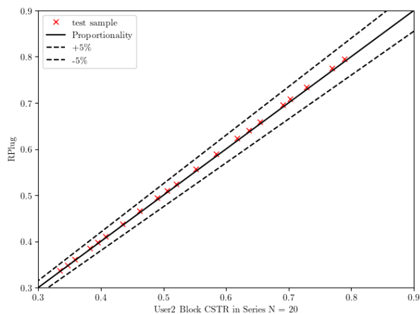
Figure 4.1.2: Parity Plot on Comparing a Set of Results on EC Conversion From a Aspen User2 Block against Aspen RPlug Block
