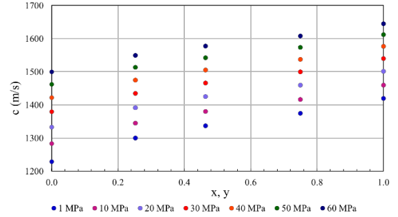
Figure 6. Sound speed in toluene-ethanol mixture against toluene composition at constant temperature of 273K
