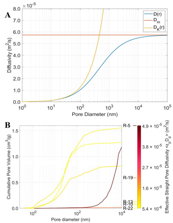
Figure 4: A) Knudsen, molecular and combined diffusivities as a function of pore diameter B) Cumulative PSDs for investigated materials. Colour-coded according to effective straight pore diffusivity.
