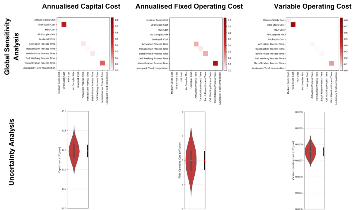
Figure 3.1.1.1 : Global Sensitivity and Uncertainty Analysis on Economic KPIs
