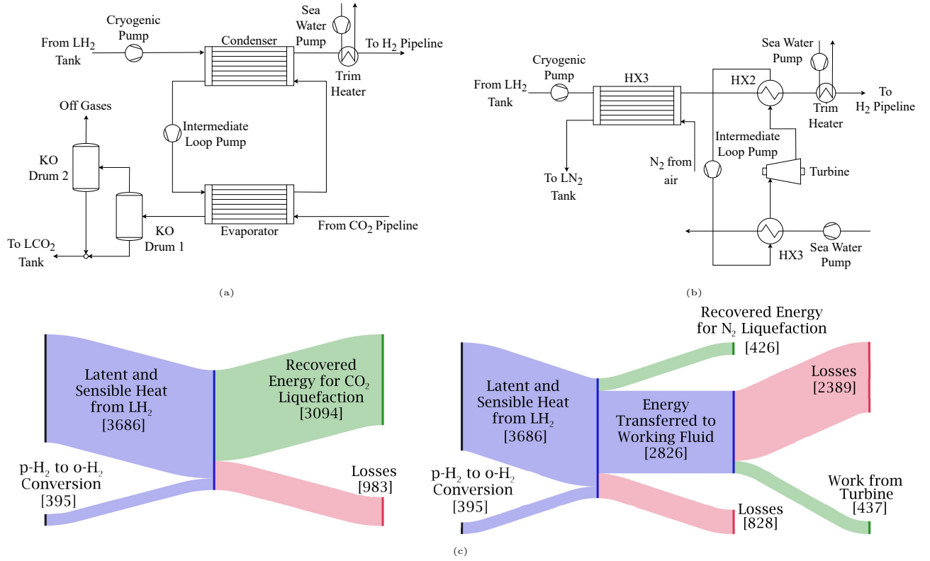
Figure 3: a = Process Flow Diagram of the LH 2 /CO 2 Terminal implemented in Aspen Plus. b = Process Flow Diagram of the LH 2 /N 2 implemented in Aspen Plus. c = Sankey Diagram showing the energy recovery from a) the LH 2 import / CO 2 export Terminal and b) the LH 2 import / N 2 export Terminal. Values in brackets are kJ/kg of H 2
