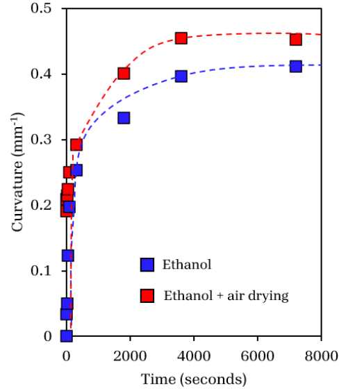
Figure 8: Curvature ( \text{mm}^{-1} ) of polymer sample with changing development procedure. The addition air drying increases the rate of curvature and the extent of curvature after a 7200 second period (2 hours)
