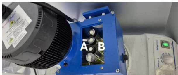
Fig. 3: Photocatalytic reactor setup.
