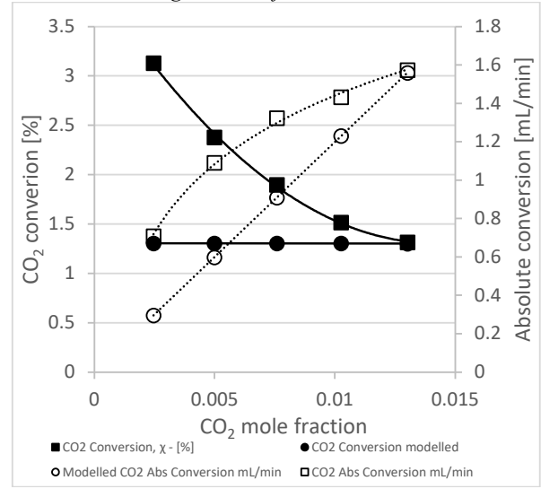
Figure 7. Plots of conversion – percentage and absolute – against inlet CO 2 mol fraction, contrasting model performance (circle markers) against experimental data (square markers). Dashed lines trends the absolute conversion data (white markers) [mL/min]. Solid lines trends the percentage conversion data (black markers) [%].
