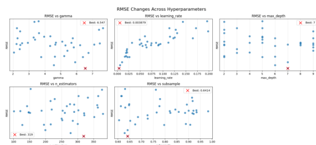
Figure 12 – Scatter plot of RMSE values against hyperparameters. With the red crosses denoting the optimal RMSE values.
