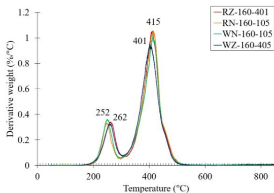
Figure 6 DTA graph showing rate of weight loss from TGA
