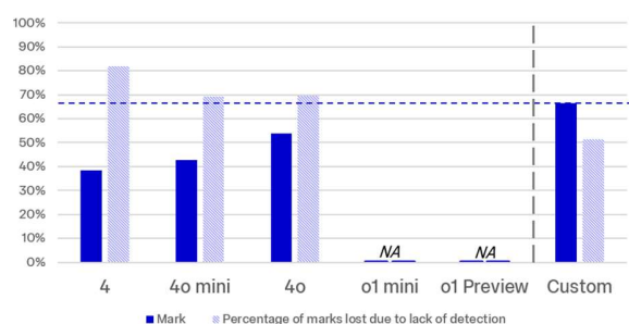
Figure 4.1.1 Image P&ID Recognition Results
