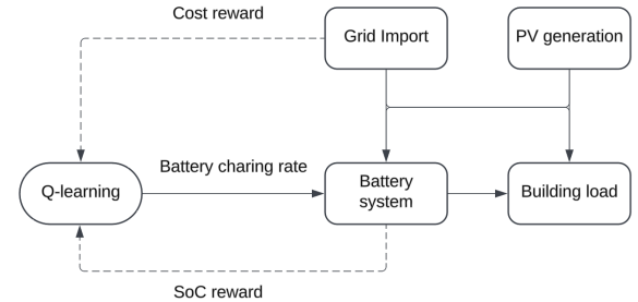
Figure 3: Control logic
