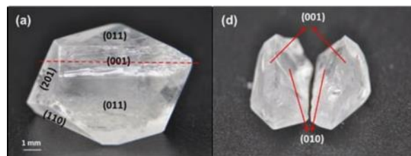
Figure 4 - Macroscopic crystal of monoclinic paracetamol (a) whole crystal, (d) cleaved crystal. (010). Source: [7]
