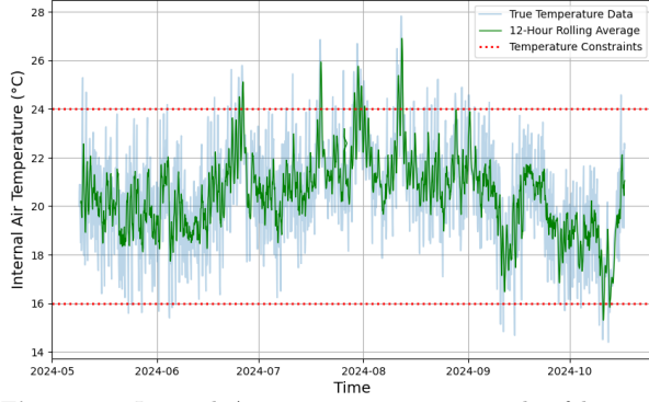
Figure 9: Internal Air Temperature as a result of heuristic based actions.
