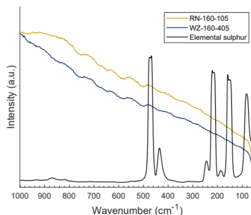
Figure 3 Raman spectrum for elemental sulphur and samples RN-160-105 and WZ-160-405.
