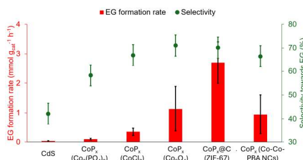
Fig. 4: EG formation rates over CdS modified with various \text{CoP}_x cocatalysts. The compound in brackets represents the precursor used to synthesise the \text{CoP}_x . All cocatalysts were loaded at 3% nominal weight.
