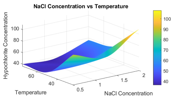
Figure 7: The combined effect of NaCl concentration and temperature on hypochlorite concentration
