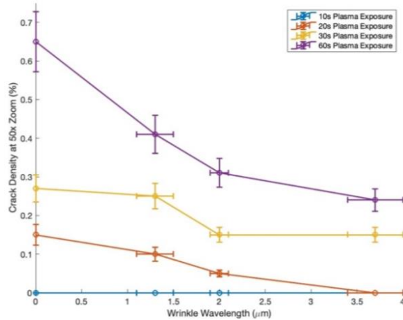
Figure 4: Impact of wrinkle wavelength (ones of \mu\text{m} ) on crack density after various plasma exposure times.
