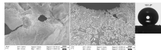
Figure 3. SEM Images of Modified PU Sponge
