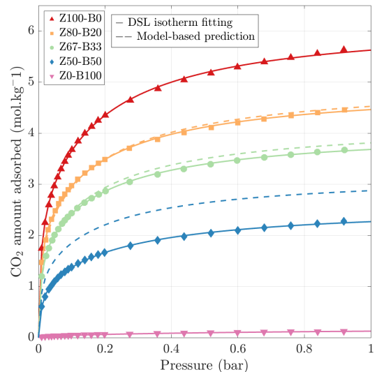
Figure 4: CO_2 adsorption isotherms at 303 K with fitted adsorption isotherms (solid line, DSL model), and model-based predicted adsorption isotherms (dashed line) for Z100-B0, Z80-B20, Z67-B33, Z50-B50, and Z0-B100.
