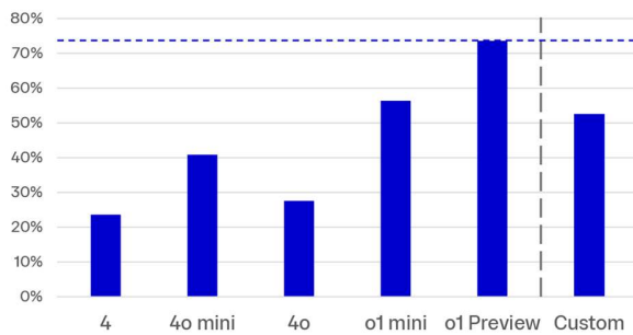
Figure 4.2.2 Average Performance Using Custom Mark Scheme
