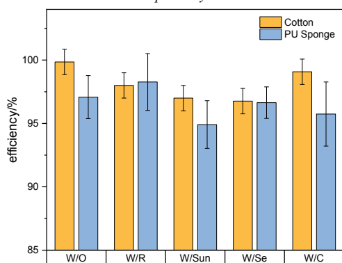
Figure 10. Oil Sorption Efficiency of Vegetable Oil. W represents DI water
