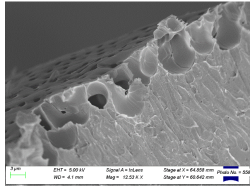
Figure 9 SEM image of the cross-section of the particle, with the skeleton of the water droplet array visible.
