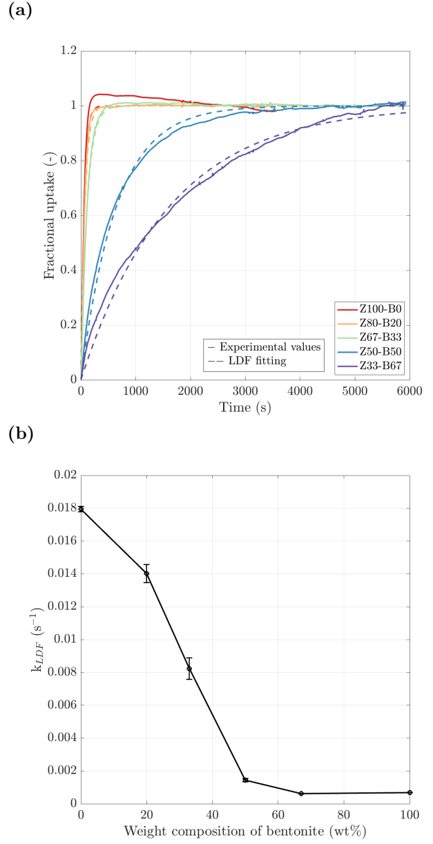
Figure 6: Quantitative and qualitative analysis of the kinetic tests carried out gravimetrically at F = 350 \text{ mL.min}^{-1} between p/p_0(\text{CO}_2) = 0.03 to 0.06 at 303 \text{ K} for Z100-B0, Z80-B20, Z67-B33, Z50-B50, Z33-B67: (a) Experimental normalised adsorption curves (solid line) with fitted adsorption curves (dashed line, LDF model); (b) Variation of k_{LDF} obtained from the LDF fit with bentonite content.
