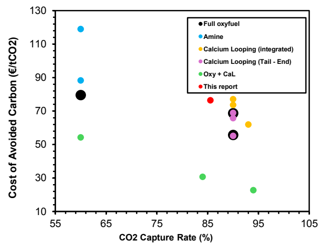
Figure 5 CAC and CO 2 capture rate of different CCS technologies [(Leeson et al., 2017), Gardarsdottir et al., 2019)]
