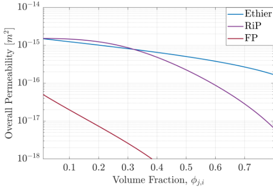
Figure 5. Log-linear plot of overall permeability functions against second component volume fraction, at constant fibrin permeability computed at a fibrin volume fraction of 0.01 using Davies' equation – Ethier's model (blue), RiP (purple), and FP (red) [21, 29-31].
