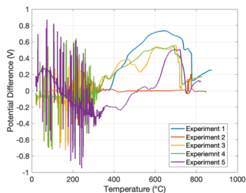
Figure 2. Open circuit potential difference of all experiments
