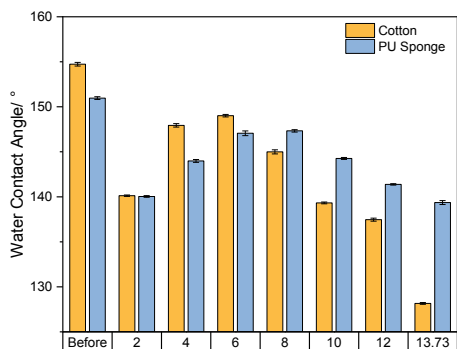
Figure 17. Water Contact Angle after pH tests
