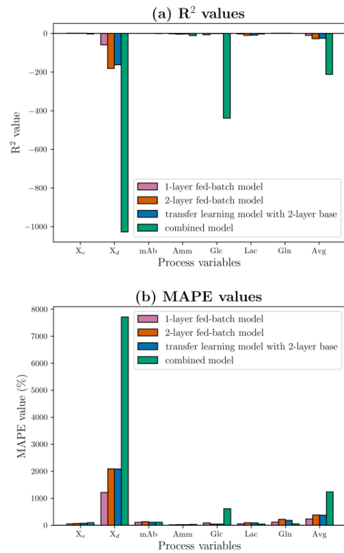
Fig. 9. Bar charts of metrics for continuous data predictions, broken down by process variable. (a) R^2 values. (b) MAPE values.
