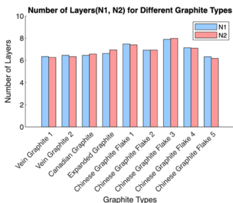
Figure 5 Number of layers (N1, N2) for different graphite types
