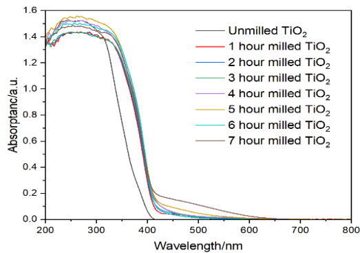
Figure 12: UV-Vis absorbance results of milled TiO 2 samples
