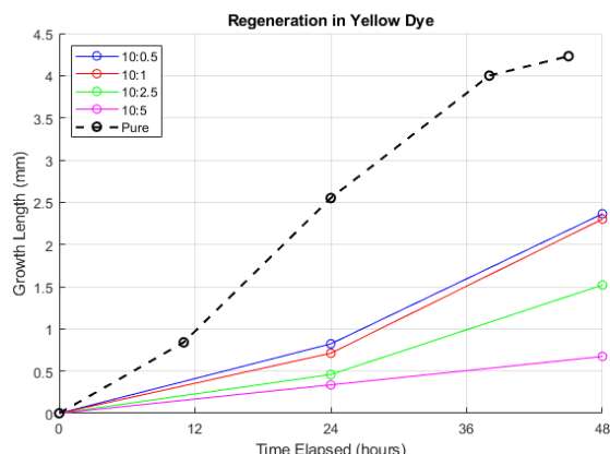
Figure 9 – Length grown against time plots for the regeneration of paracetamol crystals in volumetric ratios (ethanol to yellow food colouring) ranging from 10: 0.5 to 5
