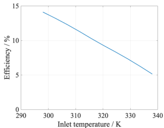
Figure 4.4. Effect of varied inlet temperature on bottom channel thermal efficiency. A rise in inlet temperature causes reductions in thermal and electrical efficiency.
