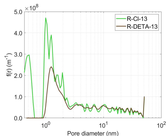
Figure 3: Effect of functionalisation on the micropore and mesopore region of the PSD of Resin 13
