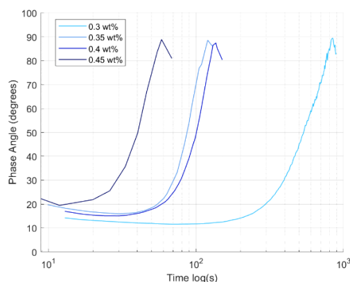
Figure 4.6 – Phase angle in degrees against a log time axis over the relaxation period for LUDOX TM-50 gels at different PEO concentrations.
