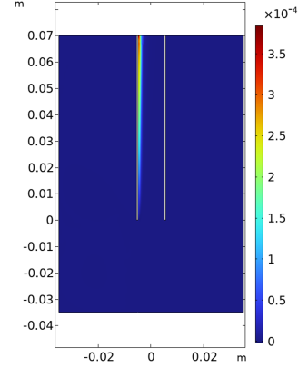
Figure 3: Hydrogen volume fraction in PEC with inlet flowrate of 500 ml/min
