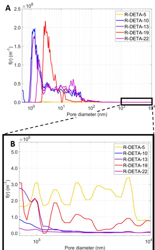
Figure 2: A) Overlapped complete PSDs for materials characterised with N_2 adsorption at 77K and MIP B) Overlapped PSDs magnified in the range 7 \times 10^2 to 1 \times 10^4 nm.
