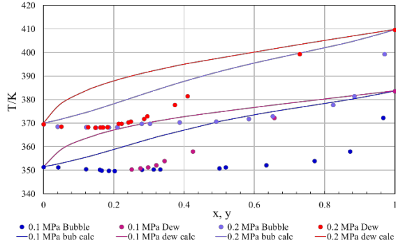
Figure 9 (b). Phase diagram of the toluene-ethanol mixture before parameters tuning
