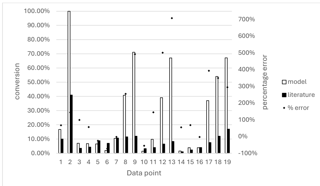
Figure 11. Comparison of reported CO 2 conversion and model simulated values, varied condition such as power, CO 2 fraction, pressure, total gas flowrate
