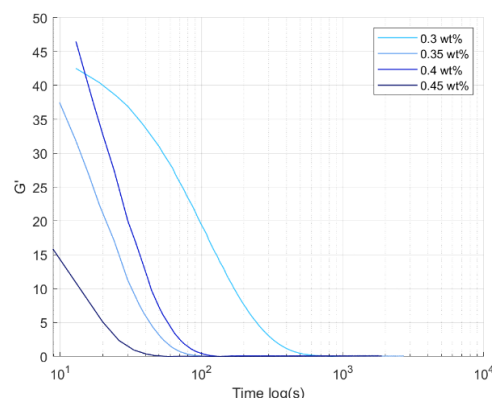
Figure 4.7 – Storage modulus against a log time axis over the relaxation period for LUDOX TM-50 gels at different PEO concentrations.
