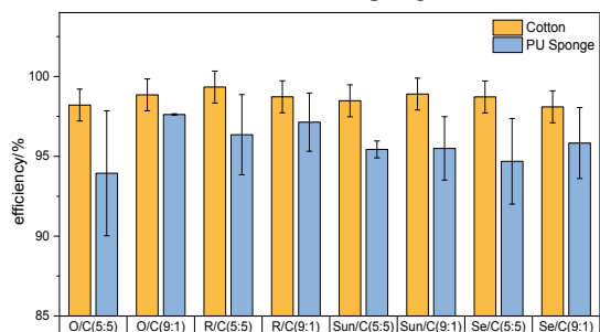
Figure 9. Oil-Water Separation of Vegetable Oil Mixed with Cyclohexane. O, C, R stand for olive oil, cyclohexane and rapeseed oil separately. Sun and Se stand for sunflower oil and sesame oil respectively
