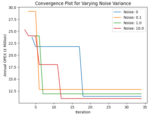
Figure 6: Annual Operational Expenditure (OPEX) convergence plot for Bayesian optimisation given different noise variance: 0, 0.1, 1.0, 10
