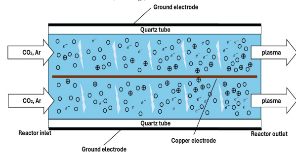
Figure 3. Illustration of 1-D plug-flow model, showing the plasma region, electric field and perpendicular flow direction. Another significant pathway for CO 2 dissociation is the energy exchange between vibrationally excited carbon
