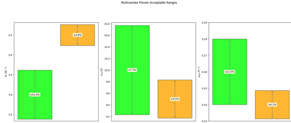
Figure 12: MPAR for each AOR found within the design space
