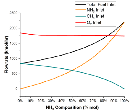
Figure 2. Flowrate of reactants for NH 3 scenarios
