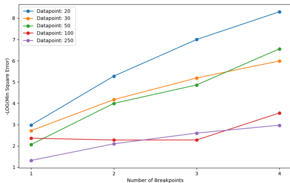
Figure 6: -\log(\text{MSE}) vs Breakpoints Across Datasets
