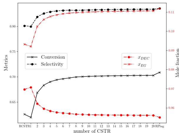
Figure 4.1.3: Conversion, Selectivity, DEC and EC Mole Fraction in increasing number of CSTRs in Series
