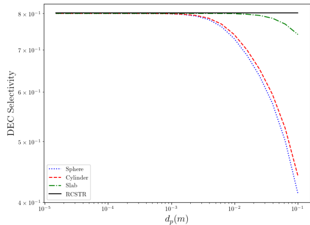
Figure 5.3.2: The relationship of the DEC selectivity on catalyst particle diameter and geometry, shown on a log-log scale
