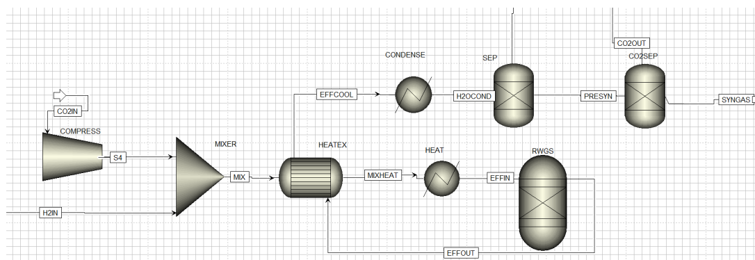
Figure 3.1: Aspen Flowsheet used for the whole process, excluding the FT reactor
