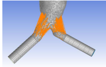
Figure 1.2 Image from ANSYS ICEM of the lower end of the AAA displaying the densities created for local refinement
