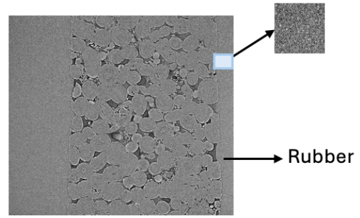
Figure 3. Slice of the raw images with dimensions of 2560 \times 2560 voxels 2
