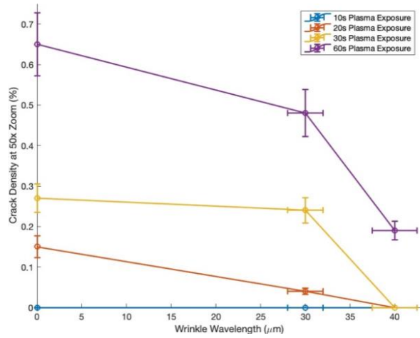
Figure 5: Impact of wrinkle wavelength (tens of \mu\text{m} ) on crack density after various plasma exposure times.
