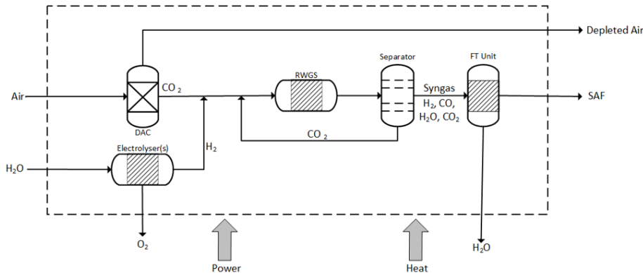
Figure 2.1: Simplified flow diagram for the overall SAF production process, self-made
