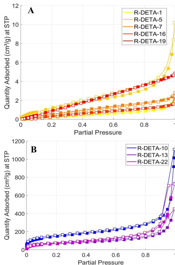
Figure 1: N 2 adsorption isotherms at 77K for materials with A) Type III isotherms and B) Type II isotherms. Filled marks/squares represent adsorption isotherm datapoints while hollow marks/squares represent desorption isotherm datapoints
