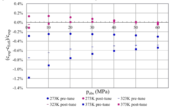
Figure 12 (a). Deviation of measured sound speed in toluene-cyclopentane mixture from the EoS predictions against absolute pressure before and after parameters tuning
