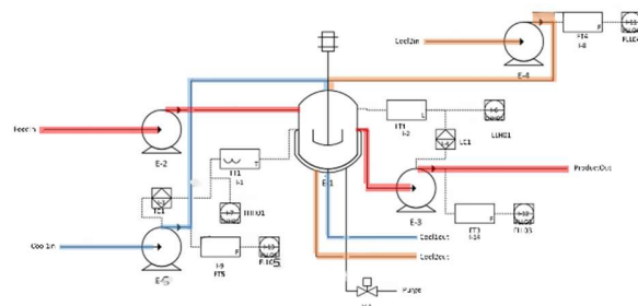
Figure 3.1 Mock P&ID Used in This Study
