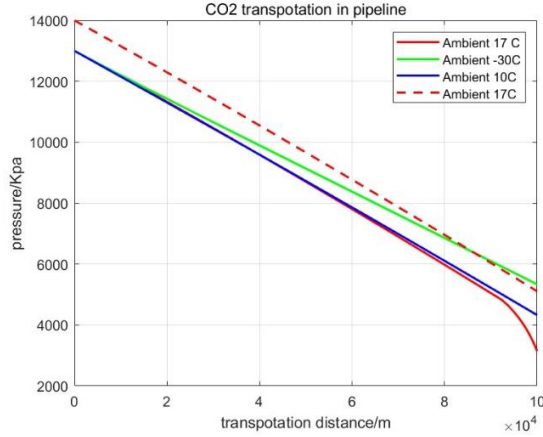
Figure 5 CO2 transportation simulation for different ambient conditions
