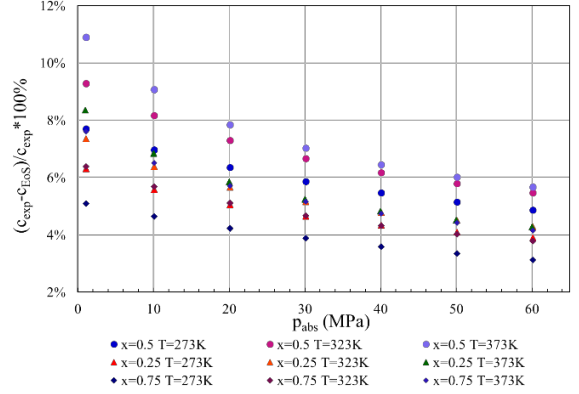
Figure 7. Deviation of measured sound speed in toluene-ethanol mixture from the EoS predictions against absolute pressure, x stands for the toluene composition
