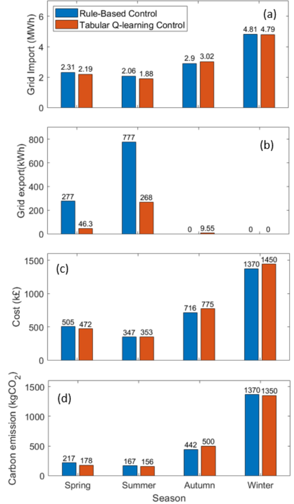
Figure 6: Results comparison between RBC and TQL during random two-day examples extracted from different seasons.
