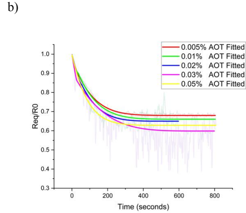
Figure 4 a) Drying curve of different surfactant concentrated samples x axis Req/R_0 is the equivalent particle radius normalised by its original radius. b) Drying curve fitted, first stage fitted with eqn_ as the first stage (pre skin formation), eqn_ as the second stage of drying (post skin formation).
