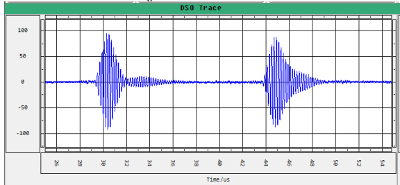
Figure 1 (a). Capture of the returning signals to the pulse-echo sensor
