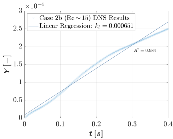
Figure 2: Linear regression plot to estimate k_l for case 2b with R^2 = 0.984 .
