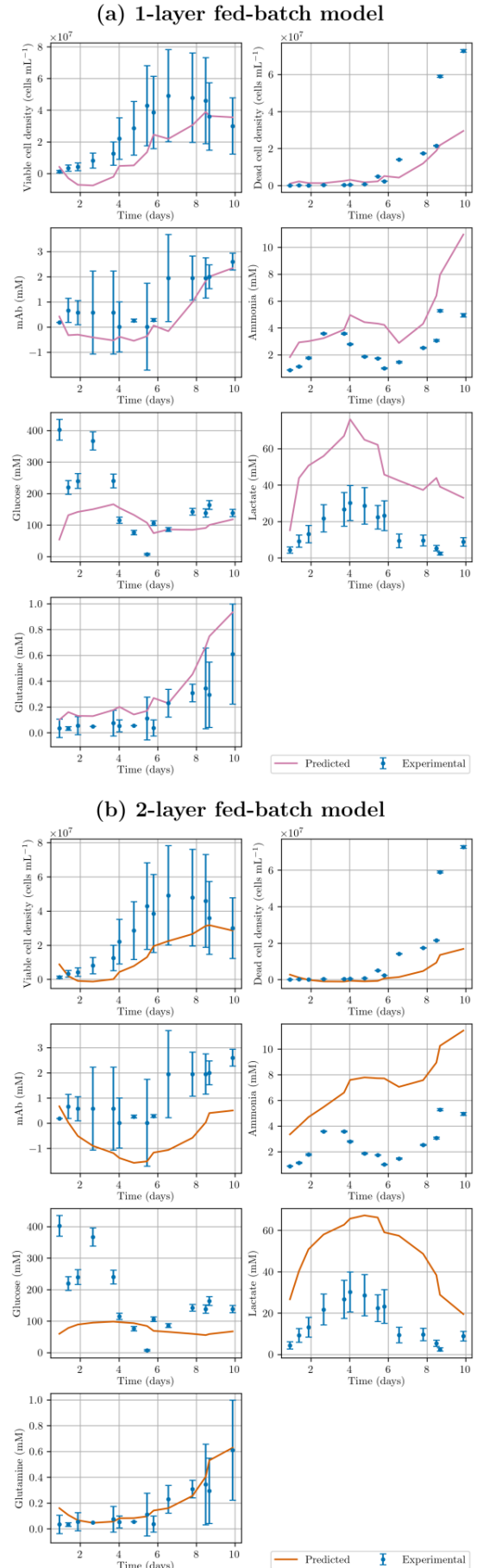
Fig. 4. Predictions of fed-batch data. (a) 1-layer fed-batch model. (b) 2-layer fed-batch model.
