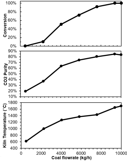
Figure 2 Effect of coal flowrate for calciner on conversion, CO 2 purity and kiln temperature.
