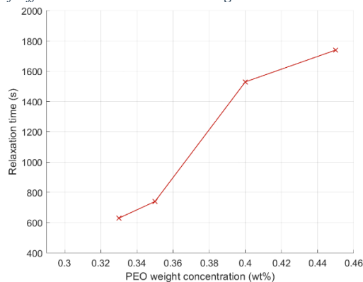
Figure 4.5 - Relaxation time (taken as time for viscosity gradient to reach zero) for CS50-28 gels compared with PEO concentration.
