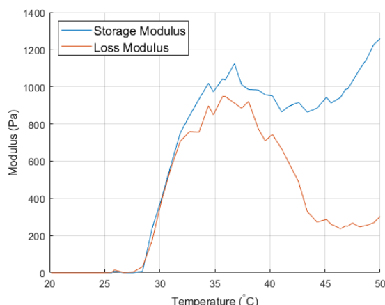
Figure 9. Storage and loss modulus of 18%w/v Pluronic hydrogel
