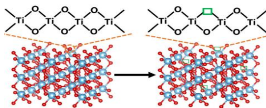
Figure 1: Oxygen Vacancy in TiO 2 nanostructure
