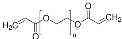
Figure 4: Molecular structure of PEGDA where n changes with molecular weight. PEGDA is susceptible to free radical polymerisation due to double bonds in acrylate groups at either end of molecule [20].
