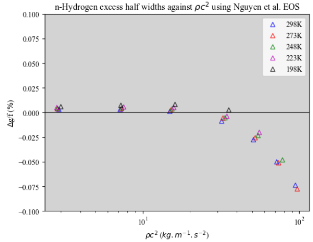
Figure 9: Excess half-widths of n-hydrogen data
