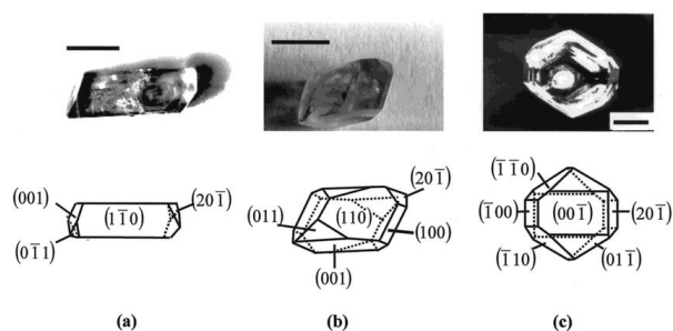
Figure 3 - Morphology of paracetamol crystals grown at (a) low, (b) medium and (c) high supersaturation. showing the observed forms of the crystals Source: [10]
