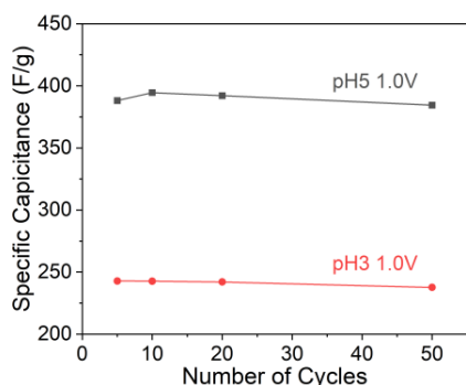
Figure 8. Specific capacitance of electro-deposited carbon paper under different pH over 50 cycles of charge-discharge.
