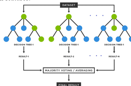
Figure 4 - 3 decision trees trained using bagging, with the final result obtained via the average of their individual outputs [31].
