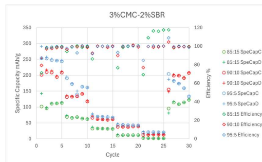
Figure 4.2-2: Cycle vs. Specific Capacity & Efficiency Graph for 3% CMC: 2% SBR
