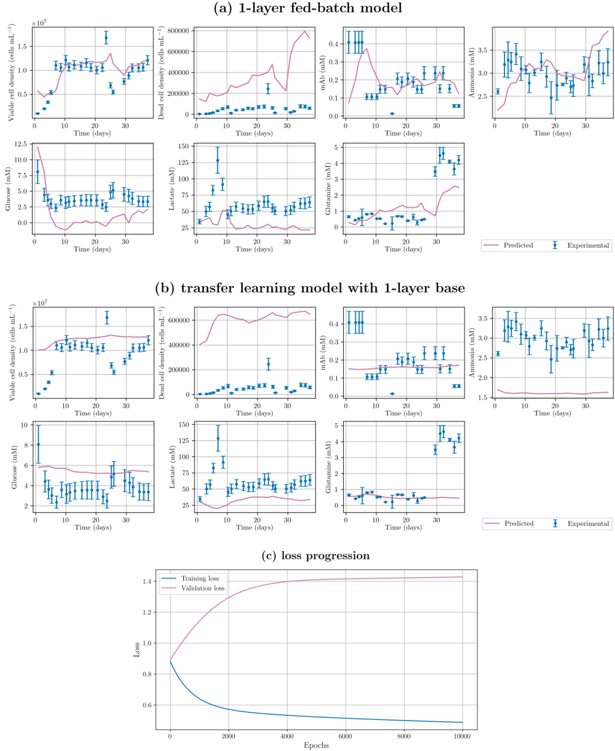
Fig. 6. Transfer learning using 1-layer model as base. (a) 1-layer fed-batch model predictions of continuous data. (b) Transfer learning model with 1-layer base predictions of continuous data. (c) Loss progression during transfer learning.
