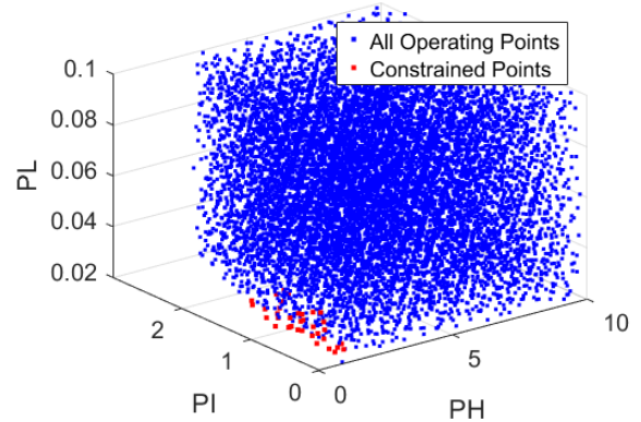
Figure 4. Z13X with 97% purity constraint imposed
