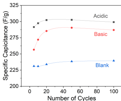
Figure 11. Specific capacitance of electrodeposited carbon paper with different pre-treatments over 100 cycles of charge-discharge.
