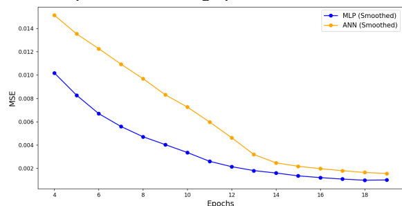
Figure 8: Mean squared error of modified MLP and ANN Across Epochs
