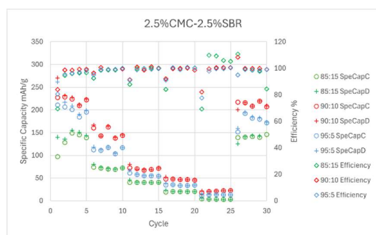
Figure 4.2-1: Cycle vs. Specific Capacity & Efficiency Graph for 2.5% CMC: 2.5% SBR
