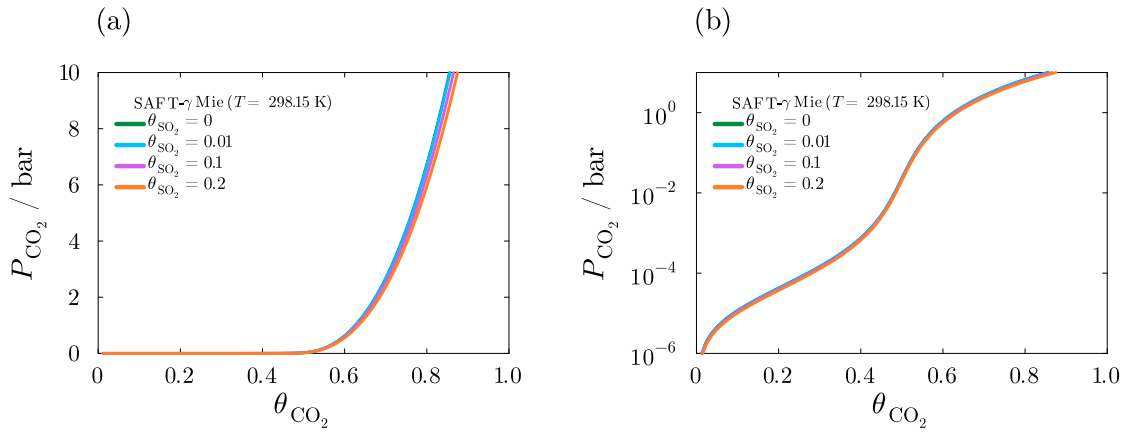
Figure 9: Predicted partial pressure of CO 2 at variable CO 2 loading in 30 w_{\text{MEA}} % solution, with lines of fixed \theta_{\text{SO}_2} . Linear plot (a), logarithmic plot (b).
