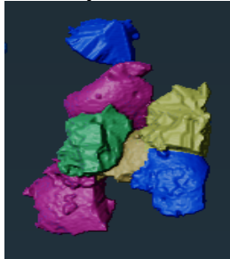
Figure 8. 3D volume rendering of the unfiltered sub volume of dimensions 500 \times 500 \times 500 \text{ voxels}^3 (height x width x depth)
