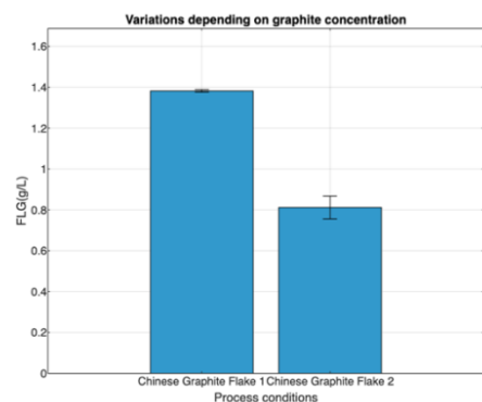
Figure 12 Variations of few-layer graphene concentration depending on graphite concentration (left: 100 g/L; right: 20 g/L).
