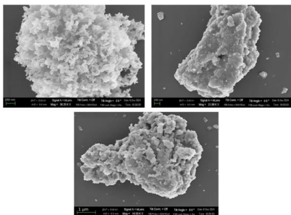
Figure 15: SEM images of unmilled (Left), 7 hour milled (Right) and 15 wt% doped TiO 2 samples (bottom)
