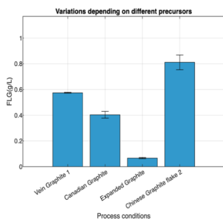
Figure 11 Variations of few-layer graphene concentration depending on precursors
