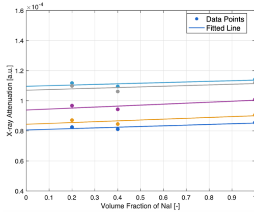
Figure 14. X-ray attenuation against volume fraction of NaI for 5 pore-sized rubber sub volumes plotted from Matlab
