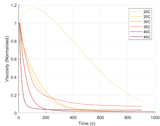
Figure 4.13 - Normalised viscosity against time of CS50-28 gel fixed at 0.35 wt% PEO concentration during relaxation at temperatures between 20-45°C.
