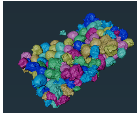
Figure 6. 3D volume rendering of the grains with dimensions 1401 \times 2018 \times 500 voxels 3 (width x height x depth)
