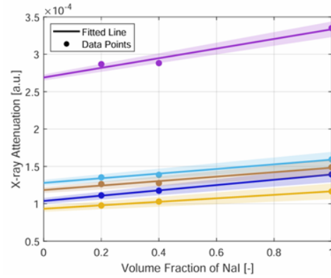
Figure 9. X-ray attenuation against volume fraction of NaI for 5 out of 136 grains plotted from Matlab
