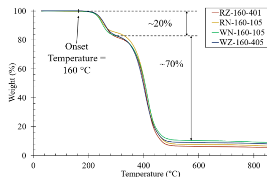
Figure 5 TGA plots over temperature range 30 - 850 °C.
