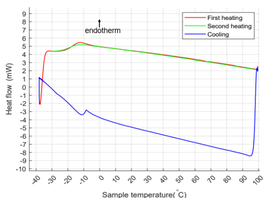
Figure 7 DSC heating and cooling curves for RZ-160-401 over the temperature range -37–100 °C.
