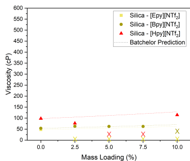
Figure 3.3.2: Viscosity (cP) against mass loading(%) trend for \text{SiO}_2 -[Epy][NTf 2 ], \text{SiO}_2 -[Bpy][NTf 2 ], \text{SiO}_2 -[Hpy][NTf 2 ] dispersions with comparison to theoretical predictions derived from the Batchelor equation
