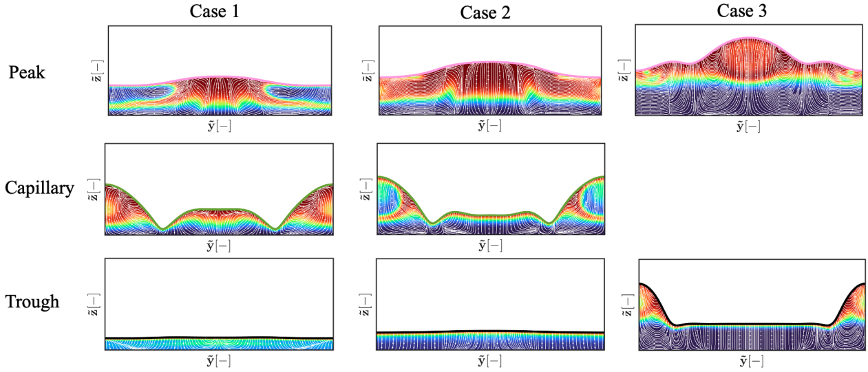
Figure 7: Spanwise slices of the concentration profile for the liquid film with streamlines at times t = 0.1s , t = 0.2s , and t = 0.35s respectively. Slices correspond to the main peak (pink), capillary waves (green), and trough (black) for (a) case 1, (b) case 2, and (c) case 3. Refer to the figure 6 for the full three-dimensional waves and plane locations.
