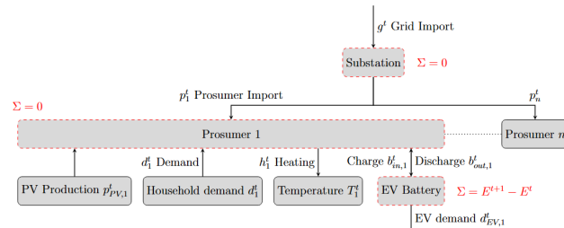
Figure 2: The energy environment model. Red dotted boxes represent energy balances.
