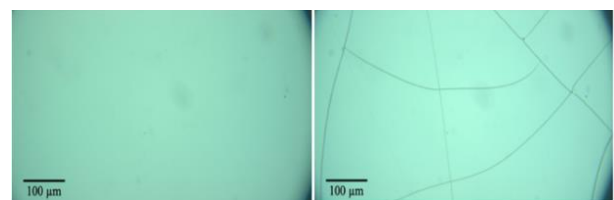
Figure 1: 50X image of plain PDMS before (left) and after (right) exposure to 60s of 99W plasma.
