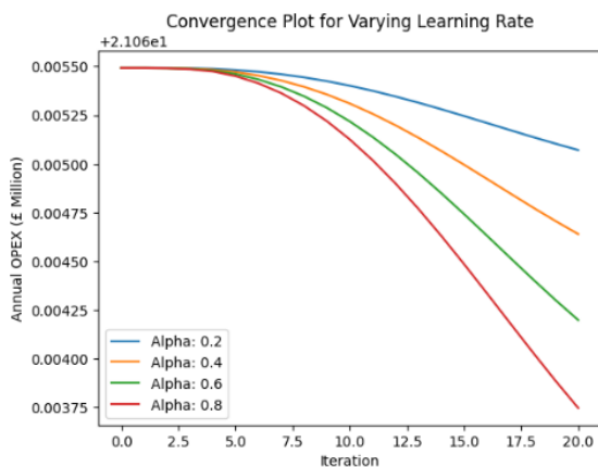
Figure 10: Annual Operational Expenditure (OPEX) convergence plot for Extremum Seeking Control given different learning rates
