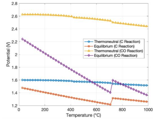
Figure 5. Modelled equilibrium potential and thermoneutral potential diagram
