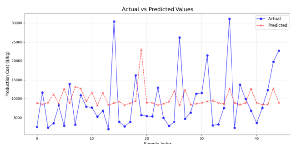
Figure 11- Actual vs. Predicted Production Cost using Random Forest.
