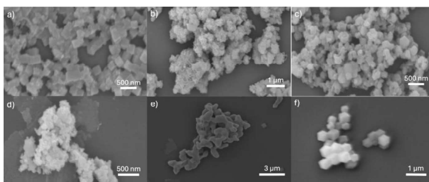
Fig. 7a-f: SEM of a) \text{CoP}_x ( \text{CoCl}_2 ), b) \text{CoP}_x ( \text{Co}_3\text{O}_4 ), c) \text{CoP}_x @C (ZIF-67), d) \text{CoP}_x (Co-Co-PBA NCs), e) \text{CoP}_x ( \text{Co}_3(\text{PO}_4)_2 ), f) ZIF-67.
