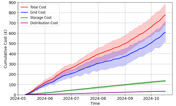
Figure 8: Heuristics mean cumulative costs for 10 prosumers.
