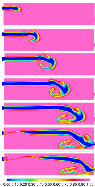
Fig. 9: Concentration maps for moving blood flow varying with time for a 1 mm mesh size and 0.01 s time-step.
