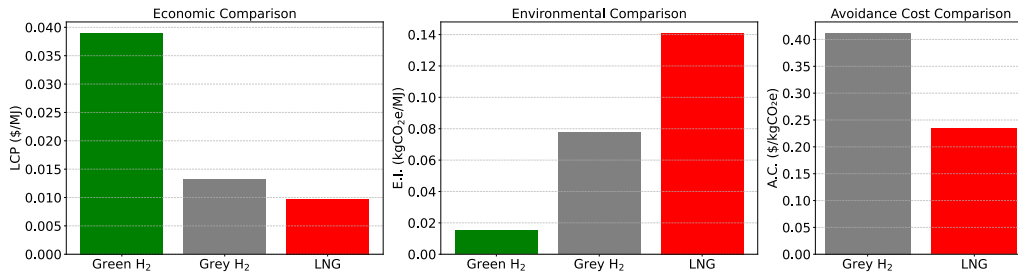
Figure 8. Comparison of Economic, Environmental, and Avoidance Costs for green hydrogen, grey hydrogen, and LNG. The avoidance costs are shown relative to green hydrogen. The graphs illustrate that whilst green hydrogen offers the greatest environmental benefits, it is the least cost-effective energy vector option.
