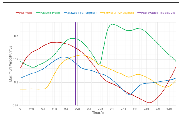
Figure 13.2 Plane 3 maximum velocity as a function of time between all 4 varying inlet boundary condition models
