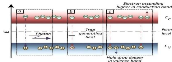
Figure 3: Radiative electron-hole recombination (Left), Shockley-Read-Hall recombination (Middle), Auger recombination (Right) [7]
