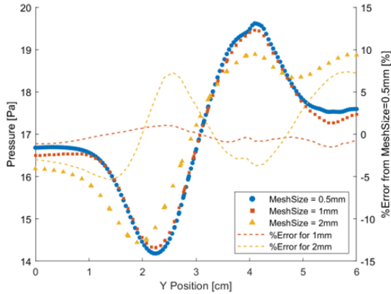
Figure 3: Pressure relationship graph with mesh size and associated error
