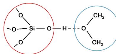
Figure 5.1 - Hydrogen bonding interaction between an isolated silanol group (circled red) and PEO oxygen (circled blue)
