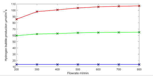
Figure 9: Hydrogen bubble production as a function of flowrate at different photocurrent densities. Blue: initial, Green: 5 times initial, Red: 10 times initial
