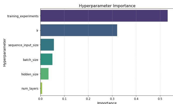
Figure 2: Forecasting Hyperparameter importance
