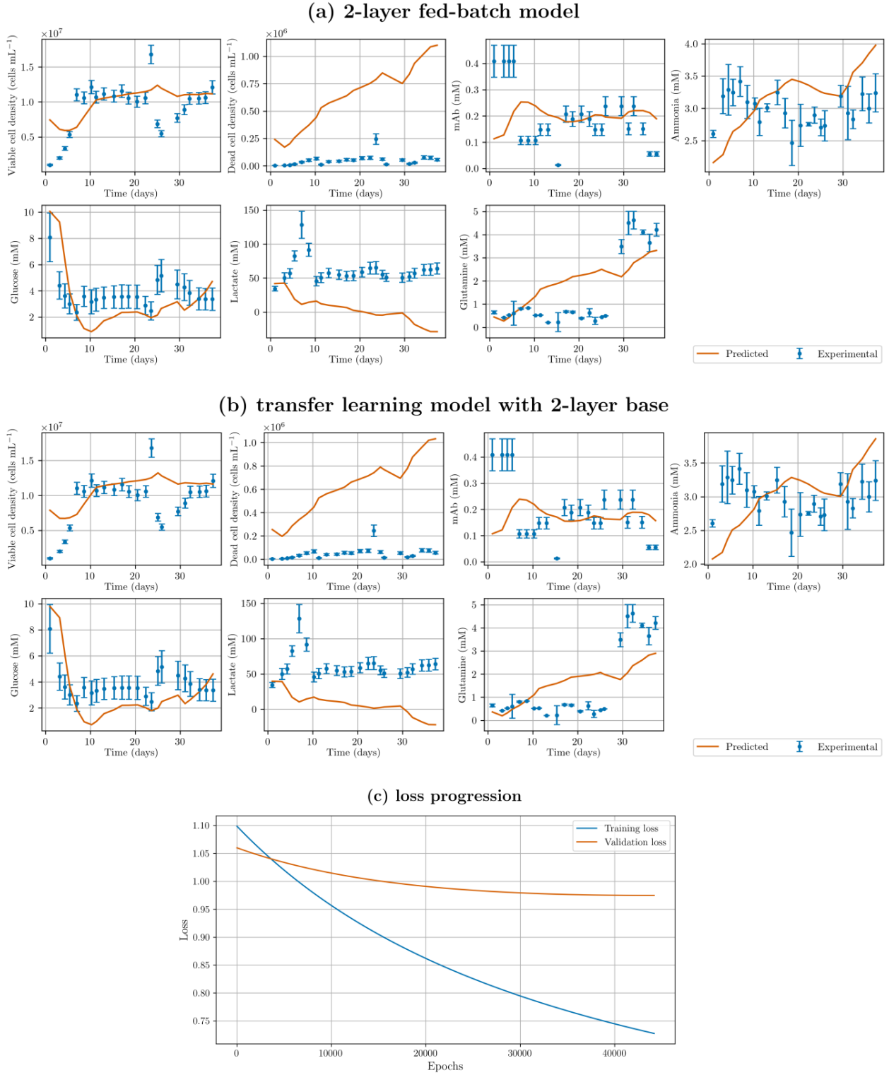
Fig. 7. Transfer learning approach using 2-layer model as base. (a) 2-layer fed-batch model predictions of continuous data. (b) Transfer learning model with 2-layer base predictions of continuous data. (c) Loss progression during transfer learning.
