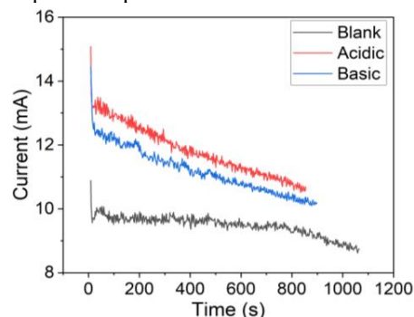
Figure 9. Electrodeposition current profile of the carbon paper under different pre-treatments, where Blank means no pre-treatment.
