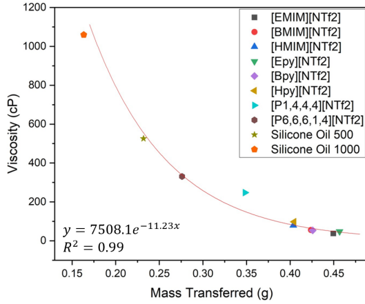
Figure 2.3.1: Calibration curve of neat ionic liquids with exponential fit curve equation
