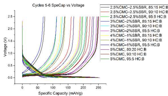
Figure 4.1-2: Specific Capacity vs. Voltage Graph for Cells of Different Composition from Cycle 5-6
