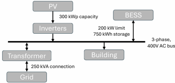
Figure 1: The system configuration of the examined store [11]
