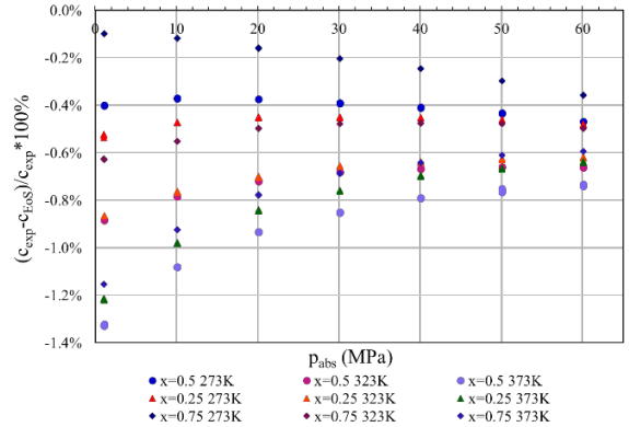
Figure 11. Deviation of measured sound speed in toluene-cyclopentane mixture from the EoS predictions against absolute pressure, x stands for the toluene composition
