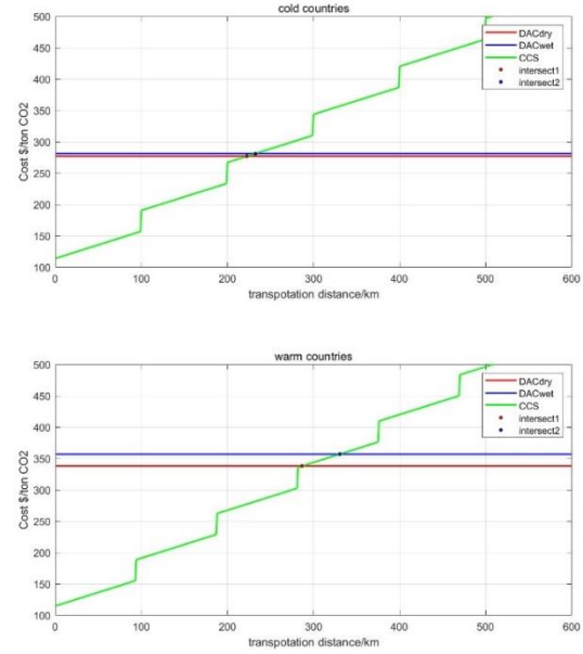
Figure 6 DAC-CCS comparison by transportation distance
