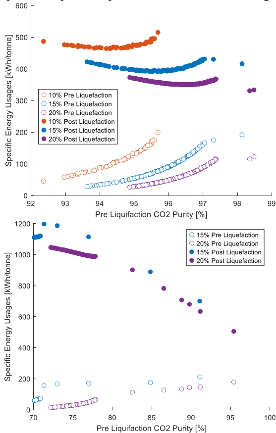
Figure 7. Z13X (top) and AC (bottom) SEN Pareto Fronts
