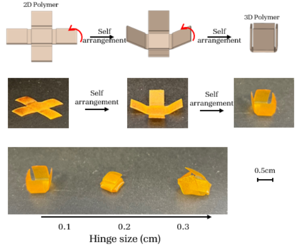
Figure 12: Self-assembly process of a 2D polymer into a 3D lidless box structure. The top panel illustrates the expected transformation from a flat 2D polymer sheet into a 3D cube structure via self-arrangement. The middle panel shows the actual sequential stages of self-arrangement for a 0.5 cm square side length and 0.1 cm hinge width structure. The bottom panel displays the resulting 3D structures at hinge sizes of 0.1 cm, 0.2 cm, and 0.3 cm, demonstrating the influence of hinge dimensions on the folding outcome. Scale bar: 0.5 cm.
