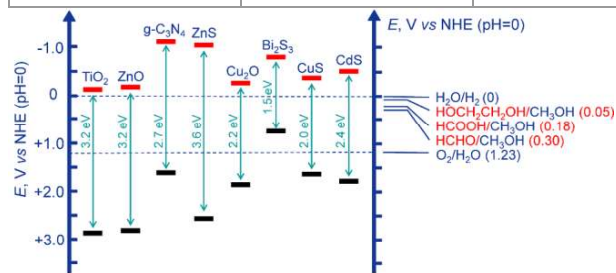
Fig. 2: Band gaps of commonly tested materials. 6
