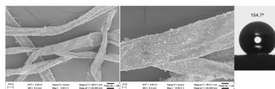
Figure 2. SEM Images of Modified Cotton
