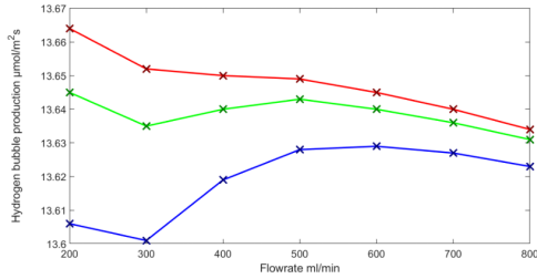
Figure 8: Hydrogen bubble production against flowrate for different bubble diameters
