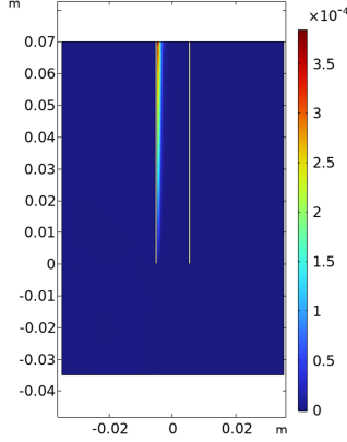
Figure 2: Velocity profile of the decoupled system with an inlet flowrate of 800 ml/min
