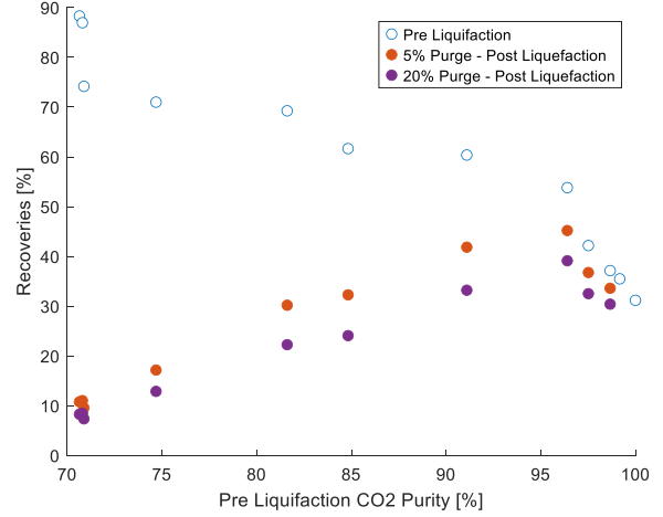
Figure 10. Z13X Recovery Pareto Fronts with varying Purge
