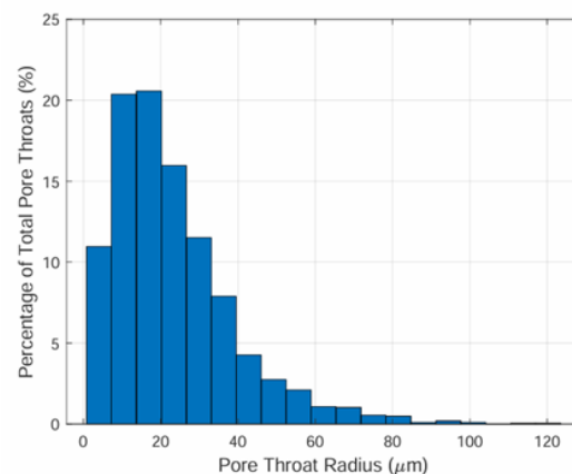
Figure 18. Histogram showing pore throat radii generated from the Pore Network Model function on Avizo.
