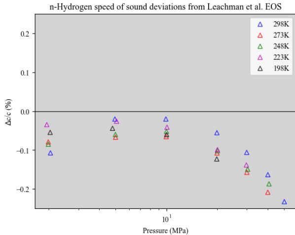
Figure 8: Deviations of n-hydrogen data from Leachman et al. [12]
