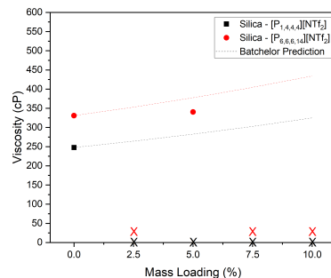
Figure 3.3.3: Viscosity (cP) against mass loading(%) trend for \text{SiO}_2 -[P 6,6,6,14 ][NTf 2 ], \text{SiO}_2 -[P 1,4,4,4 ][NTf 2 ] dispersions with comparison to theoretical predictions derived from the Batchelor equation
