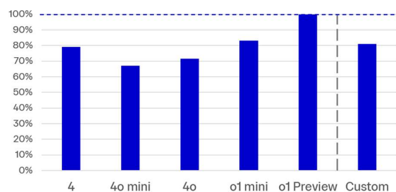
Figure 4.3.1 Average Performance Using Custom Mark Scheme
