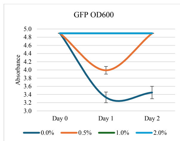
Figure 7. Line graph for GFP OD 600 absorbance during the induction period – again hidden concentrations are better seen in figure 8 .
