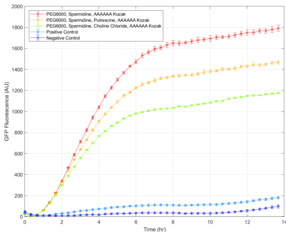
Figure 4.3.1 Fluorescence Over Time for RNA-Driven Translation with Different Kozak Sequences in a Cell-Free System
