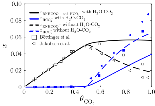
Figure 6: Predicted mole fractions of \text{NHCOO}^- and \text{HCO}_3^- in 30 w_{\text{MEA}}\% aqueous MEA at T = 293.15 K. Continuous lines indicate \text{CO}_2 - \text{H}_2\text{O} interaction, dashed lines indicate no \text{CO}_2 - \text{H}_2\text{O} interaction. Experimental data is depicted as square and triangular markers [41, 42], with filled markers indicating the data was used in parameter estimation.
