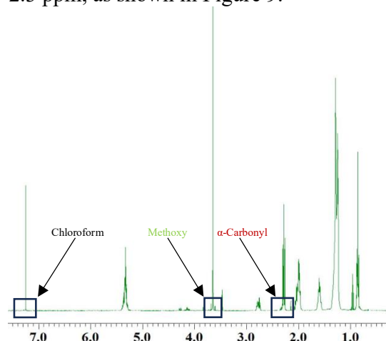
Figure 9: Proton NMR Spectrum Showing Relevant Peaks (Units of ppm).
