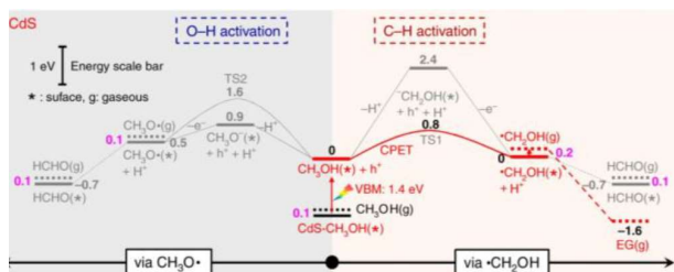
Fig. 1: MTEG reaction pathway over CdS proposed by Xie et al. 6
