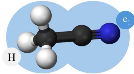
Figure 1. SAFT- \gamma Mie molecular model of acetonitrile including association sites. The model for acetonitrile comprises two identical segments decorated with two sites for like association – one of type H and another of type e_1 . The model is further discussed in Section 3.
