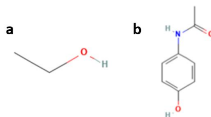
Figure 2 - structural formula of (a) ethanol and (b) paracetamol Sourced: [8] and [9]
