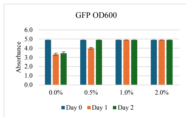
Figure 8. Bar chart representing the same GFP OD 600 data to better visualise absorbance over the entire experiment. Here, the 1% and 2% concentrations are clearly redundant towards any conclusion.
