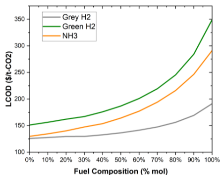
Figure 7. LCOD for all scenarios
