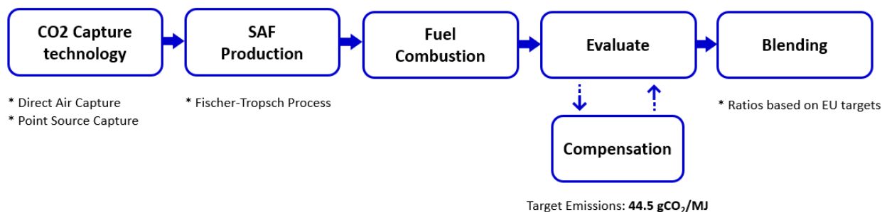
Figure 3 – Overview of SAF emission pathway
