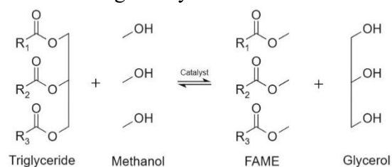
Figure 2: Methanolysis of Triglycerides. Adapted from Meher et al. (2006).
