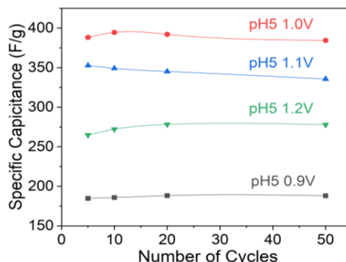
Figure 4. Specific capacitance of electro-deposited carbon paper under different applied potentials over 50 cycles of charge-discharge.
