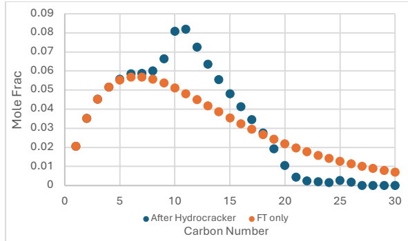
Figure 4.1: Product distribution of stream after FT and Hydrocracker
