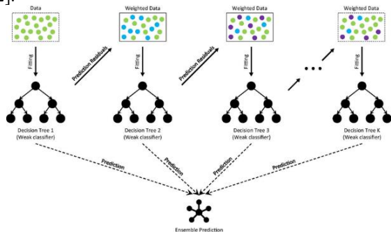
Figure 5 - Iterative Refinement for Enhanced Prediction Accuracy
