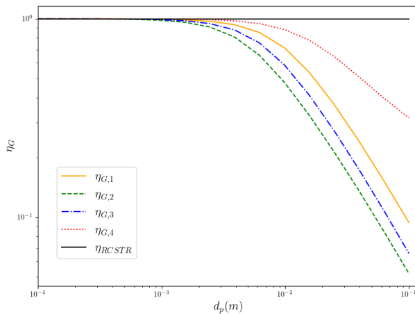
Figure 5.2.1: The relationship of the global effectiveness factor of four reactions on catalyst particle diameter, shown on a log-log scale
