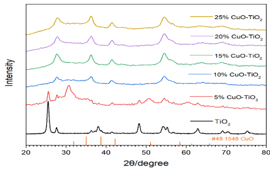
Figure 11: XRD results of CuO doped TiO 2 samples
