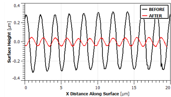
Figure 7: Graphical presentation of the cross-sectional area of a wrinkled surface before and after 10 second exposure time to plasma
