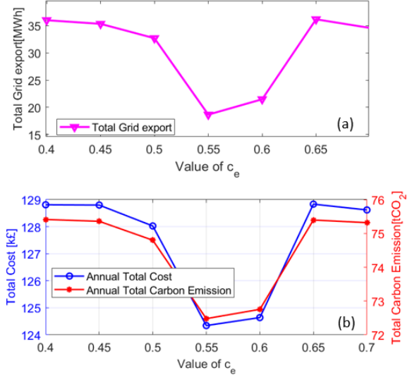
Figure 8: Sensitivity analysis of export penalty c_e , with a fixed cost coefficient w_1 of 80, trained through 1000 episodes with minimum epsilon \epsilon_{min} of 0.01
