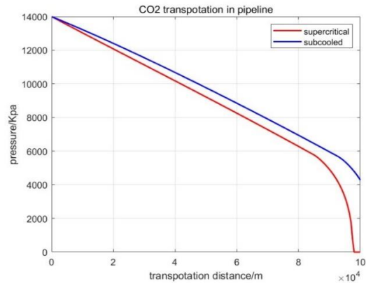
Figure 4 CO2 transportation via pipeline (Supercritical & subcooled)
