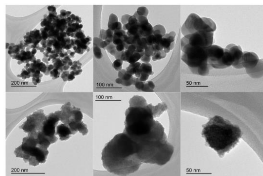
Figure 11. TEM images of ZrO 2 (top row) and H 2 SO 4 -treated ZrO 2 (bottom row) at 200, 100, 50 nm magnifications.
