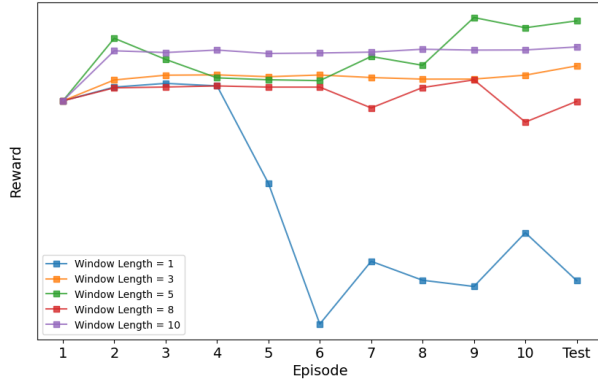
Figure 5: Learning curves for varying window lengths. Rewards are normalised to the same starting values.
