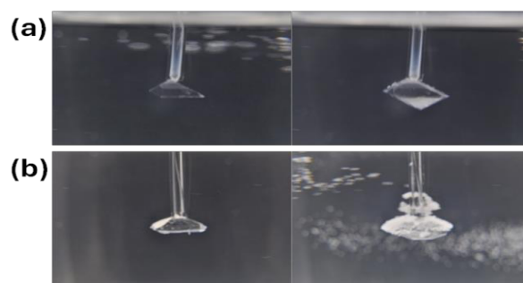
Figure 7 - Photos displaying extents of secondary nucleation at different agitation speeds of (a) 150 rpm, and (b) 200 rpm. Photos at time 0 hours and (a) 19.5 hours, (b) 30 hours.
