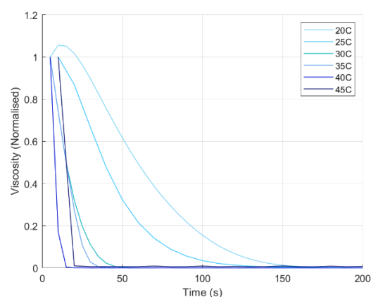
Figure 4.12 – Normalised viscosity against time of LUDOX TM-50 gel fixed at 0.35 wt% PEO concentration during relaxation at temperatures between 20-45°C.
