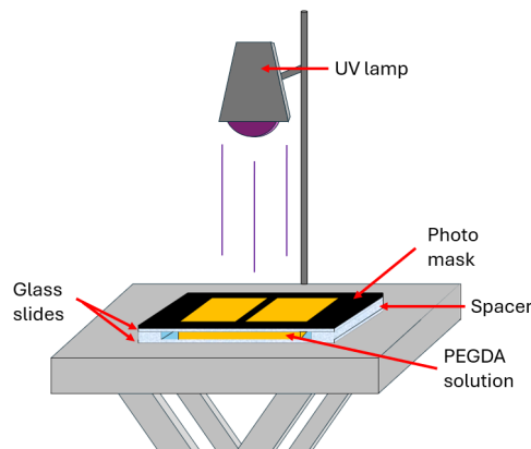
Figure 2: Experimental setup for the FPP standard fabrication procedure. The setup includes glass slides separated by spacers, with PEGDA solution forming a capillary in between the slides. The photomask controls regions of UV light exposure.
