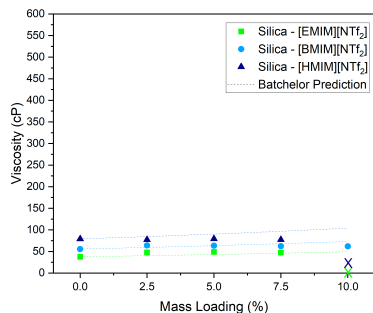
Figure 3.3.1: Viscosity (cP) against mass loading(%) trend for \text{SiO}_2 -[EMIM][NTf 2 ], \text{SiO}_2 -[BMIM][NTf 2 ], \text{SiO}_2 -[HMIM][NTf 2 ] dispersions with comparison to theoretical predictions derived from the Batchelor equation
