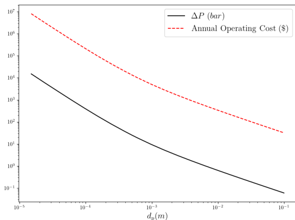
Figure 5.4.1: The relationship of Pressure Drop and Annual Operating Cost on catalyst particle diameter, shown in log-log scale
