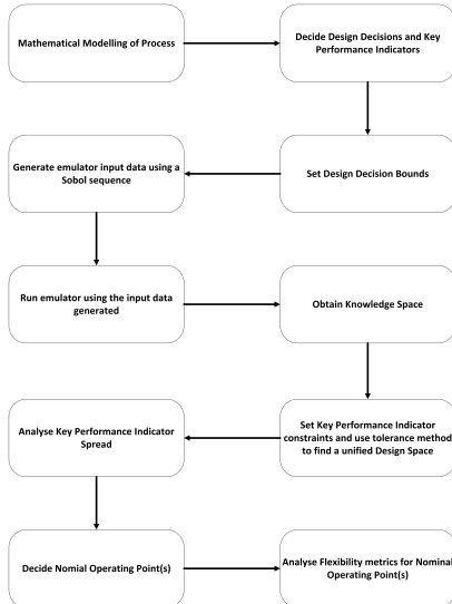
Figure 5: Computational framework for DSP identification and analysis, adapted from [7]. The workflow begins with mathematical modelling of the process, proceeds through selecting DDs and KPIs and, finishes in identifying robust and flexible operating points.
