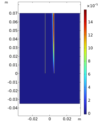
Figure 4: Oxygen volume fraction in PEC with inlet flowrate of 500 ml/min
