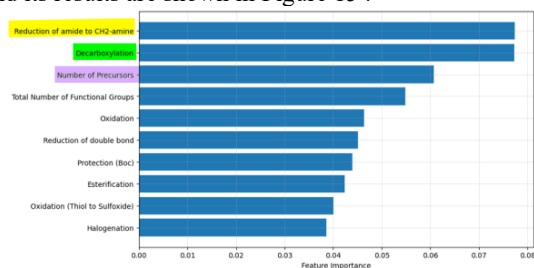
Figure 15 - Re-calculated Top 10 features of XGBoost
