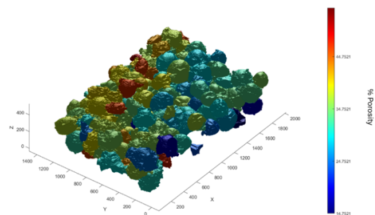
Figure 12. 3D volume rendering of the grains of dimension 1401 x 2018 x 500 (width x height x depth). The colourmap indicates each grain microporosity value
