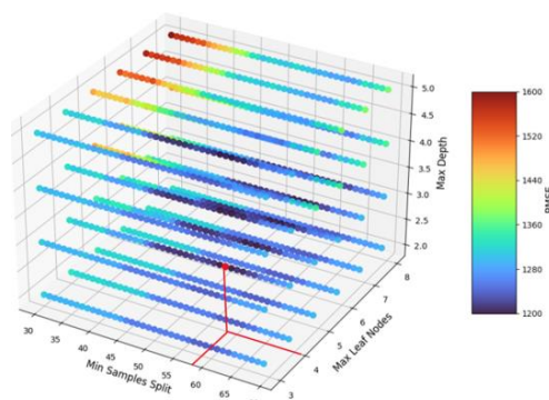
Figure 10 - 3D Heat Map of min_samples_split , max_leaf_nodes , and max_depth , with a RMSE Scale for RF
