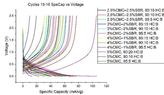
Figure 4.1-4: Specific Capacity vs. Voltage Graph for Cells of Different Composition from Cycle 15-16
