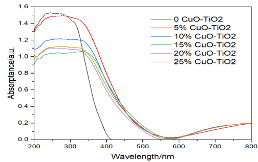
Figure 13: UV-Vis absorbance results of doped TiO 2 samples
