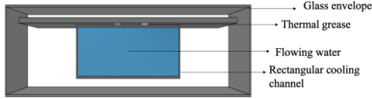
Figure 1.4 Schematic diagram of the bottom channel
