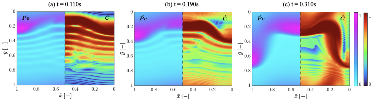
Figure 4: Contours of normalised local mass Peclet number, \hat{P}_e (left half-plane) and normalised local \text{CO}_2 concentration, \hat{C} (right half-plane) for a) case 1a, b) case 2a, and c) case 3a, for normalised global concentration of \text{CO}_2 in liquid film at \sim 0.2 .
