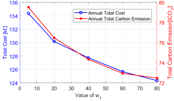
Figure 7: Sensitivity analysis of cost coefficient of reward function w_1 , with fixed export penalty c_e of 0.55, trained through 1000 episodes with a minimum epsilon \epsilon_{min} of 0.01
