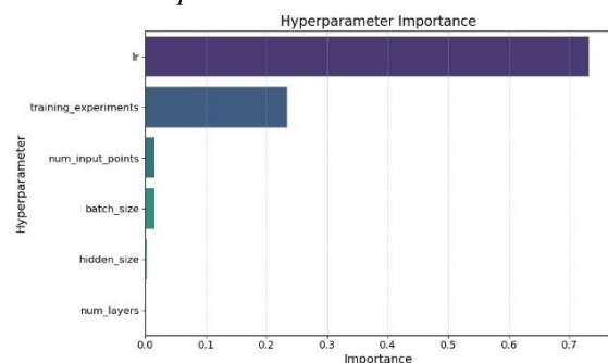
Figure 3: Interpolation Hyperparameter importance
