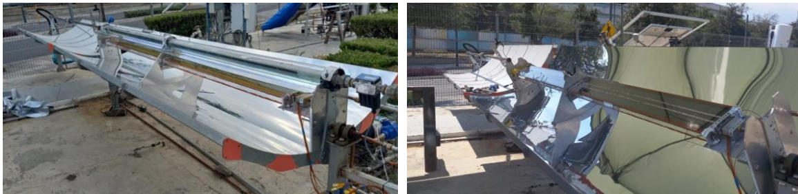
Figures A.1 and A.2 Experimental setup of collector in Mexico
