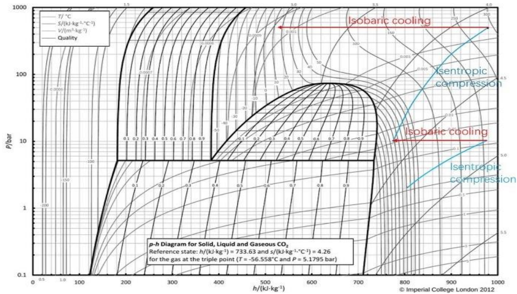
Figure 3 CO2 h-p plot and compression pathway
