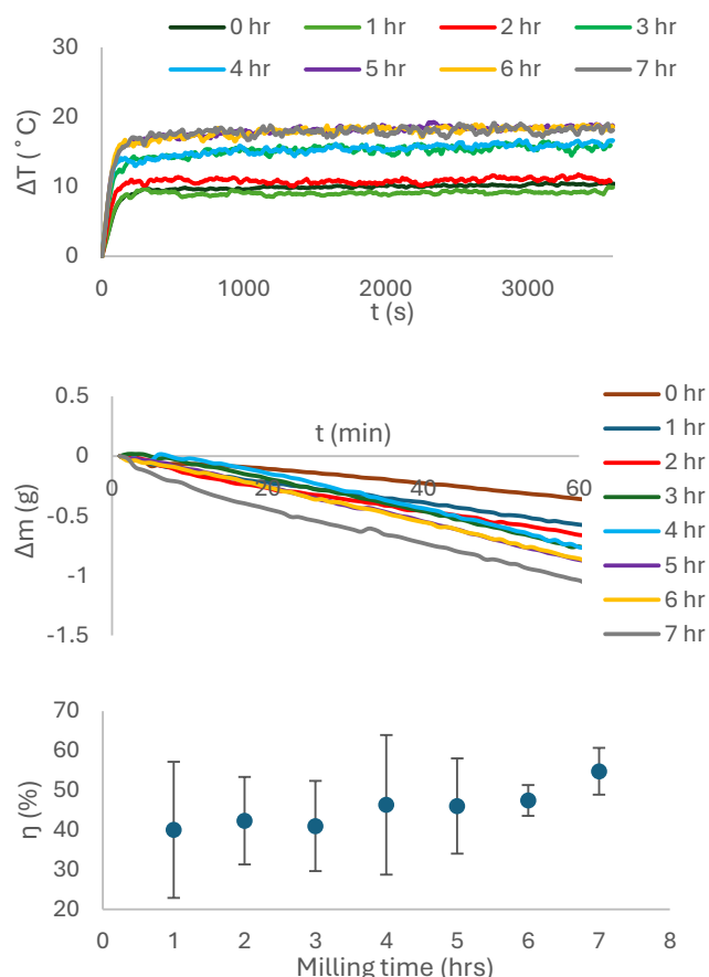
Figure 8: Temperature change (Top), Mass change (Middle), Photothermal efficiency (Bottom) for each milling time
