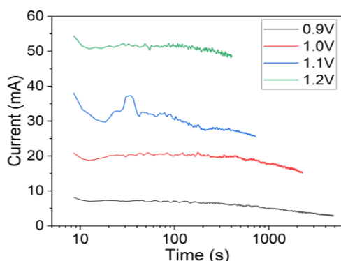
Figure 3. Electrodeposition current profiles at pH 5 under different applied potentials on carbon paper.
