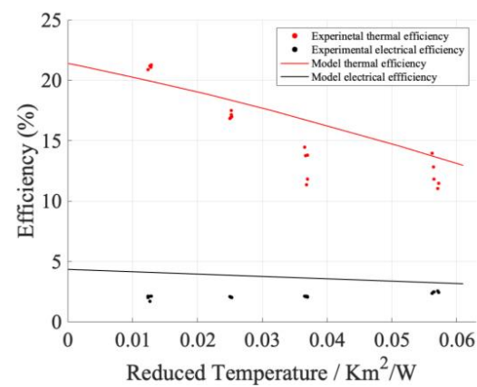
Figure 4.5. Validation of top channel model using experimental data. As reduced temperature increases, thermal and electrical efficiency both decrease.
