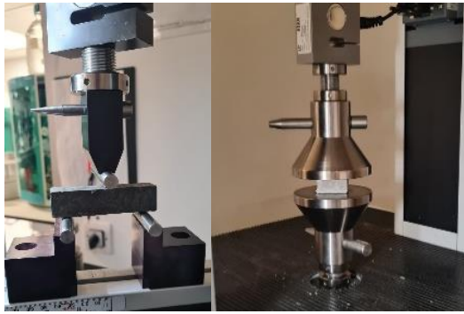
Figure 1. Different Configurations of EZ 50
