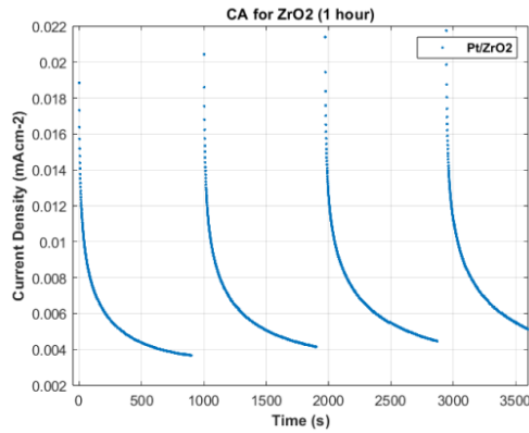
Figure 4. CA curves of Pt-based ZrO 2 catalyst over repeated 15-minute cycles for 1 hour.
