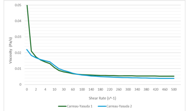
Figure 4 Viscosity as a function of shear rate from 0–500 s -1 (range of shear rate in healthy arterial systems) [24] for Carreau-Yasuda 1 & 2
