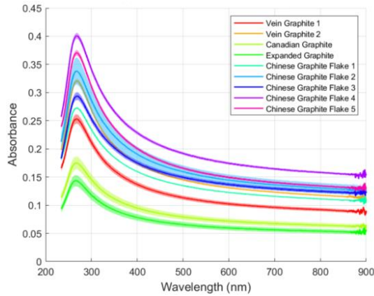
Figure 4 Absorbance intensity spectra for all processed samples including individual standard error
