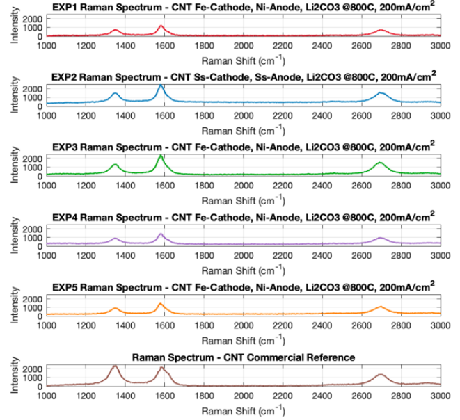
Figure 6. Raman spectra of all conducted experiments
