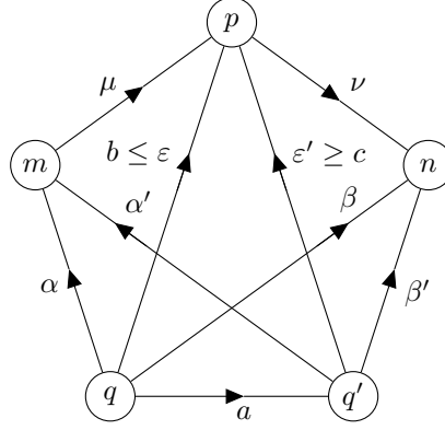
FIGURE 6. Points m, n, p, q, q' \in N' .
