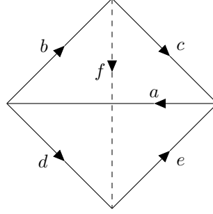
FIGURE 2. The atoms a, b, c, d, e .
