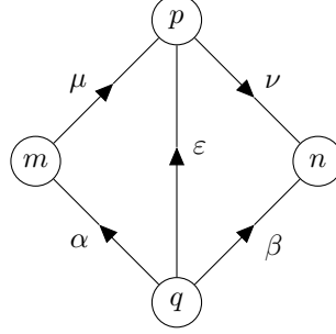
FIGURE 4. Points m, n, p, q \in N' .
