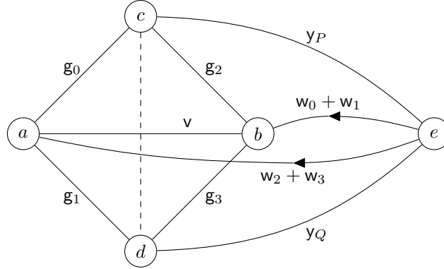
FIGURE 3. Points a, b, c, d, e \in M .
