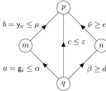
FIGURE 5. Atoms a, b, c, d, e .
