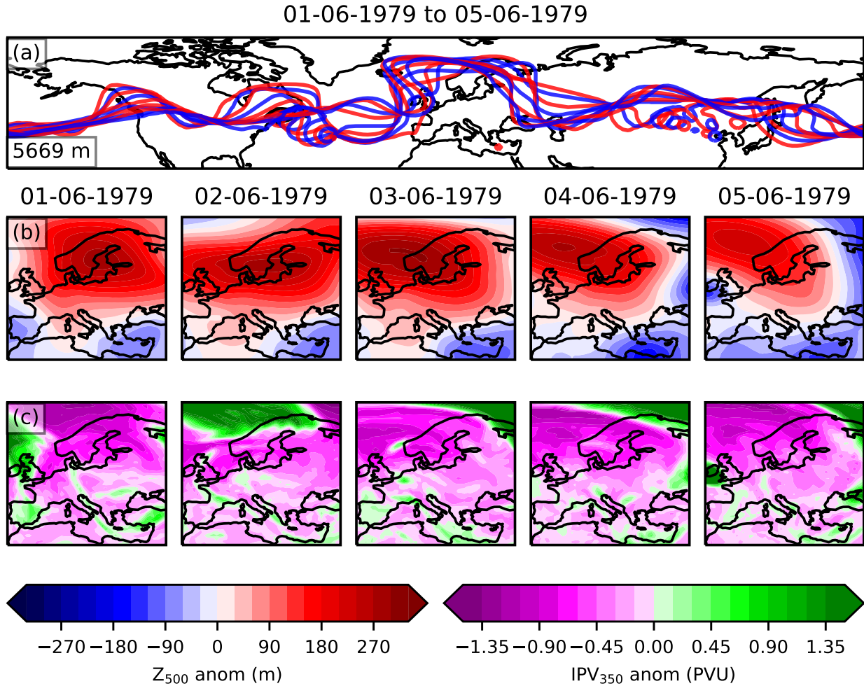
Figure 1. The information used to classify blocks in the ERA5 ground truth dataset (GTD). (a) shows the Z_{500} contour for the averaged value across 30–70 °N, indicated in the bottom left of the panel. The red and blue colours highlight the contours at midnight and midday respectively. (b) and (c) show the Z_{500} time detrended anomaly and IPV 350 anomaly for each day.
