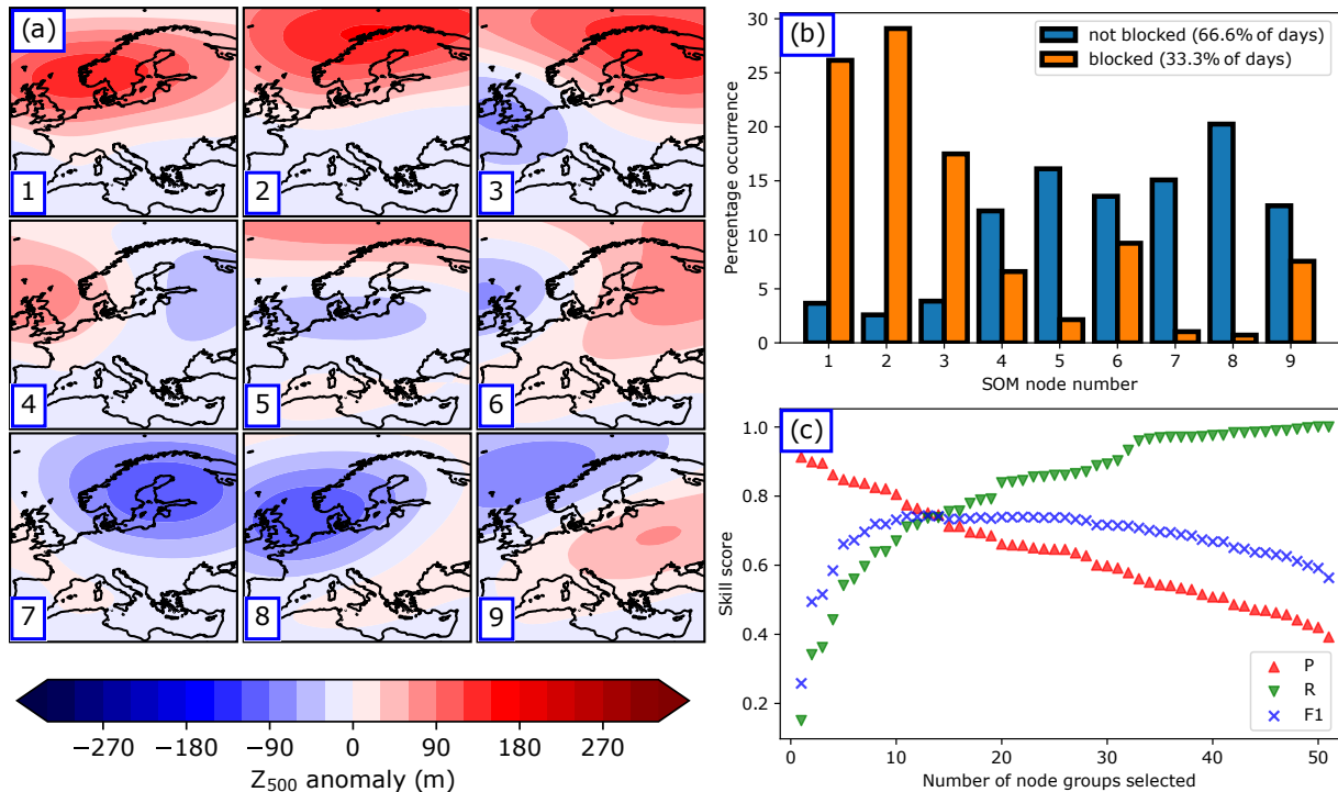
Figure 4. The SOM blocking index (SOM-BI). (a) The trained 3x3 SOM for Z_{500} time detrended anomaly. (b) Normalised histograms showing the distributions of occurrence of BMUs for the days identified as blocked or non-blocked within the GTD. (c) The SOM-BI optimisation of the set of node groups against three different skill scores (precision (P), recall (R) and F1 score) that are associated with the GTD blocking events.
